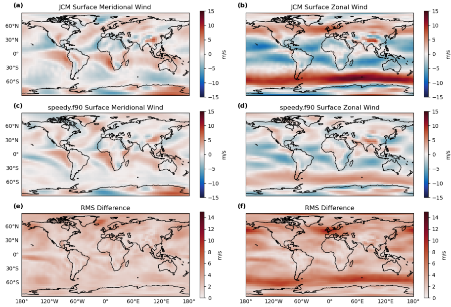
Figure 3. Average meridional and zonal winds in the surface layer in JCM (a and b) and in speedy.f90 (c and d). The RMS difference between the two simulations is shown in panels (e) and (f).
