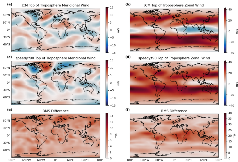
Figure 4. Average meridional and zonal winds at the top of the troposphere in JCM (a and b) and in speedy.f90 (c and d). The top of the troposphere, as defined by the SPEEDY model, is the third sigma layer from the top of the atmosphere. The RMS difference between the two simulations is shown in panels (e) and (f).
