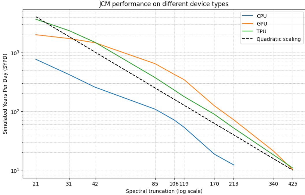
Figure 6. Model performance on different hardware for a default JCM run, 30 minute timestep. To generate this plot, runs of 1 simulated year were conducted on 3 types of Google Cloud virtual machines: a CPU VM (with 32x Intel Xeon Platinum 8581C), a GPU VM (with a 16GB Tesla P100 PCIe), and a TPU VM (with a Google Cloud TPU v5 lite). These devices were chosen as comparable based on having similar pricing (approx. $1.50 / hour) at time of writing.
