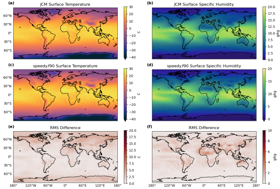
Figure 2. Average surface temperature and surface specific humidity in the surface layer in JCM (a and b) and in speedy.f90 (c and d). The root-mean-square (RMS) difference between the two simulations is shown in panels (e) and (f).
