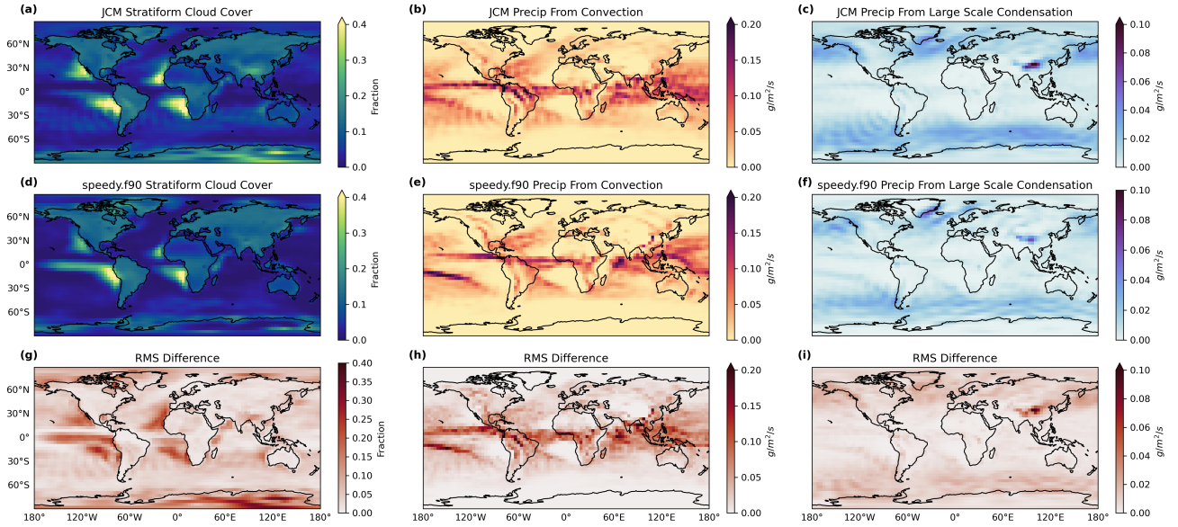
Figure 5. Average stratiform cloud cover (a and d), precipitation due to convection (b and e), and precipitation due to large scale condensation (c and f). RMS difference between JCM and speedy.f90 is shown in panels (g)-(i)
