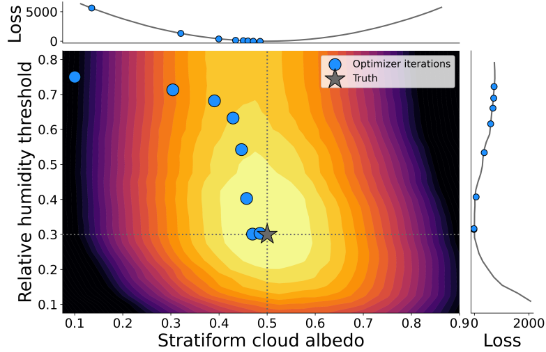
Figure 7. Loss versus Visualisation of the 2-D loss landscape for the described parameter estimation example. The optimization begins with values of 0.1 for stratiform cloud albedo and 0.75 for relative humidity threshold. The orange-optimal value is successfully found near the true SPEEDY values of 0.5 and 0.3, respectively. Blue dots show the calculated loss at each iteration of gradient descent, and the yellow grey star is the “true” value. Curves at the top and right sides of the contour plot show slices of the loss function obtained by varying the parameters independently.
