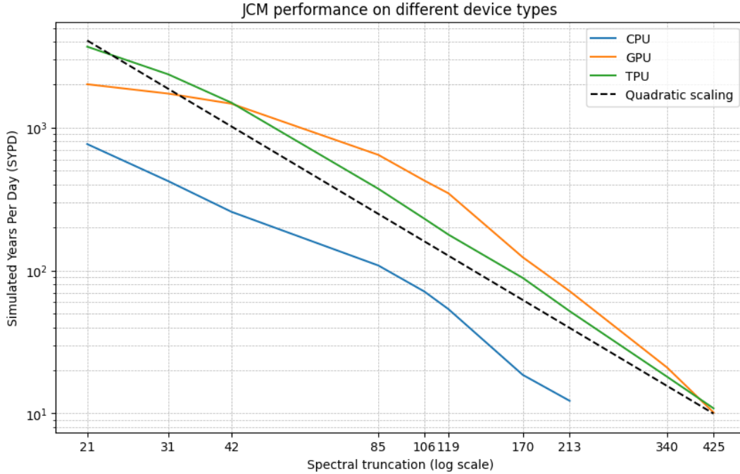
Figure 6. Model runtimes performance on different hardware for a default JCM run, 30 minute timestep. To generate this plot, runs of 1 simulated year were conducted on 3 types of Google Cloud virtual machines: a CPU VM (with 32x Intel Xeon Platinum 8581C), a GPU VM (with a 16GB Tesla P100 PCIe), and a TPU VM (with a Google Cloud TPU v5 lite). These devices were chosen as comparable based on having similar pricing (approx. $1.50 / hour) at time of writing.
