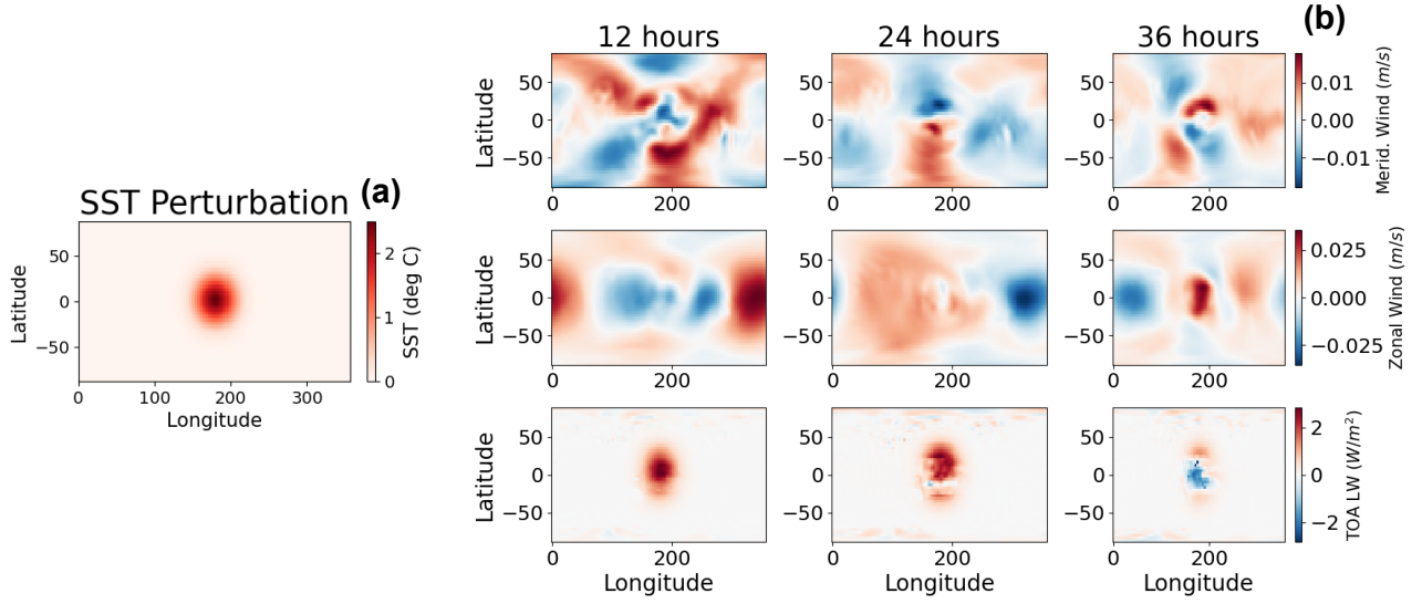
Figure 8. Influence of a sea surface temperature (SST) perturbation on the future model state. (a) Sea surface temperature (SST) perturbation in ^{\circ}\text{C} . (b) Changes to meridional wind (row 1), zonal wind (row 2), and outgoing longwave radiation at the top of the atmosphere (row 3) at 12 hours (column 1), 24 hours (column 2), and 36 hours (column 3) in the future.
