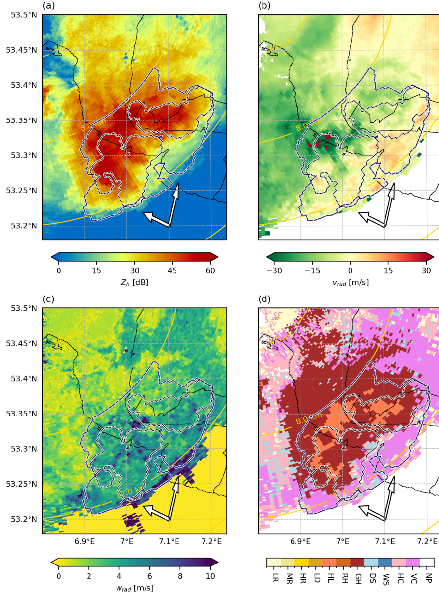
Figure 10. Top view of radar images at an elevation angle of 17^\circ , around convective system A, at the time of the LOFAR image at 19:17:37 UTC with: (a) reflectivity Z_h , (b) radial velocity V_{rad} , (c) radial velocity spectrum width W_{rad} , (d) the Hydrometeor Classification Algorithm HMC. The radar resolution volumes within 2 km of sparkles (black dotted) and other VHF sources (blue dashed) are indicated by contours. Arrows indicate cloud edges with high W_{rad} values. Yellow arcs indicate the 8 and 12 km altitude of the radar data.
