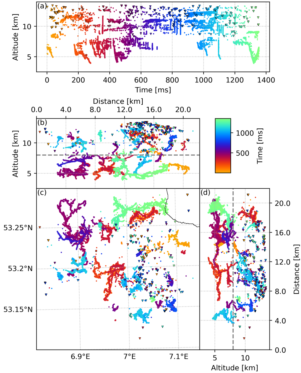
Figure S3.3. Similar to Fig. S3.1, but part of the LOFAR image at 19:19:54, and focusing on convective system B. The horizontal extent of panel (c) matches with Fig. 1. The VHF sources with a point shape and black contour are marked as sparkles by the two-stage clustering process, but fall below the 8 km altitude threshold.
