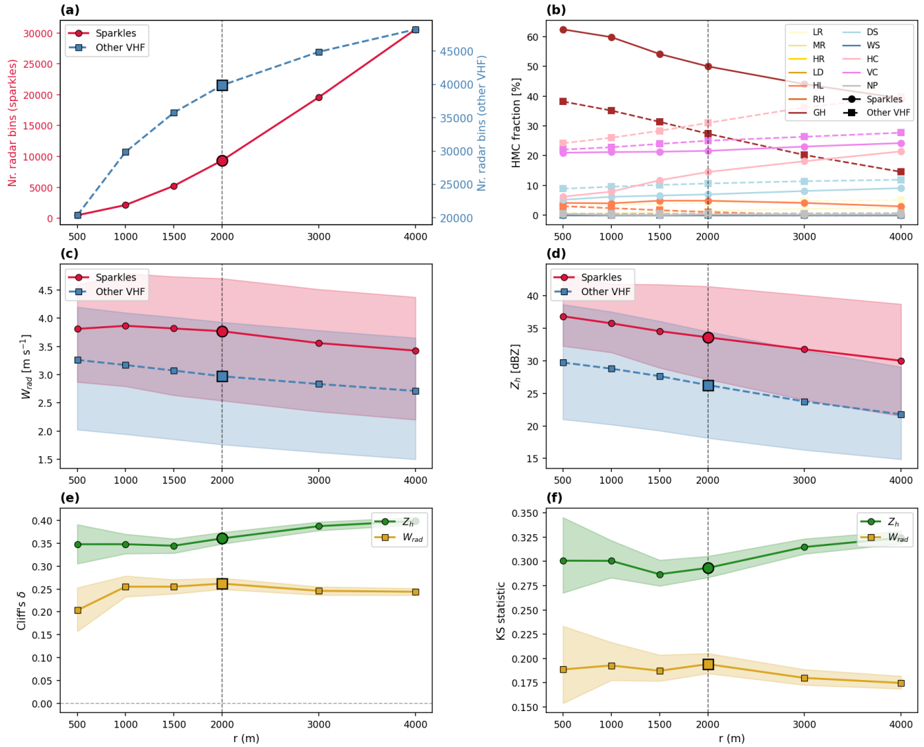
Figure S2.2. Sensitivity test of the radius r to collect radar data near VHF sources. (a) Number of radar points near sparkles (red circles, solid line) and near other VHF sources (blue squares, dashed line). (b) Fraction of the data in different HMC (hydrometeor classification) categories. (c) Mean W_{rad} values and with shading indicating the interquartile range. (d) Mean Z_h values and interquartile ranges. (e) Cliff's Delta between the distribution of sparkles versus the distribution of other VHF sources. Green for Z_h distributions, and yellow for W_{rad} distributions. Shading shows the 95% confidence intervals of Cliff's \delta based on a bootstrapping method. (f) Kolmogorov-Smirnov (KS) test statistic between sparkles and other VHF distributions. Shading indicates the 95% confidence interval from a bootstrapping method.
