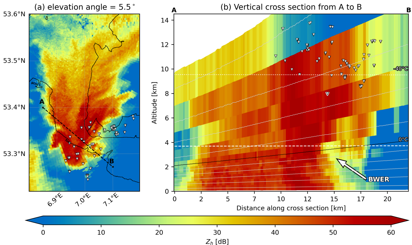
Figure 5. Radar reflectivity ( Z_h ) at 19:17:36 UTC with sparkles superimposed. Panel (a) shows a top view of the 5.5^\circ elevation scan with sparkles projected onto the horizontal plane. Panel (b) shows a vertical cross section along the A–B line in panel (a), with sparkles within 10 km projected onto this plane. 0^\circ and -40^\circ isotherms are indicated by the dashed and dotted white lines respectively. Radar beams from multiple elevation angles are indicated by gray lines, and the 5.5^\circ beam from panel (a) is highlighted in black. The vertical extent of radar data in panel (b) does not reflect the actual 1^\circ beam width. The Bounded Weak Echo Region (BWER) is annotated.
