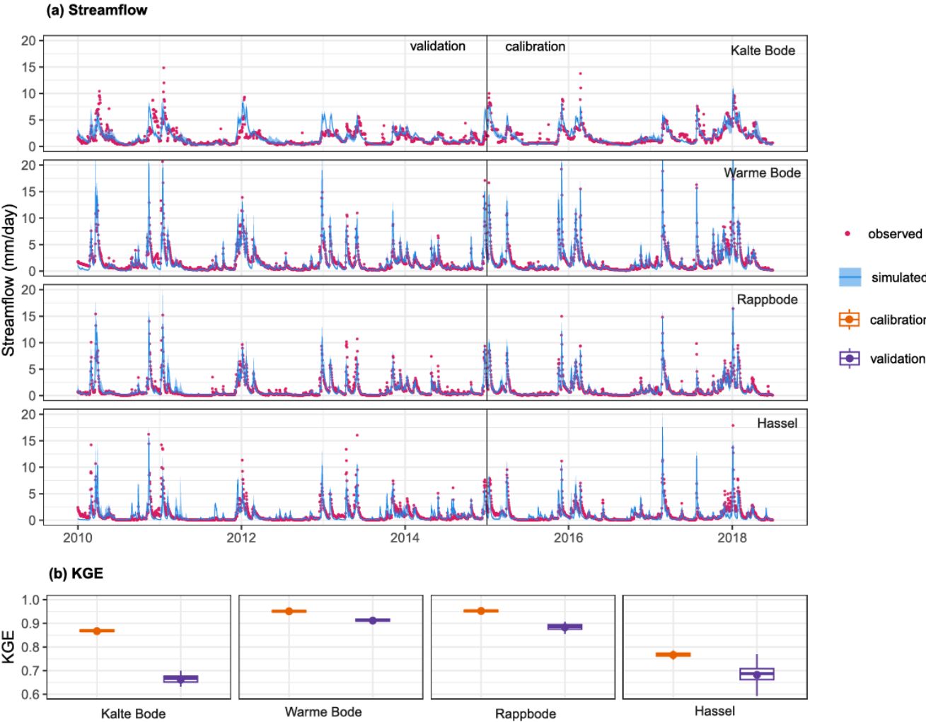
333 334 Figure 3: (a) Time series of observed and simulated streamflow and (b) the model performance (KGE) of 30 behavioural streamflow 335 simulations (the dots in the boxplots are the means). The solid lines and shaded areas (in blue) represent the medians and simulated
