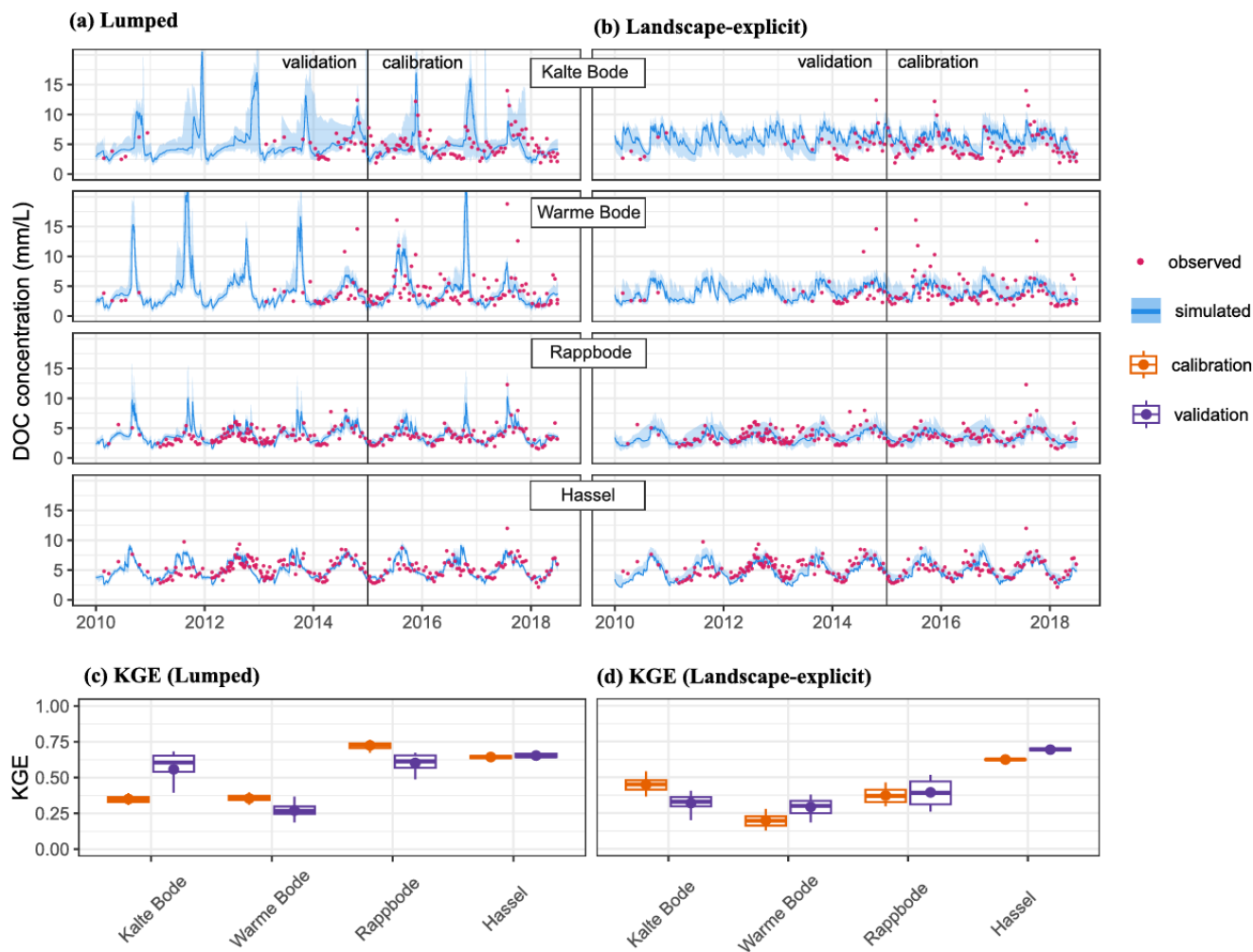
Figure 4: (a-b) Time series of observed and simulated stream DOC concentrations and (c-d) the model performance of 30 behavioural DOC simulations from (a, c) the lumped and (b, d) the landscape-explicit model structures during the calibration and validation of the baseline calibration. The solid lines and shaded areas (in blue) represent the medians and simulated ranges of these behavioural models. The dots in the boxplots are the means.
