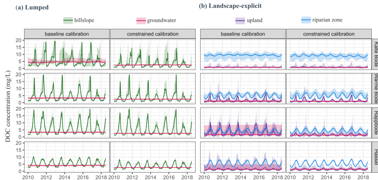
Figure 67: Internal DOC concentrations in different landscape units from (a) the lumped and (b) the landscape-explicit model structures under (a) the baseline and (b) constrained calibrations.
