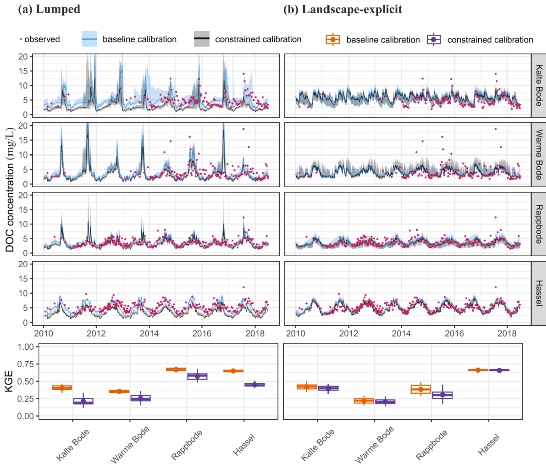
Figure 5: (a-b) Observed and simulated stream DOC concentration from (a) the lumped and (b) the landscape-explicit model structures under the baseline (blue) and constrained (grey) calibrations, along with the model performance (KGE-c-d) for both calibration and validation periods together instead of separating the results by calibration and validation periods . Simulated results were taken from 30 behavioural DOC simulations. The dots in the boxplots are the means.
