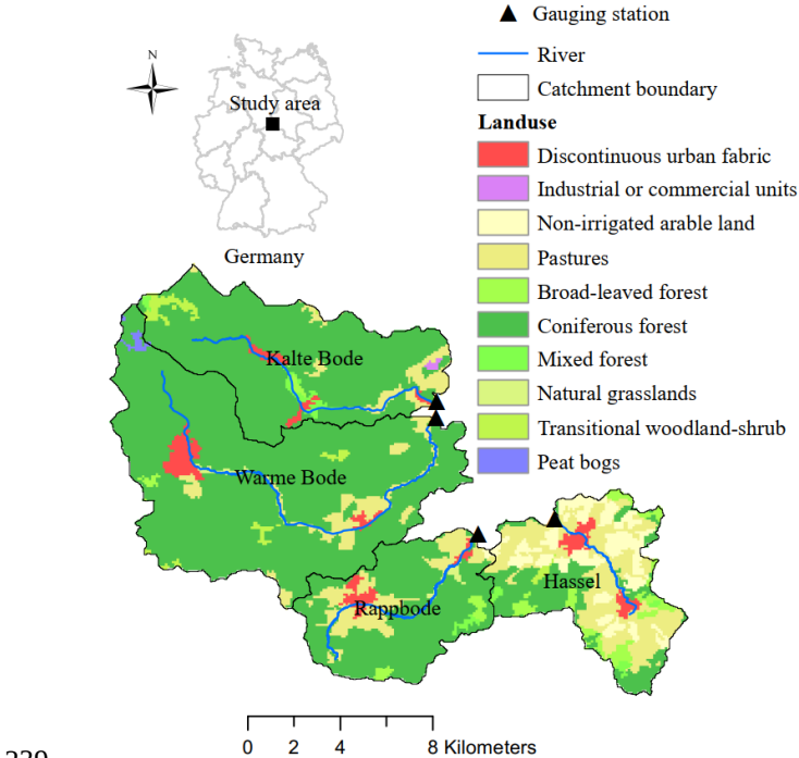
239 240 Figure 2: Location of the four study catchments in the Harz Mountains, Germany, and the CORINE land cover map in 2018.
