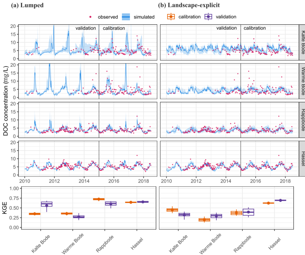
Figure 4: (a-b) Time series of observed and simulated stream DOC concentrations and (c-d) the model performance of 30 behavioural DOC simulations from (a, c) the lumped and (b, d) the landscape-explicit model structures during the calibration and validation of the baseline calibration . The solid lines and shaded areas (in blue) represent the medians and simulated ranges of these behavioural models. The dots in the boxplots are the means.
