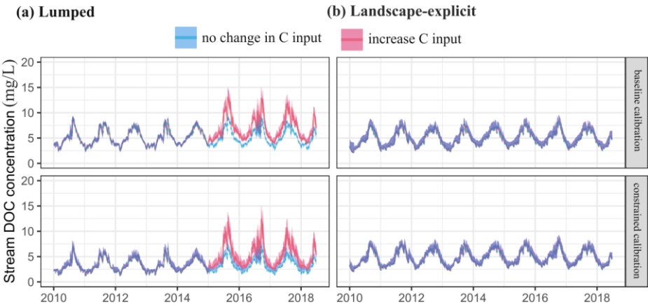
Figure 78: Simulated stream DOC concentrations in the Hassel catchment with increasing C input by 5 kg/ha for the period 2015-2018 (a) in the hillslope of the lumped model structure, and (b) in the upland of the landscape-explicit model structure.
