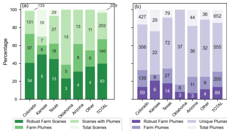
Figure 4. Summary of valid agricultural scenes (a) and associated plume detections (b) by state. Actual counts are displayed on each bar. Note: for Oklahoma, Arizona, and "Other," all valid scenes included plume detections. Additionally, all plumes detected in Oklahoma were classified as unique.
