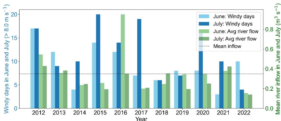
Figure 4. Number of windy days (wind speed > 8 \text{ m s}^{-1} ) at Boulogne-sur-Mer (Meteo-France station) and average river flow ( \text{m}^3 \text{ s}^{-1} ) from the Slack and Wimereux rivers during June and July (2012–2022). The dashed line indicates the mean June–July inflow of 0.35 \text{ m}^3 \text{ s}^{-1} . The blue bars indicate the number of days with wind speed > 8 \text{ m s}^{-1} during June–July and the green bars indicate mean June–July inflow.
