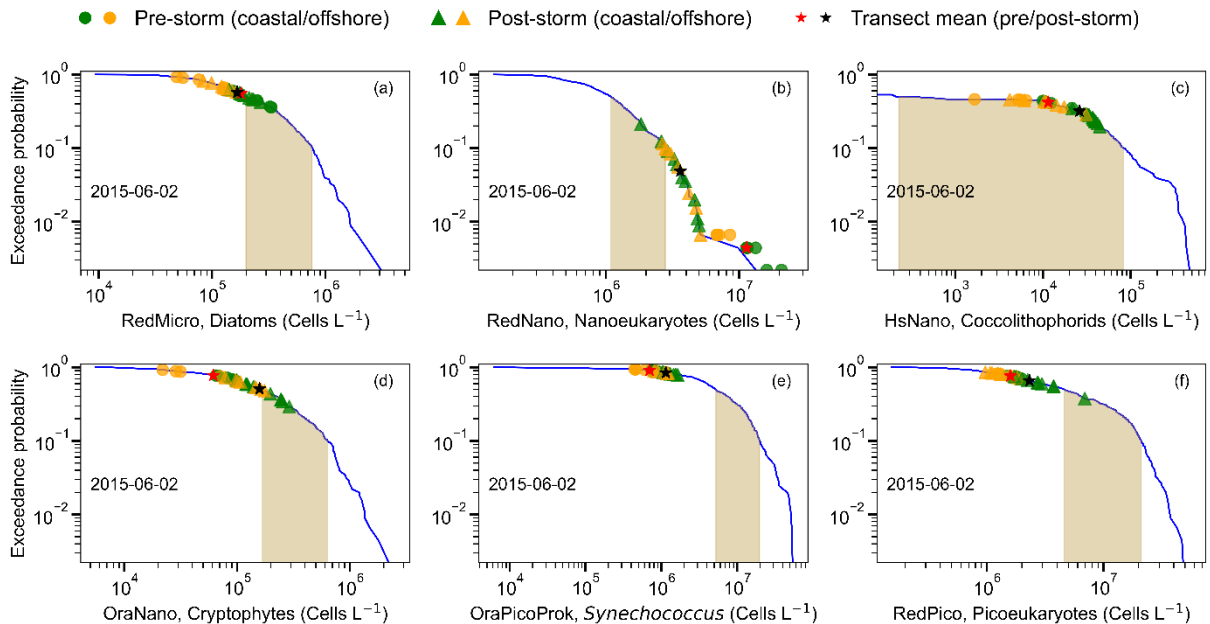
Figure F4. Exceedance probability (CCDF) distributions of six phytoplankton groups (a–f) along the DYPHYRAD transect during the storm of 2015-06-02. For each panel, RedMicro (diatoms), RedNano (nanoeukaryotes), HsNano (coccolithophorids), OraNano (cryptophytes), OraPicoProk ( Synechococcus ), and RedPico (picoeukaryotes) are presented. Blue lines represent June–July climatological distributions, with shaded areas indicating the 50 th –90 th percentiles. Pre-storm (–10 days) and post-storm (+14 days) observations are shown as green (coastal) and orange (offshore) symbols, with circles indicating pre-storm and triangles indicating post-storm abundances. Red and black stars indicate transect-mean abundances before and after the storm, respectively. Post-storm communities were initially dominated by Phaeocystis globosa , before being replaced by nanophytoplankton.
