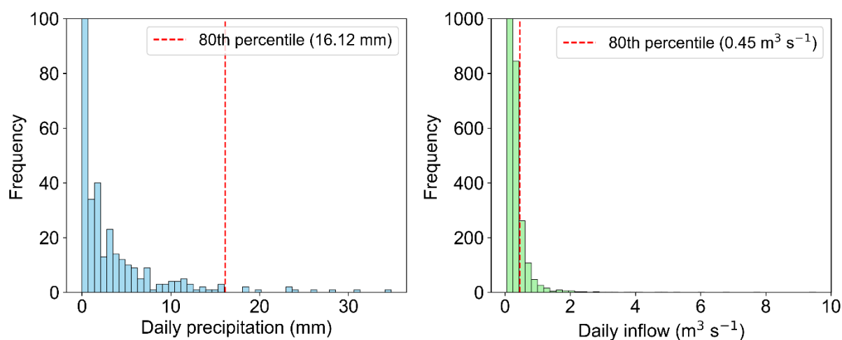
570 Figure B1. Frequency distributions of June–July precipitation (left) and river inflow (right) at the Boulogne-sur-Mer (Meteo-France station). Red dashed lines indicate the 80 th percentile thresholds (16.12 mm for precipitation; 0.45 m 3 s -1 for inflow), calculated from normalized \pm 3 -day total accumulated precipitation and mean inflow values. These thresholds were used to identify storm impacts as “High” or “Low” classes precipitation and river inflow.
