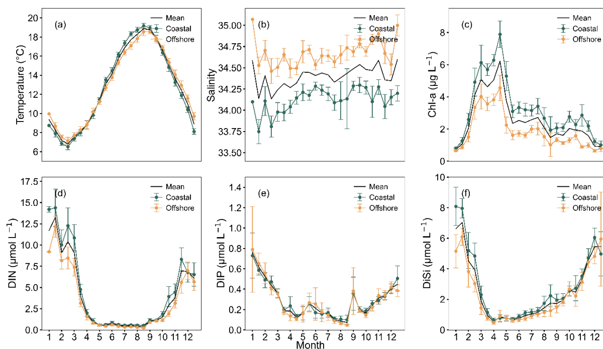
575 Figure C1. Climatological means and standard errors for Coastal (R0–R2 + SOMLIT C) and Offshore (R2'–R4 + SOMLIT L) regions of the EEC, based on 15-day means from February 2012 to December 2022. The black line represents the mean value across all stations. (a) sea temperature (°C), (b) salinity, (c) Chl-a (µg L -1 ), (d) dissolved inorganic nitrogen (DIN, µmol L -1 ), (e) dissolved inorganic phosphorus (DIP, µmol L -1 ), and (f) dissolved inorganic silicate (DiSi, µmol L -1 ). Coastal stations (R0–R2 + SOMLIT C) show stronger seasonal variability than offshore stations (R2'–R4 + SOMLIT L), particularly in salinity and Chl-a, reflecting coastal riverine influence. Chl-a exhibits two spring peaks (the first associated with diatoms and the second in April with P. globosa ), followed by a summer peak in June–July and a smaller autumn peak. Despite strongest nutrient limitation in June–July, Chl-a concentration remained elevated.
