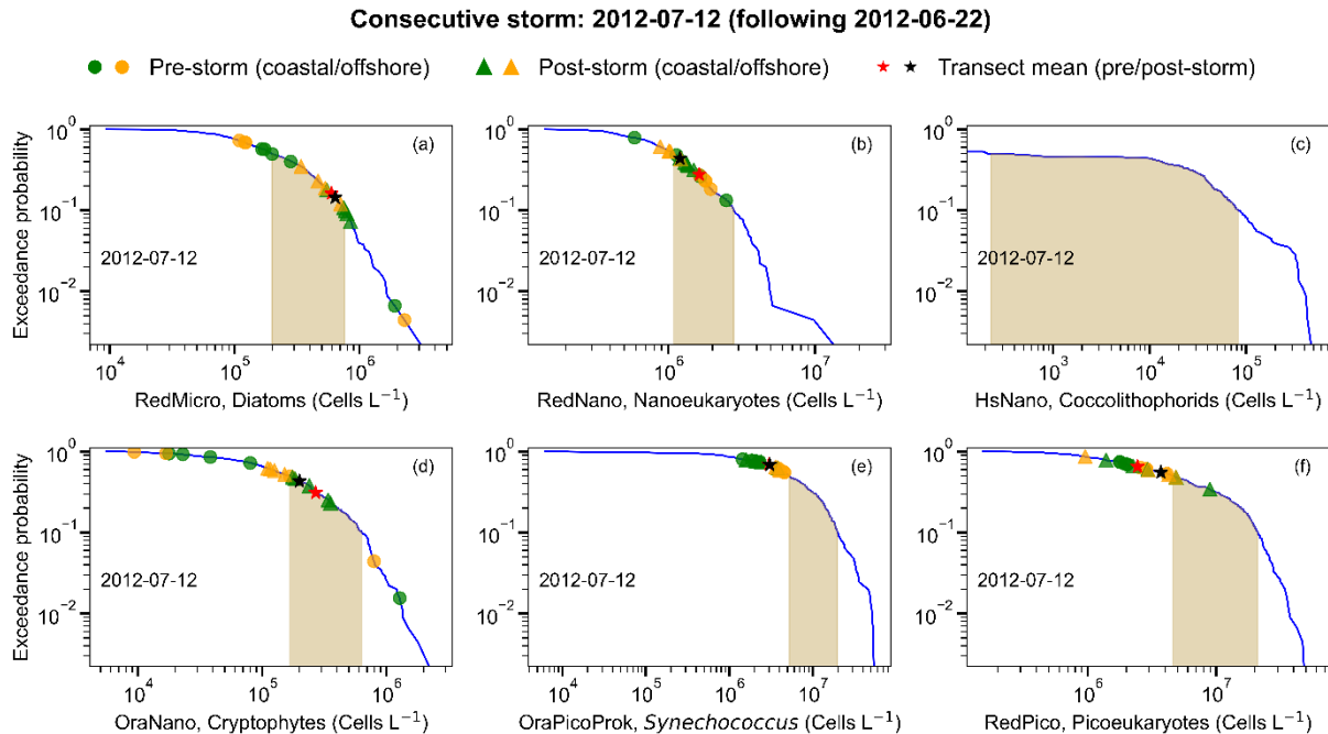
Figure F2. Exceedance probability (CCDF) distributions of six phytoplankton groups (a–f) along the DYPHYRAD transect during the storm of 2012-07-12. For each panel, RedMicro (diatoms), RedNano (nanoeukaryotes), HsNano (coccolithophorids), OraNano (cryptophytes), OraPicoProk ( Synechococcus ), and RedPico (picoeukaryotes) are presented. Blue lines represent June–July climatological distributions, with shaded areas indicating the 50 th –90 th percentiles. Pre-storm (–10 days) and post-storm (+14 days) observations are shown as green (coastal) and orange (offshore) symbols, with circles indicating pre-storm and triangles indicating post-storm abundances. Red and black stars indicate transect-mean abundances before and after the storm, respectively. Post-storm communities were dominated by diatoms and cryptophytes.
