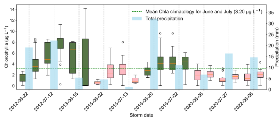
Figure E1 shows the pre- and post-storm distributions relative to precipitation occurring within \pm 3 days. Precipitation and post-storm chlorophyll a did not exhibit a linear relationship across storms.
