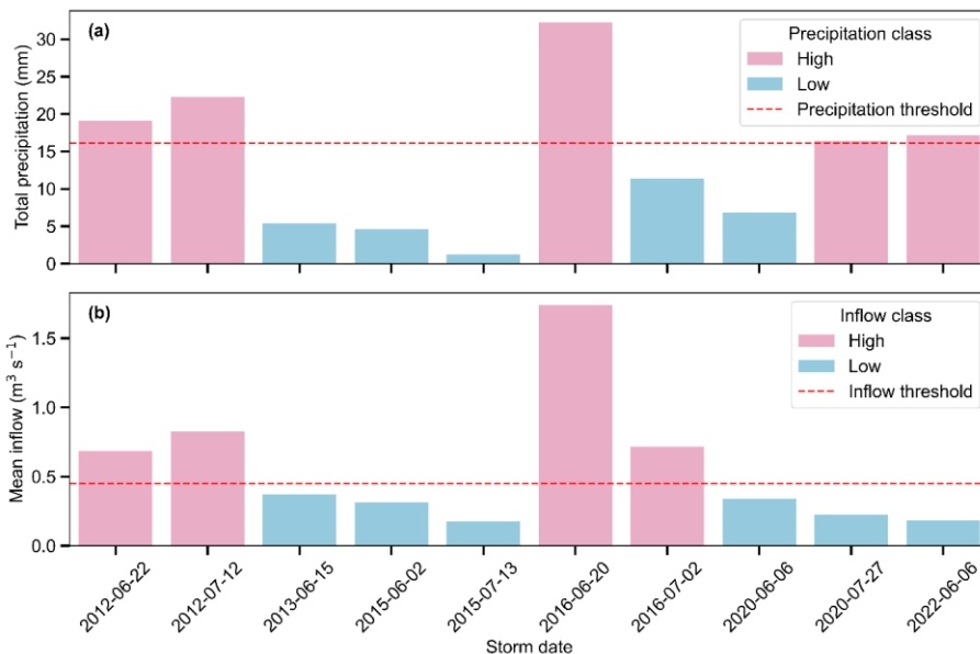
Figure 3. (a) Total precipitation (mm) over \pm 3 days at Boulogne-sur-Mer (Meteo-France station) (a) and mean river inflow ( \text{m}^3 \text{s}^{-1} ) (b) from the Slack and Wimereux rivers for 10 storms, averaged over \pm 3 days around each storm. Precipitation and inflow classes ("High" and "Low") were defined based on the 80 th percentile of their respective June–July distributions. The corresponding threshold values are 16.12 mm for precipitation and 0.45 \text{m}^3 \text{s}^{-1} for inflow. Precipitation classes ("High" and "Low") were defined from June–July rainfall distribution, with the high threshold set at 16.12 mm (80 th percentile); inflow classes were defined from June–July river-flow distribution, with the high threshold set at 0.45 \text{m}^3 \text{s}^{-1} (80 th percentile). Blue
