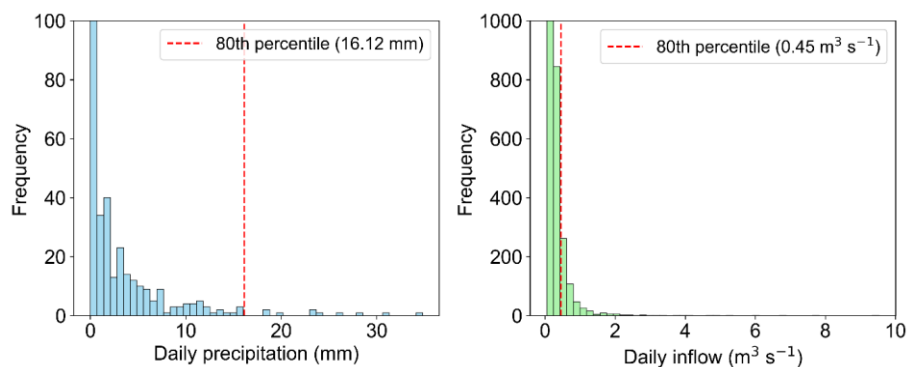
Figure B1. Frequency distributions of June–July precipitation (left) and river inflow (right) at the study site Boulogne-sur-Mer (Meteo-France station) . Red dashed lines indicate the 80 th -percentile thresholds (16.12 mm for precipitation; 0.45 m 3 s -1 for inflow), calculated from normalized \pm 3 -day total accumulated precipitation and mean inflow values. These thresholds were used to identify storm impacts as “High” or “Low” classes precipitation and river discharge inflow .
