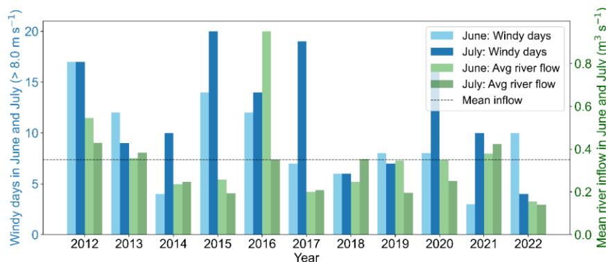
Figure 4. Number of windy days (wind speed > 8 m s -1 ) at Boulogne-sur-Mer (Meteo-France station) and average river flow (m 3 s -1 ) from the Slack and Wimereux rivers during June and July (2012–2022). The dashed line indicates the mean June–July inflow of 0.35 m 3 s -1 . The blue bars indicate the number of days with wind speed > 8 m s -1 during June–July and the green bars indicate mean June–July inflow.
