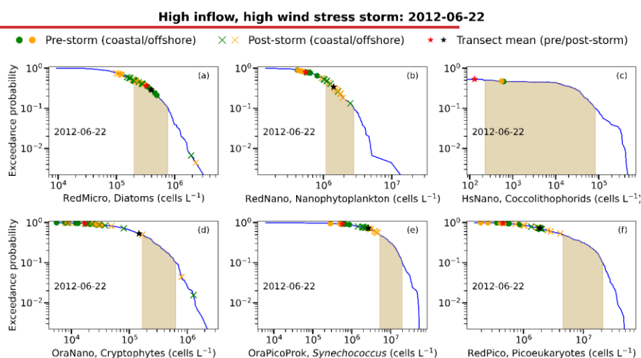
Figure F1. Exceedance probability (CCDF) distributions of six phytoplankton groups (a–f) along the DYPHYRAD transect during the storm of 2012-06-22. For each panel, RedMicro (diatoms), RedNano (nanoeukaryotes), HsNano (coccolithophorids), OraNano (cryptophytes), OraPicoProk ( Synechococcus ), and RedPico (picoeukaryotes) are presented shown as subplots (a–f). Blue lines represent June–July climatological distributions, with shaded areas indicating the 50 th –90 th percentiles. Pre-storm (–10 days) and post-storm (+14 days) observations are shown as green (coastal) and orange (offshore) symbols, with circles indicating pre-storm and triangles indicating post-storm abundances. Red and black stars indicate transect-mean abundances before and after the storm, respectively. Post-storm communities were dominated by diatoms and nanophytoplankton.
