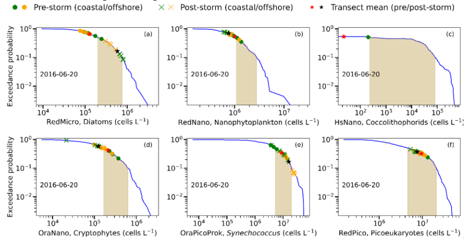
Fig. 7A — High inflow, low wind stress storm: 2016-06-20
