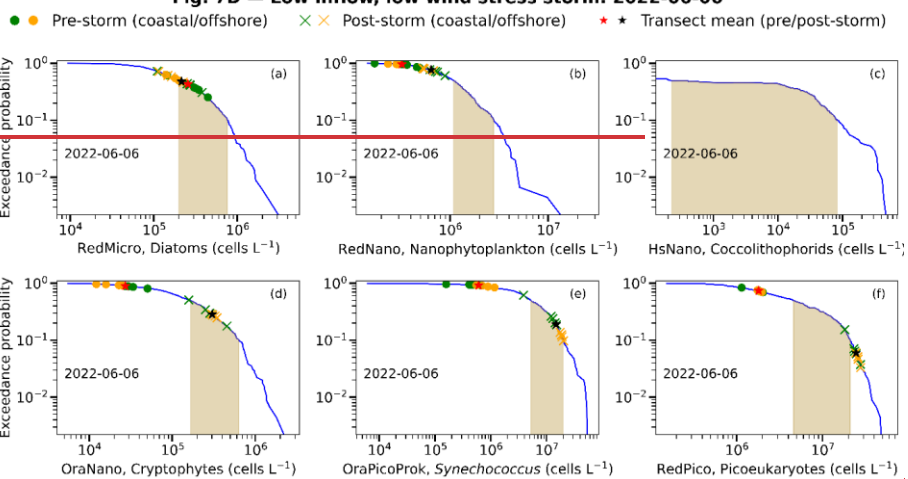
Fig. 7D — Low inflow, low wind stress storm: 2022-06-06
