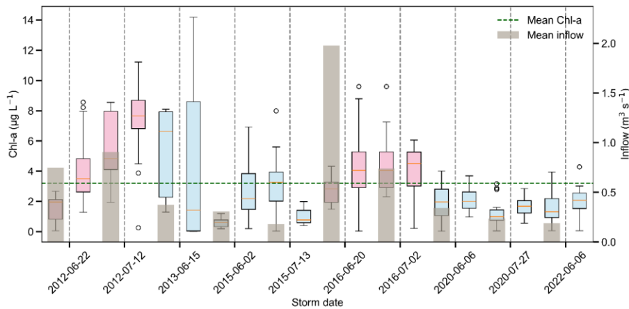
Figure 5. Boxplots of pre- and post-storm Chlorophyll a (Chl-a) distributions (compiled from DYPHYRAD and 400 SOMLIT) concentrations for before and after the 10 storms. Vertical dashed lines indicate the day of each storm event. Pre-storm Chl-a distributions are shown together with mean inflow over a \pm 3 -day storm period (grey bars), with river inflow (pink bars) and mean inflow (grey bars) overlaid. The green dashed line marks the June–July climatological mean of Chl-a concentration ( 3.20 \mu g L^{-1} ) in the eastern English Channel EEC. Pink and blue colouring indicate “High” and “Low” inflow storms, respectively. Data are compiled from DYPHYRAD and SOMLIT stations. Green and pink shading indicate “High” 405 and “Low” inflow storms, respectively.
