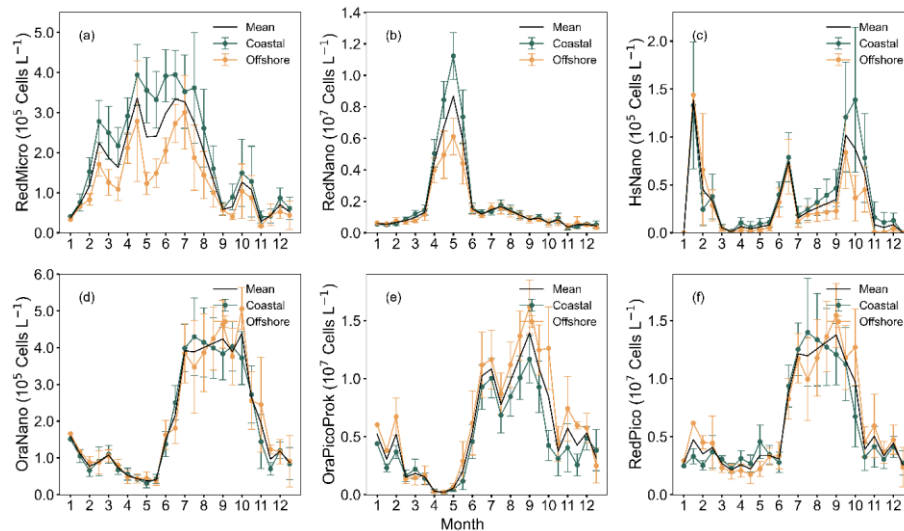
Figure 6. Climatological means and standard errors of phytoplankton abundances in the Coastal (R0–R2) and Offshore (R2'–R4) regions along the DYPRAD transect, based on 15-day means from February 2012 to December 2022. The black line represents the mean value across all stations. (a) RedMicro (diatoms), (b) RedNano (nanoeukaryotes), (c) HsNano (coccolithophorids), (d) OraNano (cryptophytes), (e) OraPicoProk ( Synechococcus ), and (f) RedPico (picoeukaryotes), respectively (see also Table 2). Seasonal and spatial variability of phytoplankton abundances in the eastern English Channel, based on 15-day climatological means from February 2012 to December 2022 estimated from DYPRAD data. Mean values (circles) and standard errors (error bars) are shown for coastal (green) and offshore (orange) stations. Subplots (a–f) represent RedMicro (diatoms), RedNano (nanophytoplankton), HsNano (coccolithophorids), OraNano (cryptophytes), OraPicoProk ( Synechococcus ), and RedPico (picoeukaryotes), respectively.
