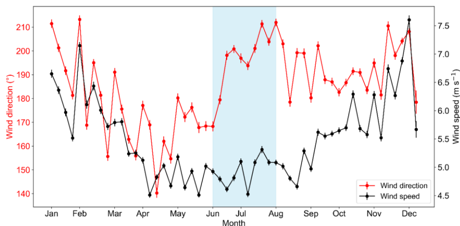
Figure D1. 15-day climatology of wind speed (black line, mean \pm SEM) and wind direction (red line, mean \pm SEM) at the study site Boulogne-sur-Mer (Meteo-France station), based on hourly measurements for 2010–2025. The shaded area highlights the June–July period used for the summer analysis, during which south-westerly winds dominate. The June–July period is characterized by a clear predominance of south-westerly winds, coinciding with the summer storm season.
