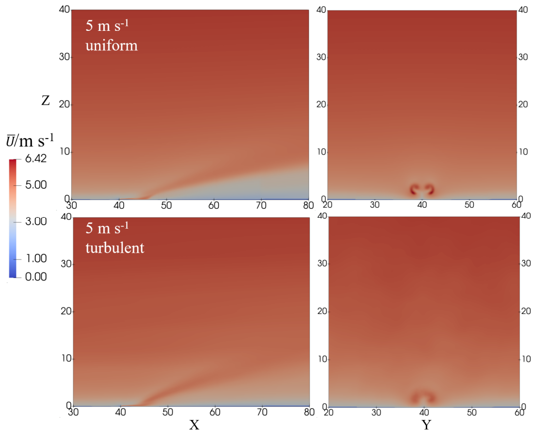
Figure 7 Mean velocity at the Y=40 m plane (left column) and X=50 m plane (right column) for U_0=5 m s -1 . First row for uniform condition, and second row for turbulent condition.
