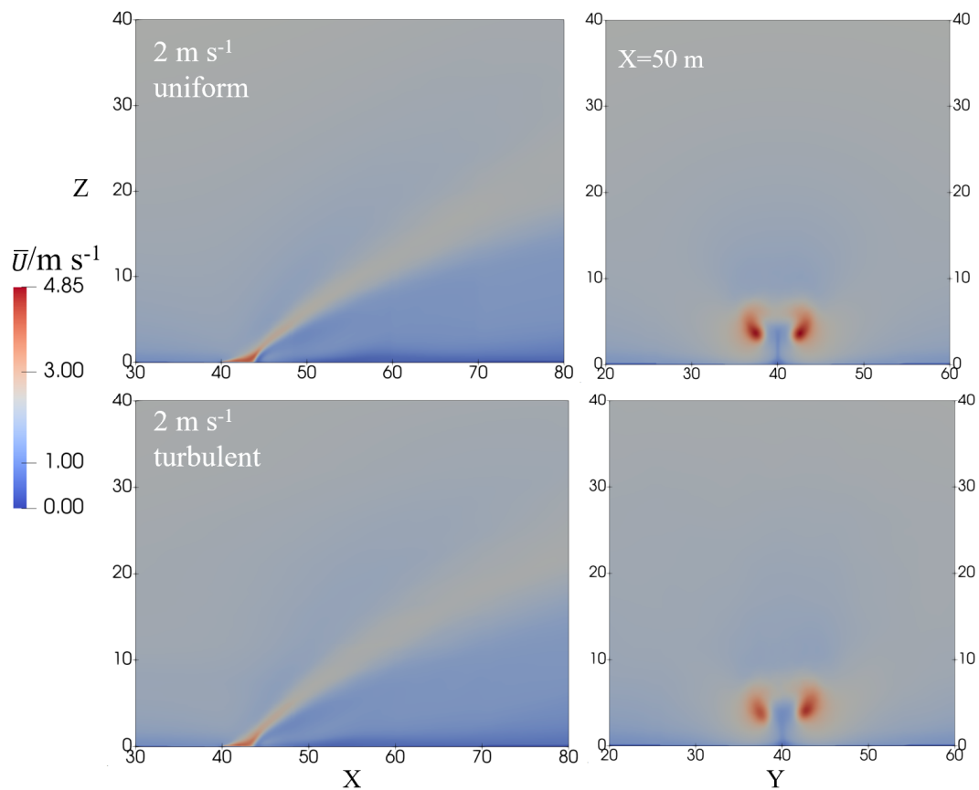
Figure 5 Mean velocity at the Y=40 \text{ m} plane (left column) and X=50 \text{ m} plane (right column) for U_0=2 \text{ m s}^{-1} . First row for uniform condition, and second row for turbulent condition.
