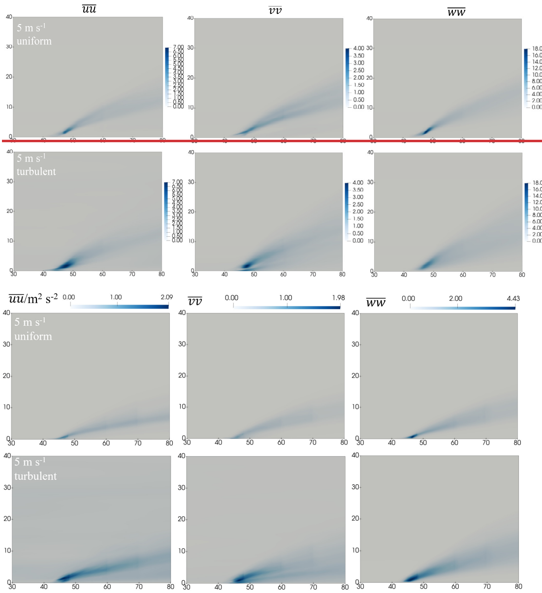
Figure 15 Mean velocity fluctuations of the fire plume for U_0=5\text{m s}^{-1} .
