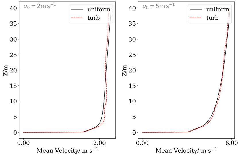
130 Figure 3 Mean streamwise velocities 2 m before the fire under different conditions. “uniform” means uniform inflow condition, “turb” means turbulent inflow condition.
