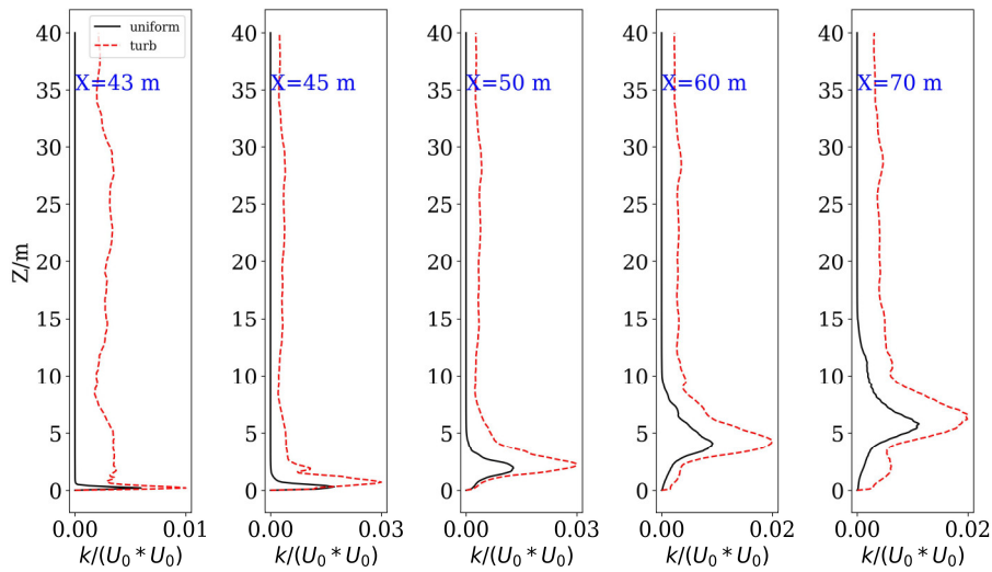
325 Figure 17 Turbulent kinetic energies ( k ) at different x locations for U_0=5\text{ m s}^{-1} . k is extracted from the middle Y plane.
