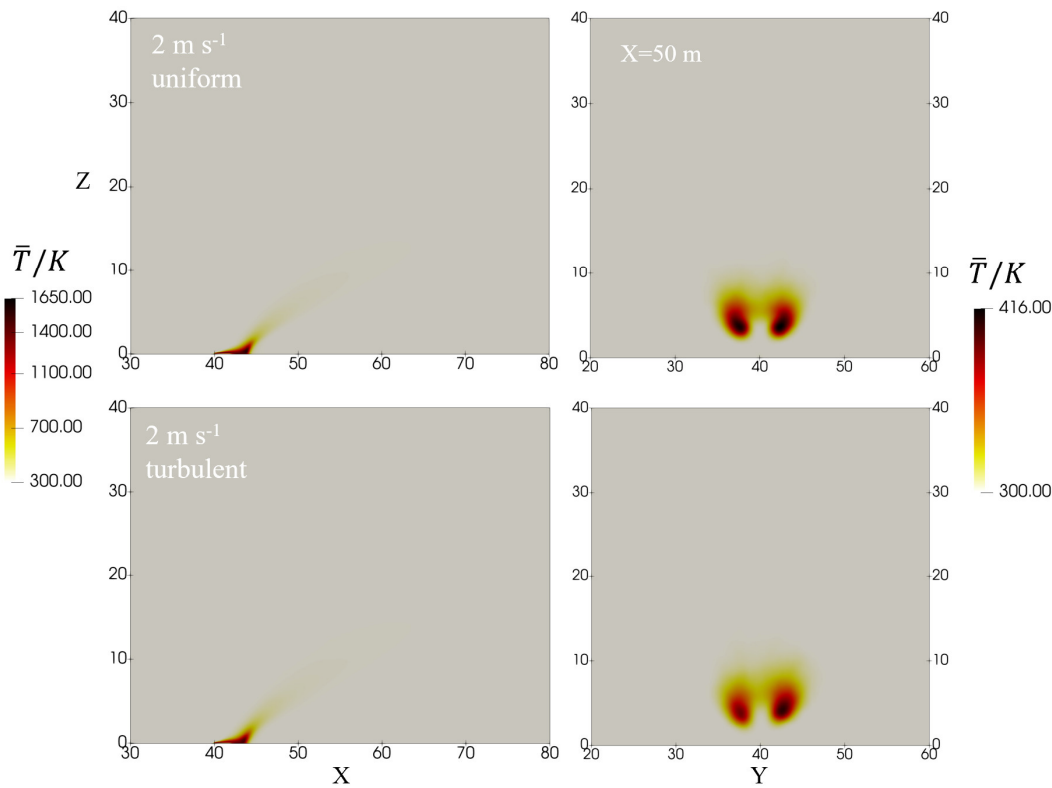
180 Figure 6 Mean temperature at the Y=40 m plane (left column) and X=50 m plane (right column) for U_0=2 m s^{-1} . First row for uniform condition, and second row for turbulent condition.
