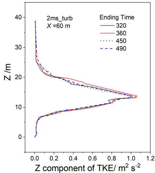
Fig. A1 Effect of time averaging window on the TKE distribution at X=60 m for the 2m s -1 turbulent case
