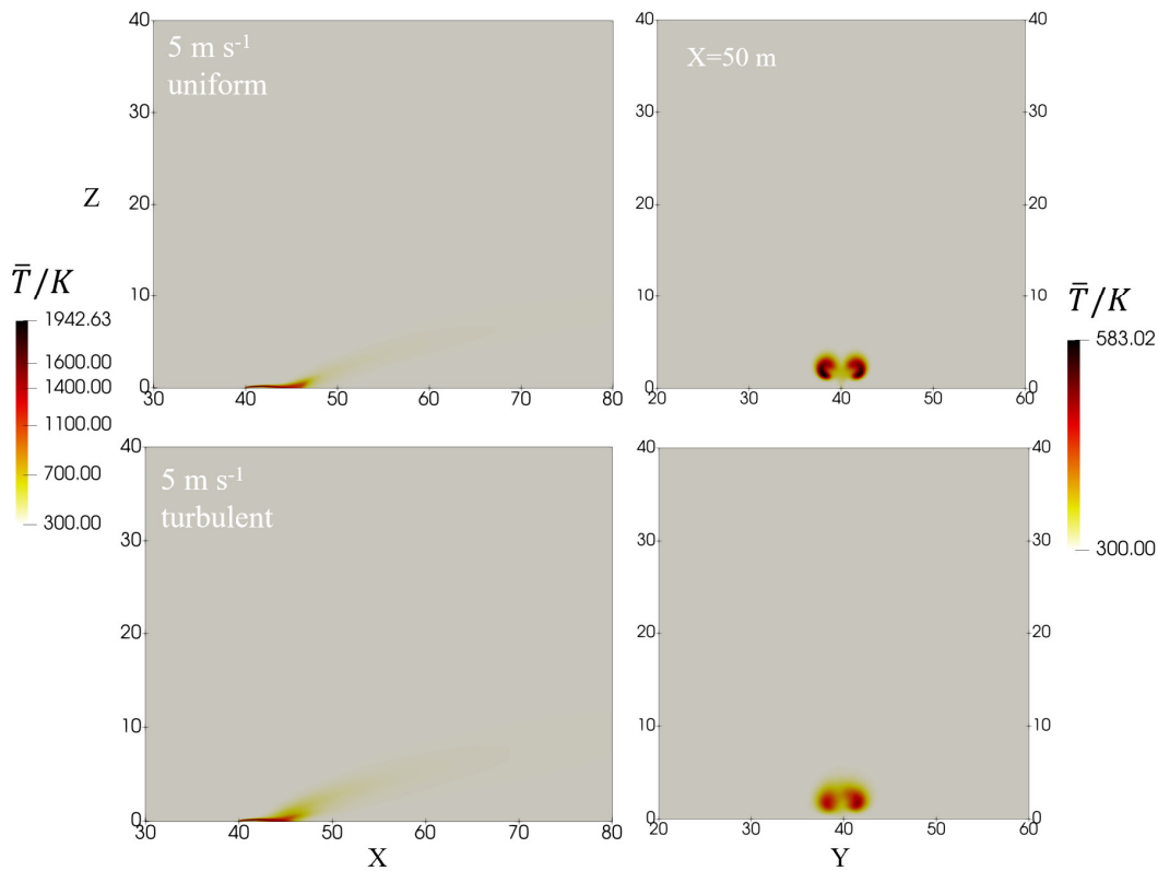
210 Figure 8 Mean temperature at the Y=40\text{m} plane (left column) and X=50\text{m} plane (right column) for U_0=5\text{m/s} . First row for uniform condition, and second row for turbulent condition.
