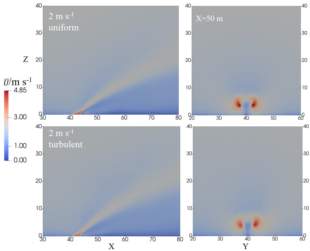
175 Figure 5 Mean velocity at the Y=40 m plane (left column) and X=50 m plane (right column) for U_0=2 \text{m s}^{-1} . First row for uniform condition, and second row for turbulent condition.
