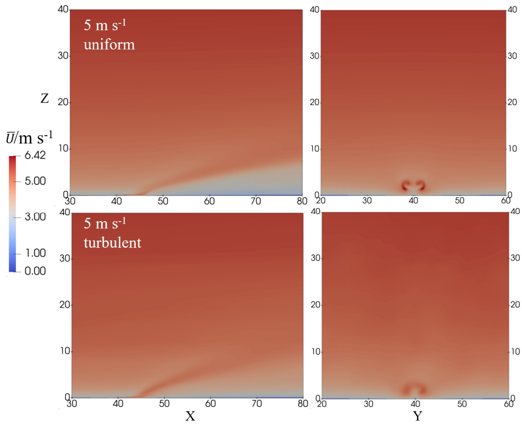
205 Figure 7 Mean velocity at the Y=40 m plane (left column) and X=50 m plane (right column) for U_0=5 m s -1 . First row for uniform condition, and second row for turbulent condition.
