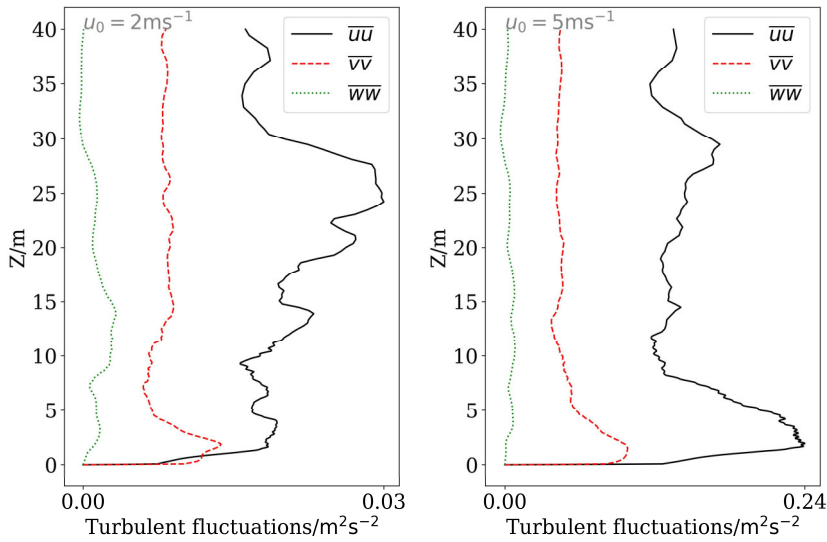
Figure 4 Mean velocities fluctuations 2 m before the fire source under different conditions. Velocities fluctuations under different conditions.
