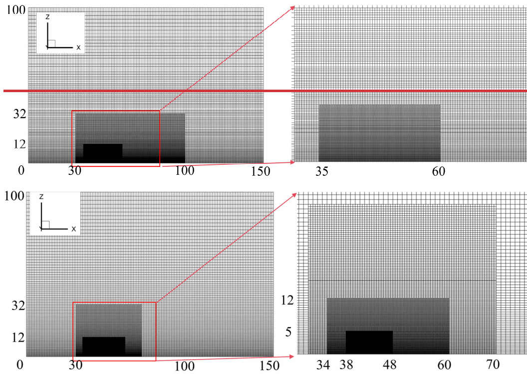
Figure 2 Schematic of refined mesh near the fire source
