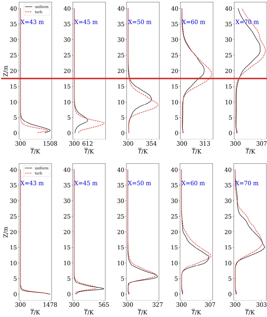
Figure 10 Mean temperature profiles at different X locations for U_0=2 \text{ m s}^{-1} . The temperatures are extracted from the middle Y plane.
