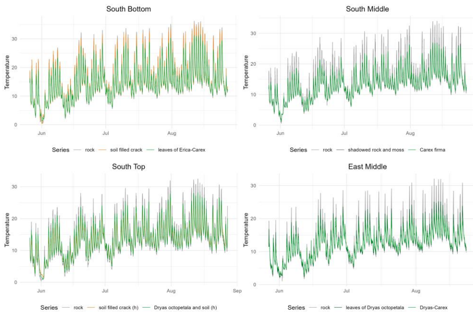
Figure A2: Development of the temperature in the rock with different cover at the surface from May 27 to Aug. 27.
