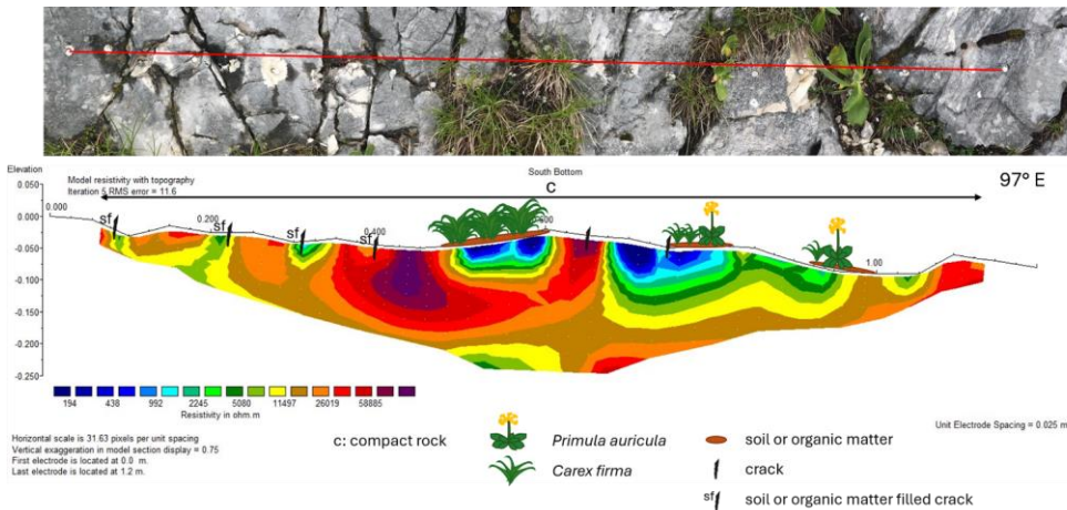
Figure 7: ERT profile at South Bottom (June 27, 2024): Top: Photo of the profile (profile length 120cm); Bottom: 2D-resistivity section, with blue colors representing low resistivity (high conductivity) and red colors high resistivity (low conductivity); complemented with information on cracks, soil and vegetation.
