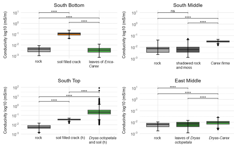
Figure 4: Distribution of the conductivity in the rock with different cover at the surface from May 27 to Aug. 27 (significance levels indicated by ns = not significant ( p > 0.05 ), **** p \leq 0.0001 )
