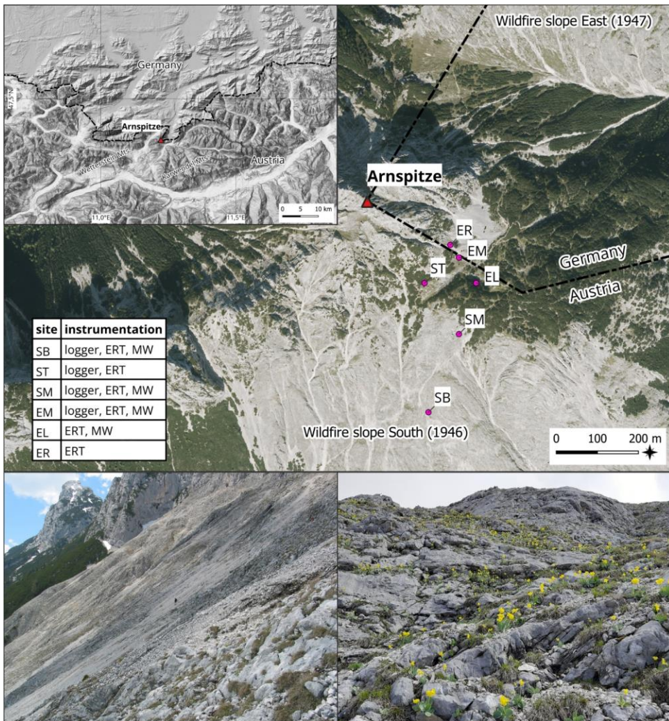
140 Figure 1: Location of the study area at the border between Germany and Austria (top left) and the study sites on the slopes of the Arnspitze; Background: Open street maps (top left); hillshade and contourlines processed from digital terrain model of the state of Tyrol (data.tirol.gv.at). Photos from the south-facing slope by OS.
