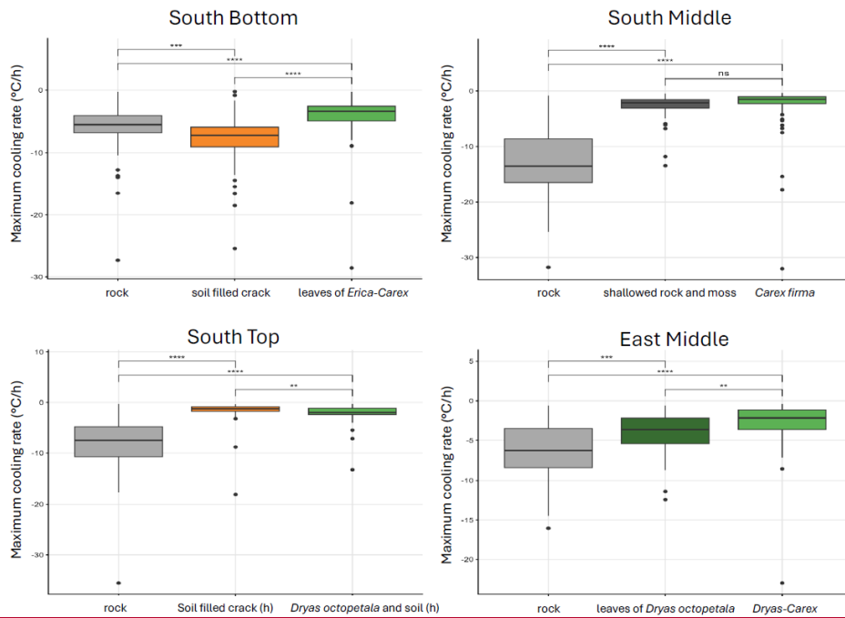
Figure A1: Maximum heating and cooling rates in the rock with different cover at the surface from May 27 to Aug. 27 (significance levels indicated by ns = not significant ( p > 0.05 ), * p < 0.05 , ** p < 0.01 , *** p < 0.001 , **** p < 0.0001 ). Temperature change rates are systematically higher in bare rock compared to vegetation cover. The notable exception of South Bottom / soil filled crack is thought to be caused by lower albedo of dark soil or lower heat capacity of dry soil compared to rock.
