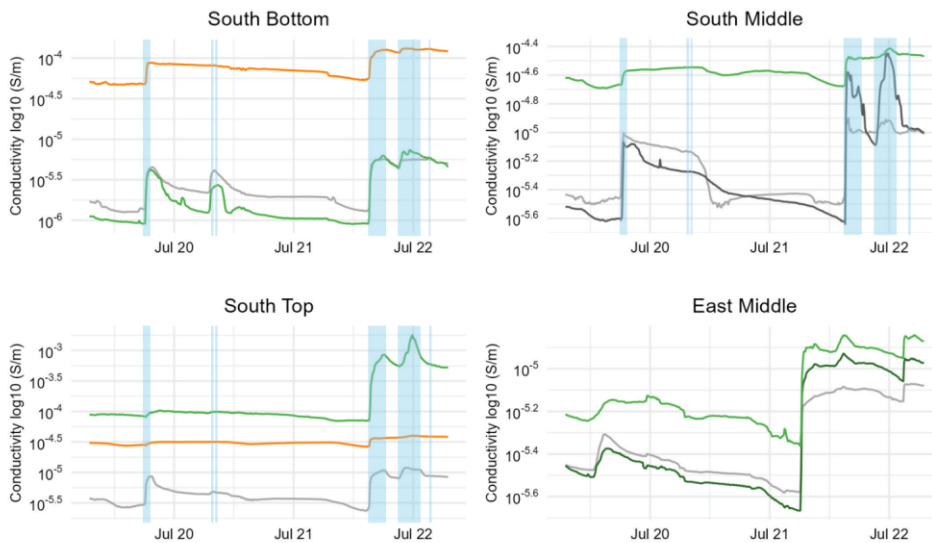
305 Figure 6: Response of conductivity in the rock on five rainfall events (19-22 July 2024) with different cover at the surface. At EM there is a time shift between rainfall and conductivity measurements due to logger malfunction which is why rainfall events are not shown.
