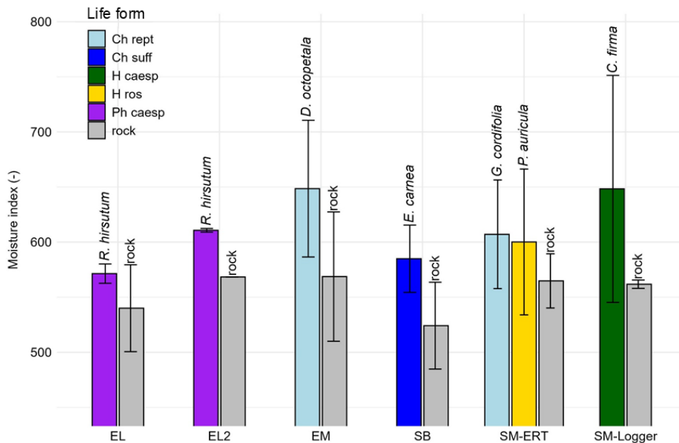
365 Figure 9: Dimensionless MW moisture index with cover of different plant species; 0-3 cm rock depth (life-plant forms according to Ellenberg and Mueller-Dombois (1967): Ch rept = mat-forming chamaephyte, Ch suff = subshrubby chamaephyte, H caesp = tufted hemicryptophyte, H ros = rosette hemicryptophyte, Ph caesp = tufted phanerophyte).
