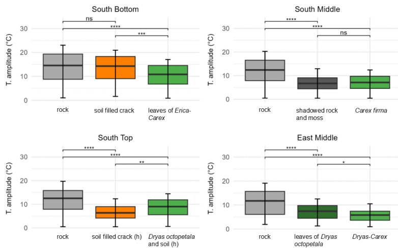
250 Figure 3: Distribution of the daily temperature amplitude in the rock with different cover at the surface from May 27 to Aug. 27 (significance levels indicated by ns = not significant ( p > 0.05 ), * p < 0.05 , ** p < 0.01 , *** p < 0.001 , **** p < 0.0001 )
