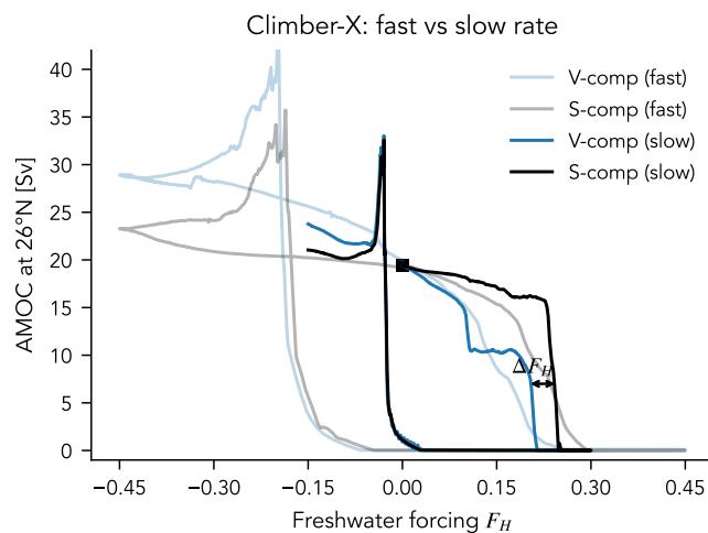
Figure B1. Comparison of AMOC hysteresis in Climber-X at two different rates: 0.3 Sv/kyr (“fast”; same as in POP) and 0.05 Sv/kyr (“slow”). \Delta H - \Delta F_H marks the difference in critical thresholds (as in Fig. 1) in the slow hysteresis. The “plateau” in the V-comp case at slow rates has been observed in some Climber-X hysteresis experiments before (Boot and Dijkstra, 2025) and does not appear appears to be a an intermediate stable state resembling the stable “weak AMOC” state of Willeit and Ganopolski (2024) .
