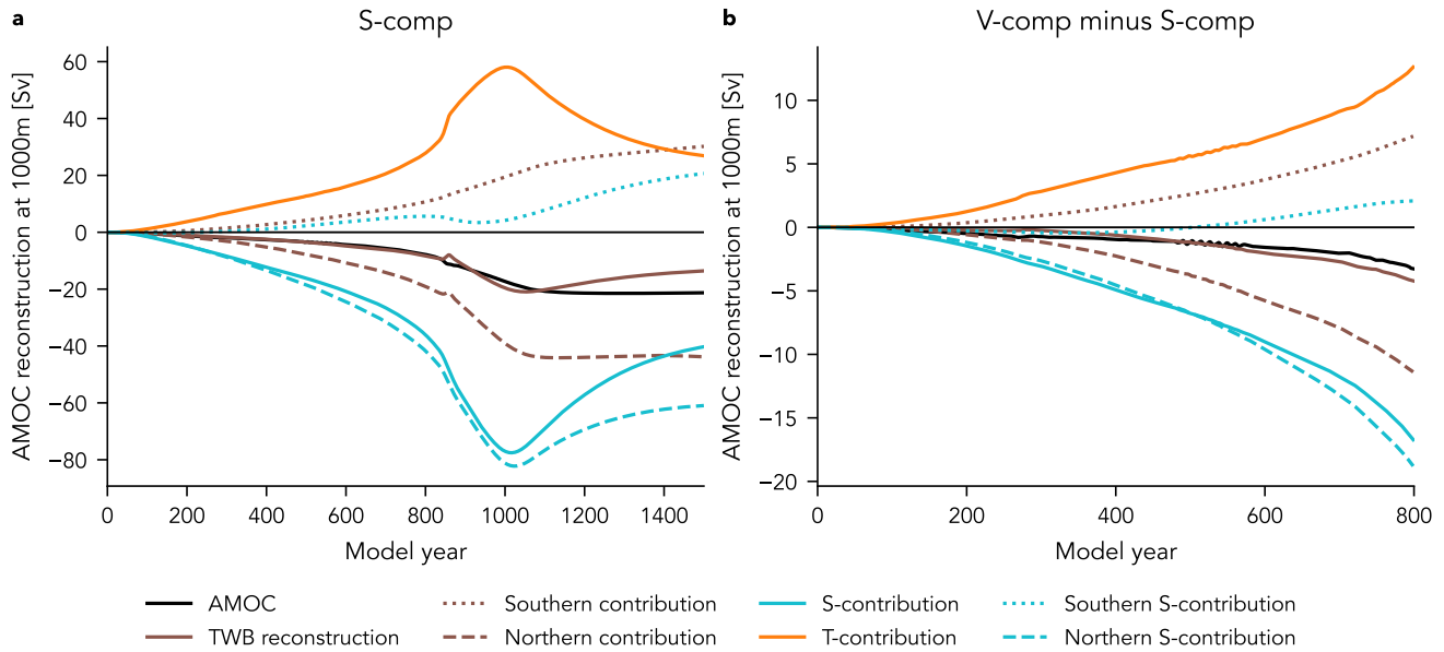
Figure 4. (a) Decomposition of the reconstructed AMOC anomalies in POP: (a) decomposition of AMOC anomalies in S-comp into contributions from temperature and salinity changes as well as density changes in the North and South Atlantic, (b) difference between V-comp and S-comp for each of the components. Note that only model years 1 to 800 are shown here.
