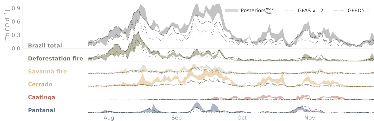
Figure A4. Same as Fig. 5 in the main text, but with the shaded area showing the full posterior range (minimum to maximum) instead of the posterior mean.
