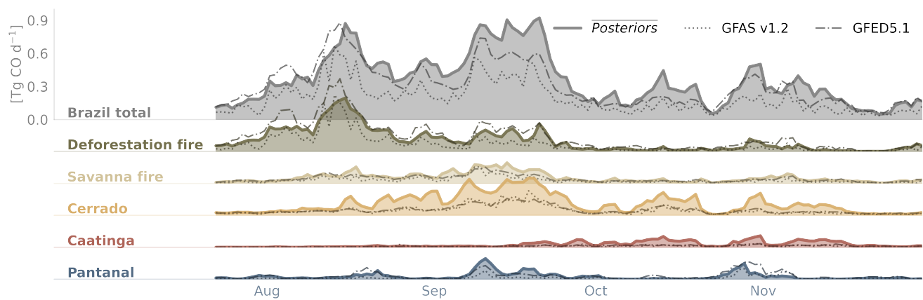
Figure 5. Daily evolution of CO fire emissions by biome. The filled areas and thick lines show the posterior mean of across the three inversions (GFED5.1_TROPOMI, GFED5.1_MOPITT, and GFASv1.2_TROPOMI), while the dashed lines indicate the corresponding priors (— GFED5.1, ... GFAS v1.2). The y-axis is shared across all biomes for direct comparison; successive ridges are spaced at 0.3 TgCO day -1 intervals and can serve as visual reference marks. The posterior spread can be found in Fig. A4.
