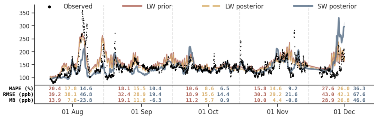
Figure 3. Comparison of measured and simulated CO mole fractions at the ATTO tower at 79 m measurement height (m.a.g.l.) measurement height. The lines represent the long-window prior (red), long-window posterior (yellow), and short-window posterior (blue). Shading around the mean ensemble member shows the one ensemble standard deviation of from the ensemble mean. The short-window posterior is based on derived from the GFED5.1_TROPOMI inversion. Monthly validation metrics — mean absolute percentage error (MAPE), root mean squared error (RMSE), and mean bias (MB) — are reported in the corresponding colours for each run.
