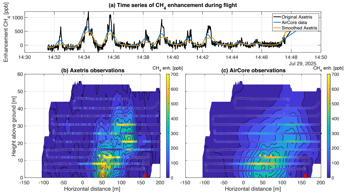
Figure J4: Overview of the observed \text{CH}_4 enhancements and spatial interpolation of flight 5. Estimated mass emission rate of Axetris 2.8 \text{ gCH}_4/\text{s} (B); AirCore 3.0 \text{ gCH}_4/\text{s} (C)
