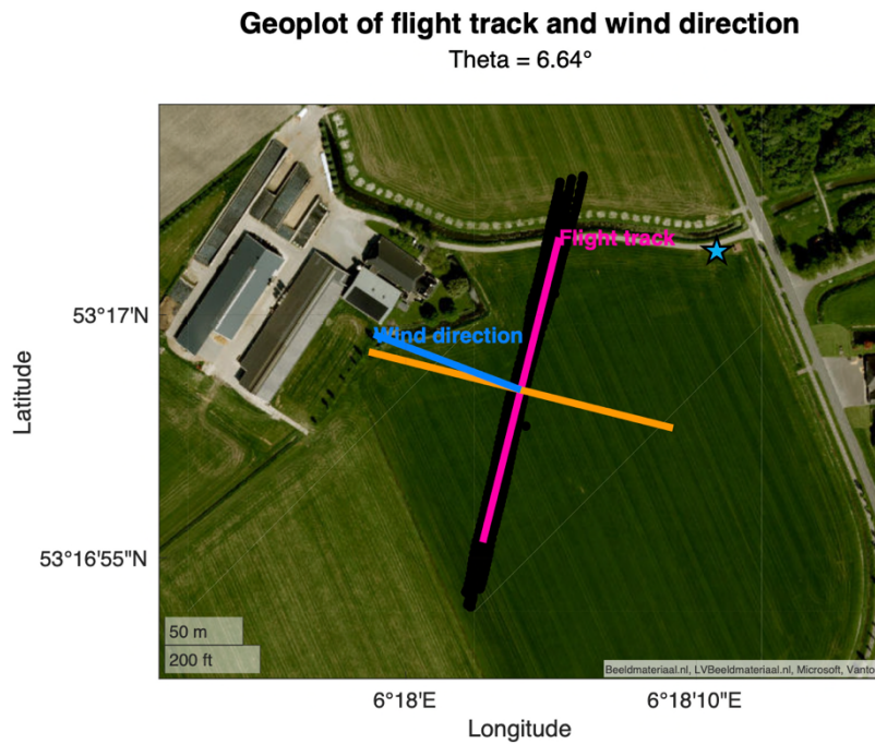
1120 Figure 11: Top-down view of the flight track and CH 4 observations of the Axetris during flight 1. Figure used to determine the angular deviation between the perpendicular line (orange line) of the mean flight track (pink line) and the wind direction (blue). The blue star represents the position of the WindMaster Pro. Images: © Microsoft
