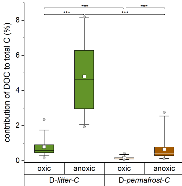
495 Figure A3: Contribution of the dissolved carbon fraction (DOC) to total litter-C and total permafrost-C recovered at the end of the experiment under oxic and anoxic incubation conditions. Significant differences are indicated by *** = p < 0.001 (Kruskal-Wallis ANOVA). The Box shows the 25/75 percentiles, the whiskers the 5/95 percentiles, the horizontal line the median and the white square the mean. Outliers are presented as circles.
