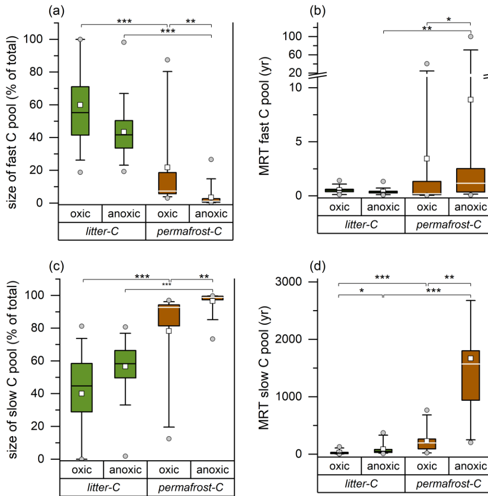
240 Figure 2: Size of the fast (a) and slow (c) litter-C and permafrost-C pools and mean residence times (MRT) of the respective carbon pools (b, d) determined by a two-pool carbon decomposition model. Significant differences are indicated by * = p < 0.05 , ** = p < 0.01 and *** = p < 0.001 (Kruskal-Wallis ANOVA). The Box shows the 25/75 percentiles, the whiskers the 5/95 percentiles, the horizontal line the median and the closed square the mean. Outliers are presented as open circles.
