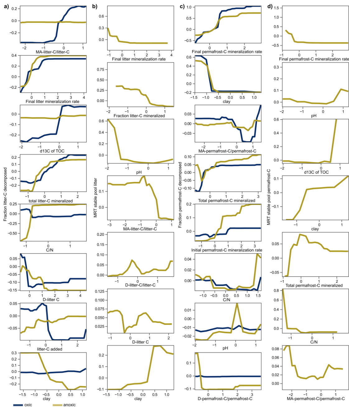
490 Figure A2: Partial dependence plots for Random Forest models, showing the responses of predictors used in Fig. 4. Panels show the fraction of litter-C decomposed (a), the mean residence time (MRT) of stable litter-C pool (b), the fraction of permafrost-C decomposed (c) and the MRT of the stable permafrost-C pool (d) under oxic and anoxic conditions. Note that variables were scaled prior to analyses using z-score centring.
