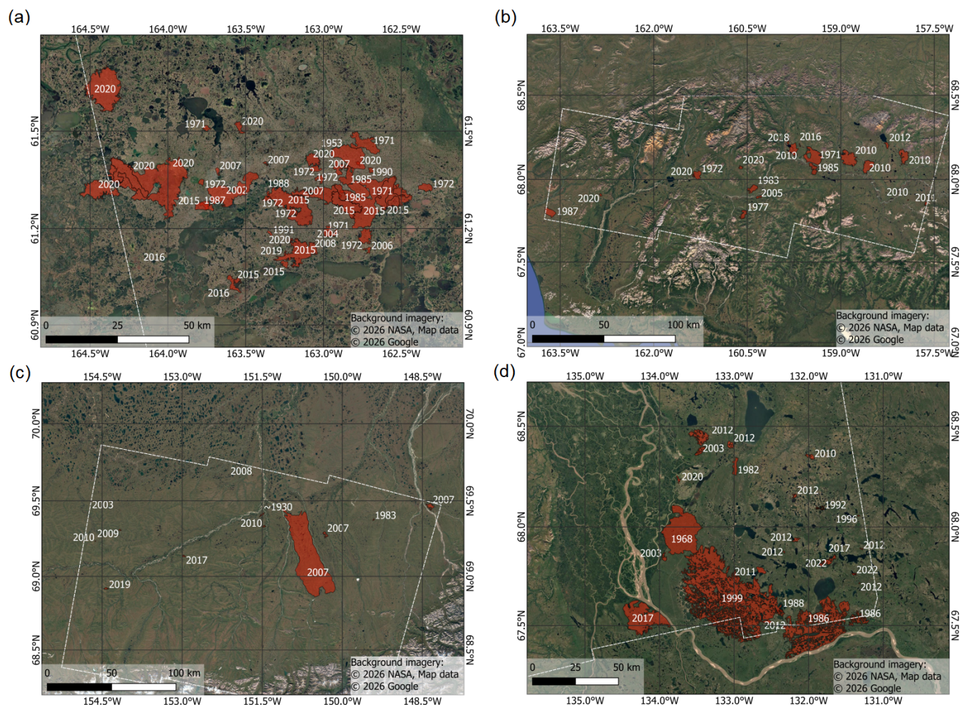
Figure 2. a)-d) Fire scars analyzed in this study and fire years of the study regions a) Yukon-Kuskokwim Delta, b) Noatak River Basin, c) Central North Slope, d) Inuvik region. Dashed white lines indicate the analysis boundary. (Fire scars of a)-c), with the exception of the prehistoric Shivugak Bluffs Burn in c), derived from the Alaska large fire database (Kasischke et al., 2002) and d) Fire History dataset from the Government of the Northwest Territories (NWT Centre for Geomatics). Background imagery: © 2026 NASA, Map data © 2026 Google Satellite)
