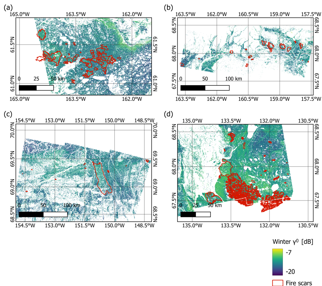
Figure A6. Sentinel-1 winter backscatter maps for the study regions a) Yukon-Kuskokwim Delta, b) Noatak River Basin, c) Central North Slope, d) Inuvik region. Values represent the median of all calculated years. For the sources of fire scars, see Section 3.3.
