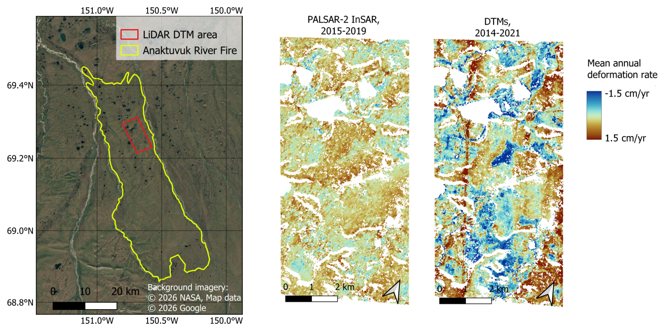
Figure 9. Comparison of annual ground deformation rate maps derived from PALSAR-2 InSAR data (2015–2019) and downsampled LiDAR DTMs (Jones et al., 2024b) (2014–2021) for a 50 km 2 area within the Anaktuvuk River tundra fire scar (fire event 2007). The left panel shows the extent of the Anaktuvuk River fire scar and the location of the LiDAR DTM analysis area, which is displayed in the deformation maps on the right. (Background imagery of left panel: © 2026 NASA, Map data © 2026 Google Satellite)
