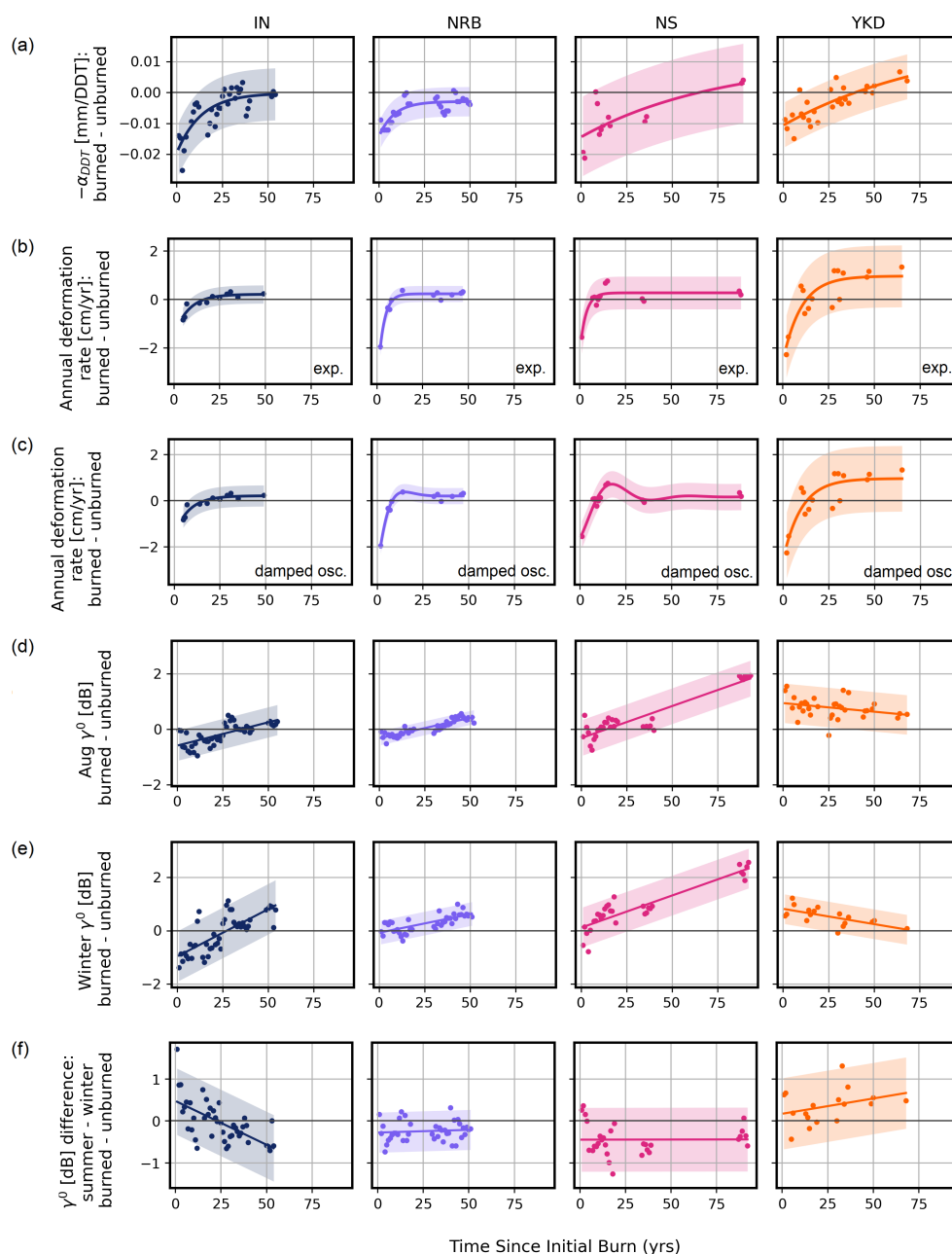
Figure 4. Dependence of investigated parameters on fire scar age. Parameter values of the fire scars were normalized by subtracting the unburned buffer area values and averaged per year and study region (NRB: Noatak River Basin, NS: Central North Slope, YKD: Yukon-Kuskokwim Delta.) The shaded regions represent the 95% confidence interval of the fitted models. Both exponential (Michaelides et al., 2019) and damped oscillation models (Cao and Furuya, 2025) were tested to describe the annual deformation rates.
