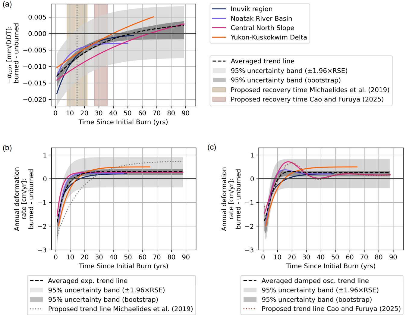
Figure 5. Regionally merged representation of Figures 4a, b and c representing the analyzed parameters as a function of fire scar age: a) -\alpha_{DDT} and fitted exponential functions, b) annual deformation rate and fitted exponential functions c) annual deformation rate and fitted damped oscillation functions. Two alternative 95% uncertainty bands are shown for comparison: (1) the light grey band shows the interval estimated as the predicted value \pm 1.96 times the residual standard error, based on all regional data points shown in Figure 4; (2) the dark grey band was computed using a parametric bootstrap (2000 samples) based on all regional data points shown in Figure 4, and defined as the 2.5th and 97.5th percentiles of the resulting predictions. The vertical bands in a) indicate the proposed recovery time of the thaw season deformation according to Fig. 7 in Michaelides et al. (2019) and Cao and Furuya (2025). Dotted lines b) and c) represent the functions suggested by Michaelides et al. (2019) and Cao and Furuya (2025) for annual deformation rates. Average and literature-based annual deformation rate functions are listed in Table A9.
