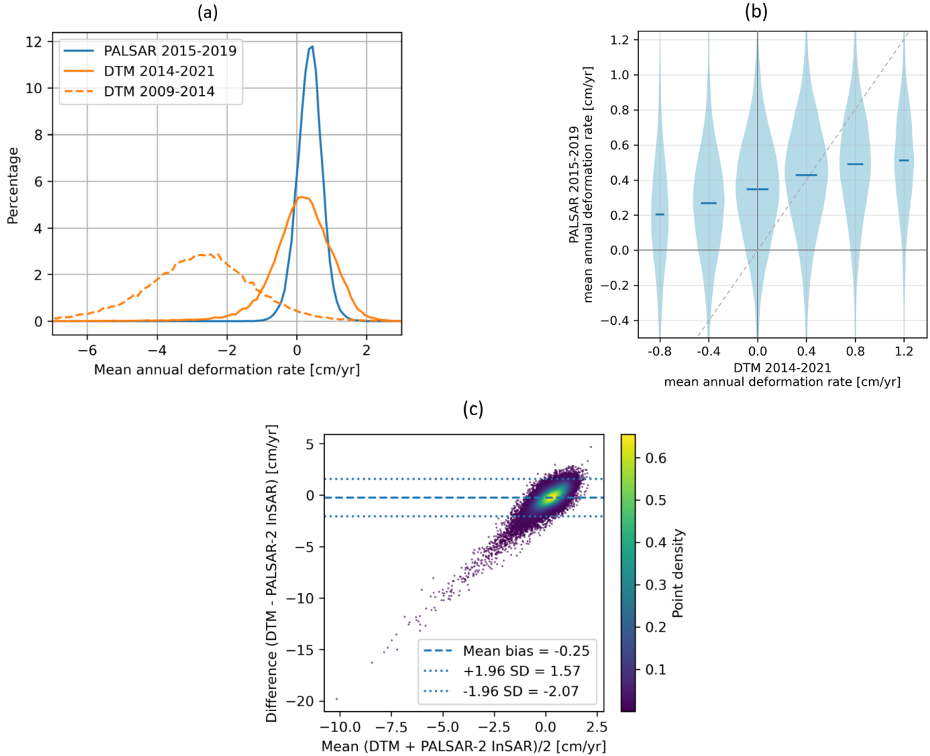
Figure 10. Anaktuvuk River tundra fire scar (fire event 2007) assessment: a) Histograms of annual deformation rate from PALSAR-2 InSAR for the period 2015-2019, and annual deformation rate values derived from downsampled LiDAR DTMs (Jones et al., 2024b) for the periods 2009-2014 and 2014-2021 for a 50 km 2 area within the fire scar. The histograms use a bin size of 0.1 cm/yr. b) Annual deformation rate from PALSAR-2 InSAR for the period 2015-2019 statistics (violin plot) by annual deformation rate bins (bin size 0.4 cm/yr) derived from downsampled LiDAR DTMs (Jones et al., 2024b) for the periods 2014-2021. Median values are shown as vertical lines; violin widths reflect the sample size. c) Bland-Altman plot of annual deformation rates from PALSAR-2 InSAR (2015-2019) and downsampled LiDAR DTMs (Jones et al., 2024b) (2014-2021). The dashed line indicates the mean bias (-0.25 cm/yr) and the dotted lines indicate the 95% limits of agreement (-2.07 to +1.57 cm/yr). The color indicates the point density.
