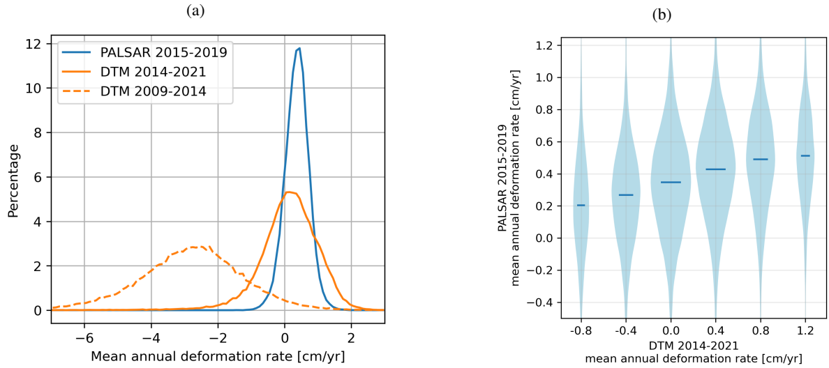
Figure 10. a) Histograms of annual deformation rate from PALSAR-2 InSAR for the period 2015-2019, and annual deformation rate values derived from downsampled LiDAR DTMs (Jones et al., 2024b) for the periods 2009-2014 and 2014-2021 for a 50 km 2 area within the Anaktuvuk River tundra fire scar (fire event 2007). The histograms use a bin size of 0.1 cm/yr. b) Annual deformation rate from PALSAR-2 InSAR for the period 2015-2019 statistics (violin plot) by annual deformation rate bins (bin size 0.4 cm/yr) derived from downsampled LiDAR DTMs (Jones et al., 2024b) for the periods 2014-2021. Median values are shown as vertical lines; violin widths reflect the sample size.
