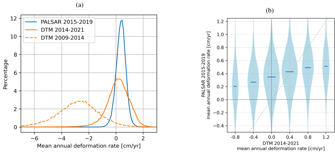
(c) a) Histograms of annual deformation rate from PALSAR-2 InSAR for the period 2015-2019, and annual deformation rate values derived from downsampled LiDAR DTMs (Jones et al., 2024b) for the periods 2009-2014 and 2014-2021 for a 50 km 2 area within the Anaktuvuk River tundra fire scar (fire event 2007). The histograms use a bin size of 0.1 cm/yr. b) Annual deformation rate from PALSAR-2 InSAR for the period 2015-2019 statistics (violin plot) by annual deformation rate bins (bin size 0.4 cm/yr) derived from downsampled LiDAR DTMs (Jones et al., 2024b) for the periods 2014-2021. Median values are shown as vertical lines; violin widths reflect the sample size.
