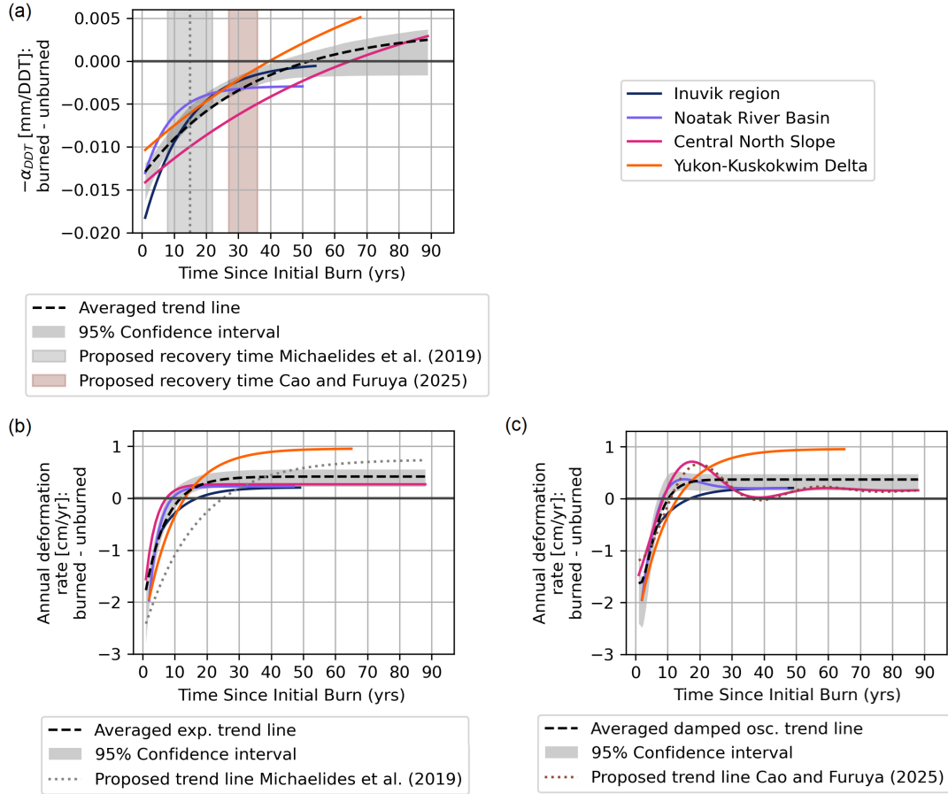
Figure 5. Regionally merged representation of Figures 4a, b and c representing the analyzed parameters as a function of fire scar age: a) -\alpha_{DDT} and fitted exponential functions, b) annual deformation rate and fitted exponential functions c) annual deformation rate and fitted damped oscillation functions. The 95% confidence intervals were computed using a parametric bootstrap (2000 samples) based on all regional data points shown in Figure 4, and defined as the 2.5th and 97.5th percentiles of the resulting predictions. The vertical bands in a) indicate the proposed recovery time of the thaw season deformation according to Fig. 7 in Michaelides et al. (2019) and Cao and Furuya (2025). Dotted lines b) and c) represent the functions suggested by Michaelides et al. (2019) and Cao and Furuya (2025) for annual deformation rates. Average and literature-based annual deformation rate functions are listed in Table A9.
