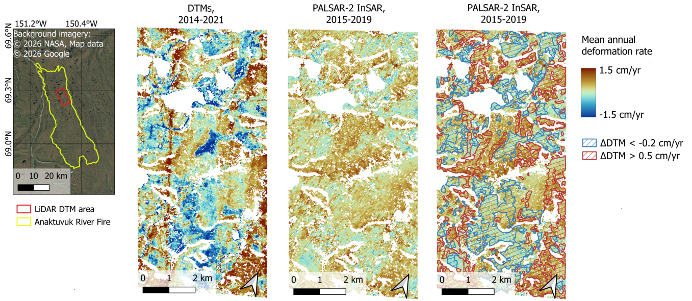
Figure 9. Comparison of annual ground -deformation rate maps derived from PALSAR-2 InSAR data (2015–2019) and downsampled LiDAR DTMs (Jones et al., 2024b) (2014–2021) for a 50 km 2 area within the Anaktuvuk River tundra fire scar (fire event 2007). The left panel shows the extent of the Anaktuvuk River fire scar and the location of the LiDAR DTM analysis area, which is displayed in the annual deformation rate maps on the right. (Background imagery of left panel: © 2026 NASA, Map data © 2026 Google Satellite)
