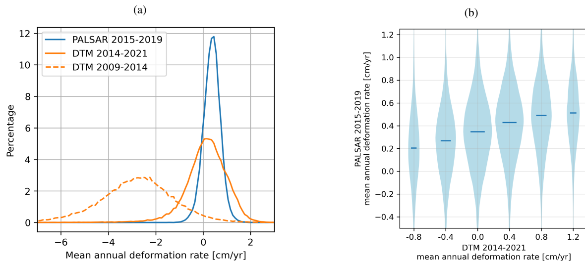
Figure 10. a) Histograms of long-term annual deformation rate from PALSAR-2 InSAR for the period 2015-2019, and annual deformation rate values derived from downsampled LiDAR DTMs (Jones et al., 2024b) for the periods 2009-2014 and 2014-2021 for a 50 km 2 area within the Anaktuvuk River tundra fire scar (fire event 2007). The histograms use a bin size of 0.1 cm/yr. b) Long-term annual Annual deformation rate from PALSAR-2 InSAR for the period 2015-2019 statistics (violin plot) by annual deformation rate bins (bin size 0.4 cm/yr) derived from downsampled LiDAR DTMs (Jones et al., 2024b) for the periods 2014-2021. Median values are shown as vertical lines; violin widths reflect the sample size.
