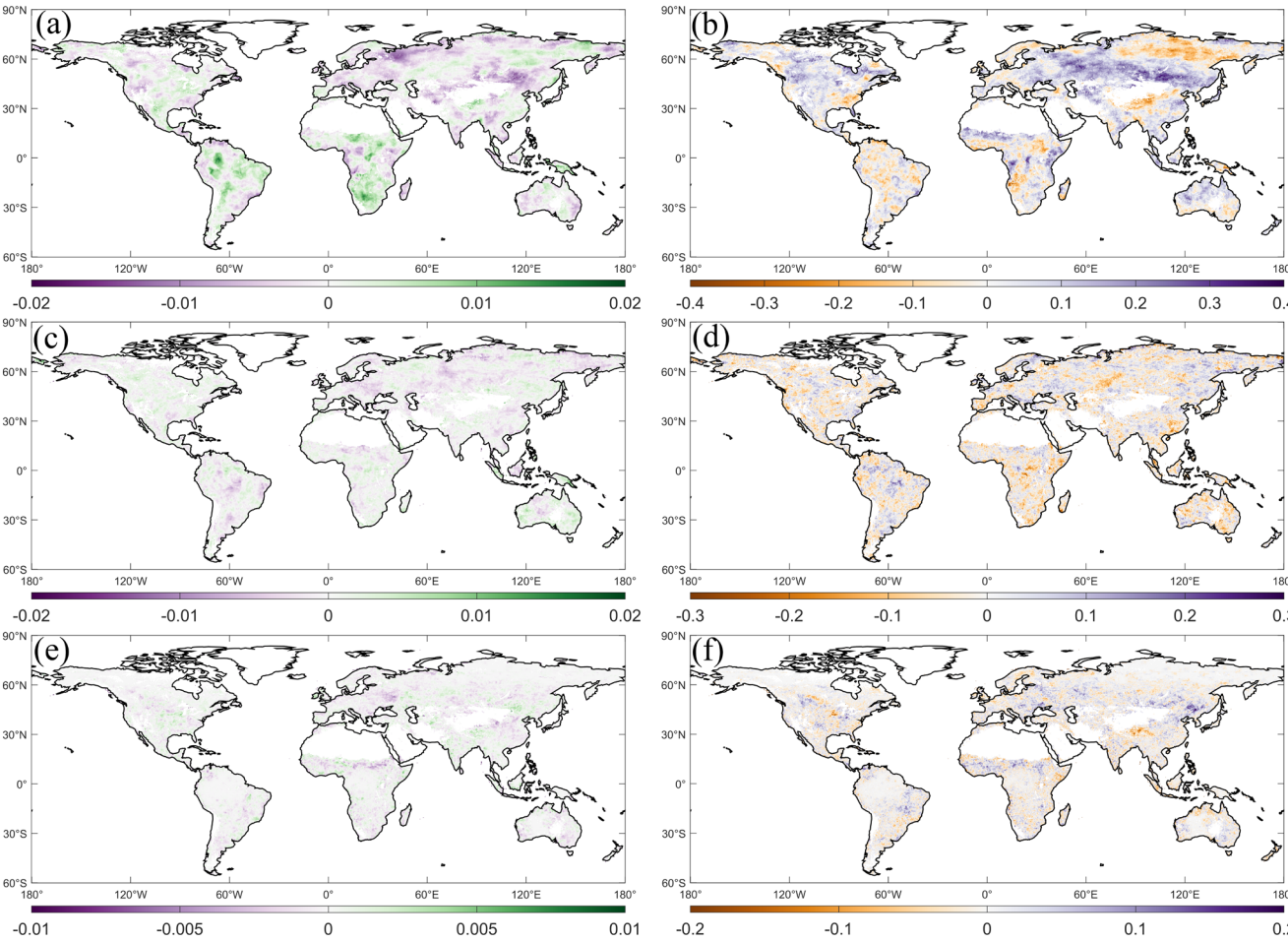
Figure 3. The contributions of CO 2 , CLI, and LCC to the R_{max} and T_{opt} under an 18-year moving window. (The left and right columns represented the contributions of variables to the R_{max} and T_{opt} , respectively, with the contributions of CO 2 , CLI, and LCC shown from top to bottom.)
