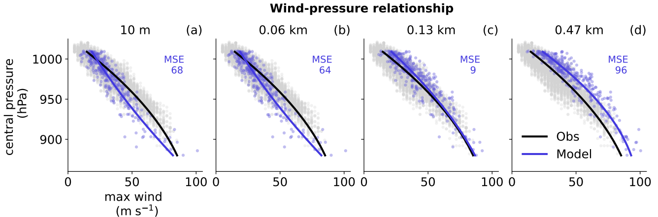
Figure 2. Wind-pressure relationship across TC life cycles for observations (black, n=12,318 ) and model (blue, n=363 ). Observed winds are at 10 m, modeled winds are selected from 10 m to 0.47 km (a-d). Curves show a quadratic fits excluding outliers. The mean squared error (MSE, in \text{m}^2 \text{s}^{-2} ) of the model fit is indicated in each panel.
