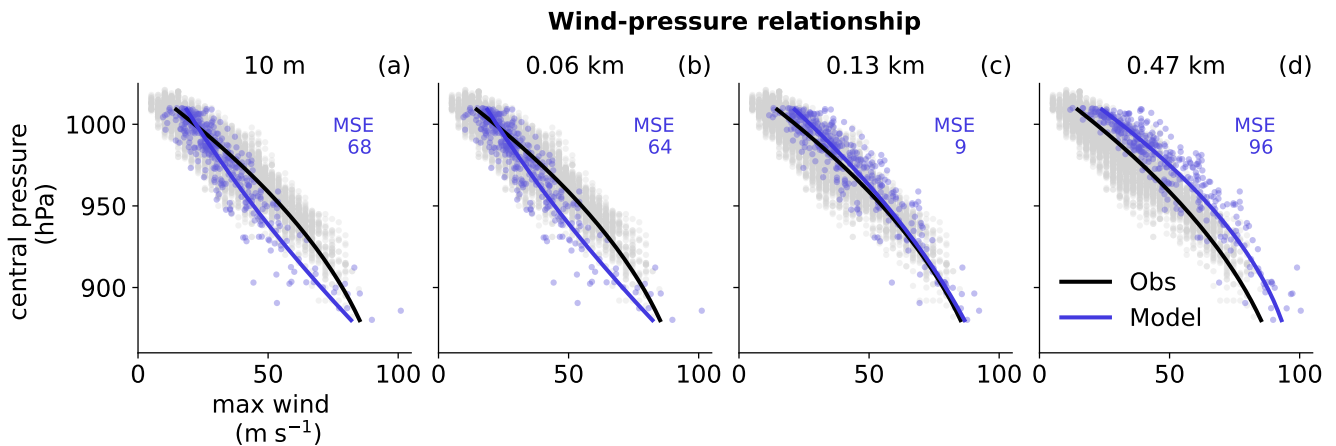
Figure 2. Wind-pressure Wind-pressure relationship across TC life cycles for observations (black, n=12,318 ) and model output (blue, n=363 ). Observed winds are at 10 m, modeled winds are selected from 10 m to 8.230.47 km (a-d). Curves show a quadratic fits excluding outliers. The mean squared error (MSE, in \text{m}^2 \text{ s}^{-2} ) of the model fit is indicated in each panel.
