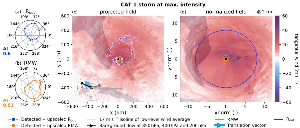
Figure 6. As Fig. 5, but for a \text{cat}_{\text{pres}} 1 storm.
