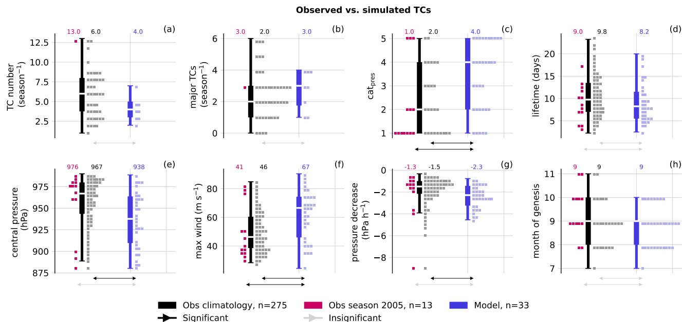
Figure 3. Comparison of observed and simulated TC activity: number of TCs per season (a), number of major hurricanes per season (cat pres 3-5, b), overall distribution of pressure based categories (c), storm lifetime (d), minimum central pressure reached (e), wind at maximum intensity (f), largest pressure decrease within intensification phase (g) and month of genesis (h). Maximum winds in (f) are taken at 10 m for observations and at 130 m for the model. Black box plots show observed climatology (HURDAT2, since 1980), blue box plots show model results. Squares indicate underlying distributions: gray for observed climatology (n = 297, 1 square = 6 TCs, rounded to an integer), red for observations of the season 2005 (n = 16, 1 square = 1 TC), and blue for the model (n = 33, 1 square = 1 TC). In (c) and (h), each square represents 12 TCs (rounded to an integer) for the climatology for better visibility. Numbers above each panel indicate the distribution medians. Arrows at the bottom denote insignificant (gray) or significant (black) deviations of the model from the observed climatology (short arrow) or from the season 2005 (long arrow) based on a two-sided permutation test at a significance level of 0.05.
