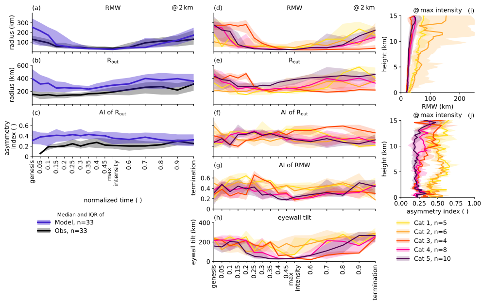
Figure 7. Evolution of TC structure related metrics over the storm’s life cycle: RMW (a, d), R_{out} (b, e), asymmetry index (AI) of R_{out} (c, f) and AI of RMW (g) and eyewall tilt (h). Panels (a-c) show a comparison of observed TC structures (HURDAT2 since 2021, black) and simulated TC structures (blue). Simulated TC wind radii and AIs are diagnosed at 2 km altitude, observations correspond to 10 m altitude. Panels (d-ij) show simulated TCs split according to their lifetime maximum intensity, hence storm intensity can differ within one category before and after reaching maximum intensity. Vertical profiles of RMW (hi) and RMW AI (ij) are displayed at maximum intensity. The eyewall tilt is estimated as the difference between the minimum and maximum of the vertical profile of RMW between 0-15 km. Lines display the group’s median and the shaded area represents the interquartile ranges (IQRs). Normalized time ticks indicate the frequency of diagnosed radii and AIs setting a focus on the intensification phase.
