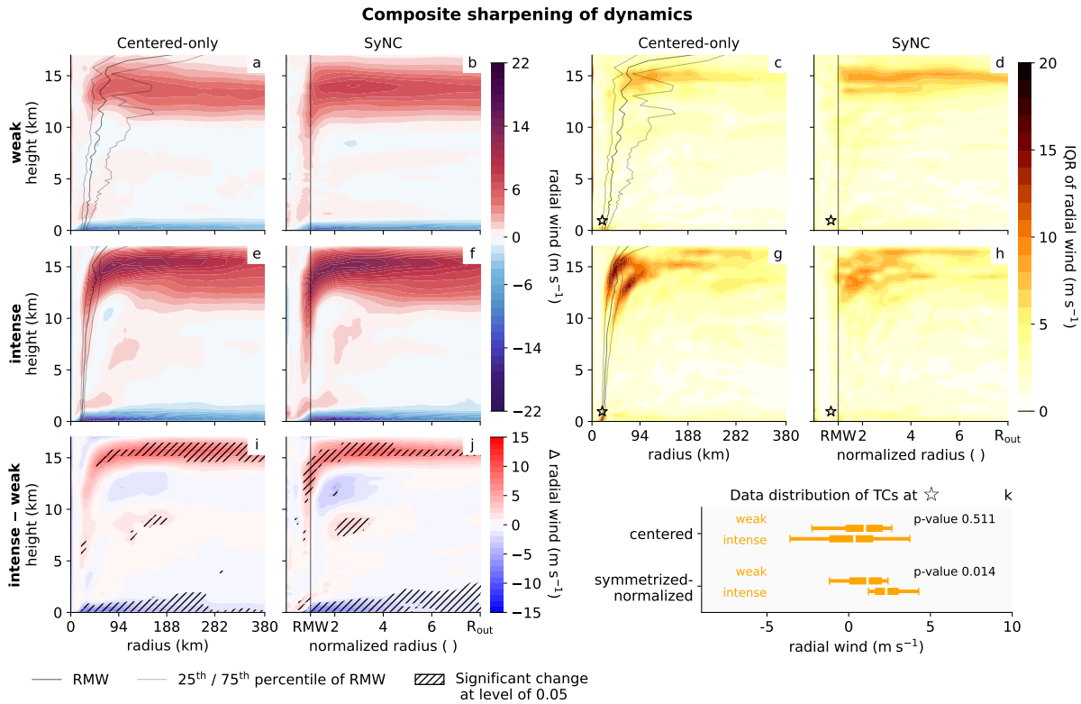
Figure 10. Composite sharpening of radial winds and its influence on statistic testing between weak and intense TC groups at lifetime maximum intensity : The centered-only composite ( a , e , i ) of weak TCs ( n=15 , a ), intense TCs ( n=18 , e ) and their difference ( i ). Panels ( b ), ( f ) and ( j ) show the same, but for the SyNC composite. Hatched areas ( i , j ) indicate statistically significant differences between the two TC groups based on a false-discovery rate corrected permutation test at a 0.05 significance level. The interquartile ranges (IQRs) of each grid cell of both composite methods are shown in ( c ), ( d ), ( g ) and ( h ): centered-only weak ( c ), centered-only intense ( g ), SyNC weak ( d ) and SyNC intense TCs ( h ). The black star highlights one selected grid cell, at which location the data distribution of the TC groups is displayed in ( k ). The p-value at the selected grid cell is indicated within the sub panel ( k ). For the centered-only cross sections, the extent of the cross sections is set to the average R_{out} detected over the intense TC group, since the mean R_{out} of the weak TC group is smaller. RMW is indicated with a black line, whereof the spread of the eyewall location is shown by the two gray lines.
