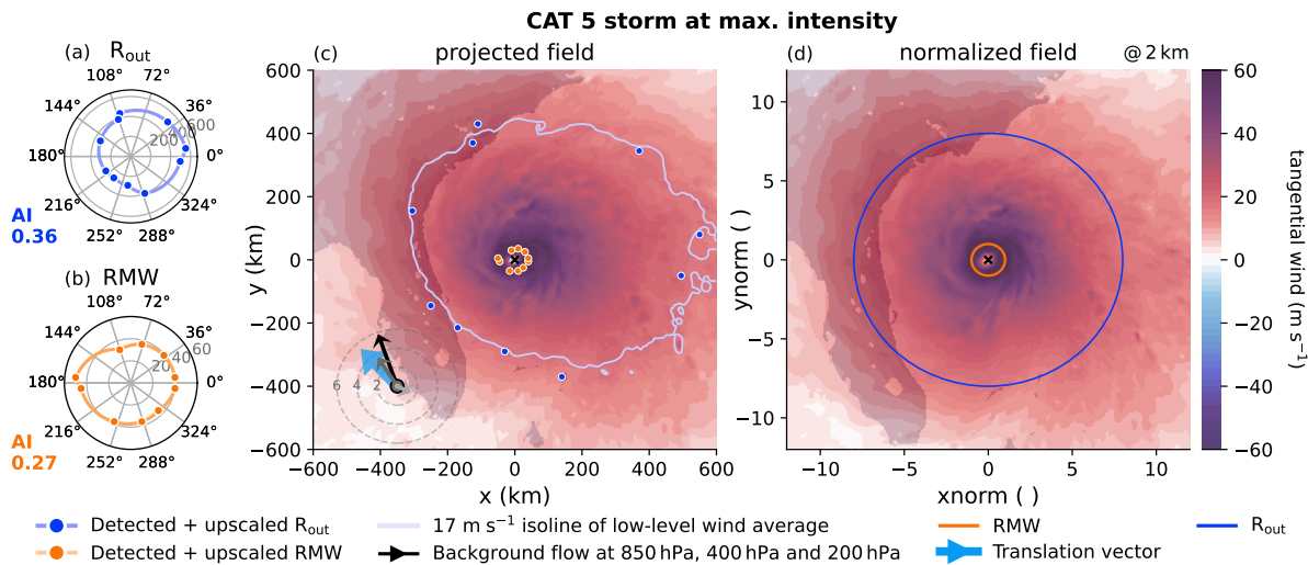
Figure 5. Demonstration of detected wind radii and the effects of SyNC of a \text{cat}_{\text{pres}} 5 storm at maximum intensity. Detected (blue points) and upscaled (blue line) R_{\text{out}} (a). Detected (orange points) and upscaled (orange line) RMW (b). The asymmetry index (AI) of R_{\text{out}} and RMW is noted in the left corner of corresponding sub panel. The vortex on the projected grid (c). The cyclone center is marked with a black cross. Contours show the tangential wind field at 2 km height with detected R_{\text{out}} (blue points) and detected RMW (orange points). The light blue line marks the 17 \text{ m s}^{-1} isoline of the low-level (0-2 km) tangential wind average used for R_{\text{out}} detection. The arrows in the lower-left corner of panel (c) indicate the background flow at 850 hPa (black), 400 hPa (gray), and 200 hPa (light gray) averaged within 600-800 km horizontal distance of the storm center, as well as the storm's translation vector (blue). Dashed circles provide magnitudes of background winds and translation speeds at levels of 2, 4 and 6 \text{m s}^{-1} . The vortex on the normalized grid (d). Contours show the tangential wind field after symmetrization and normalization, where the location of R_{\text{out}} (blue circle) and RMW (orange circle) are highlighted. Dark background shading in (c-d) denotes land.
