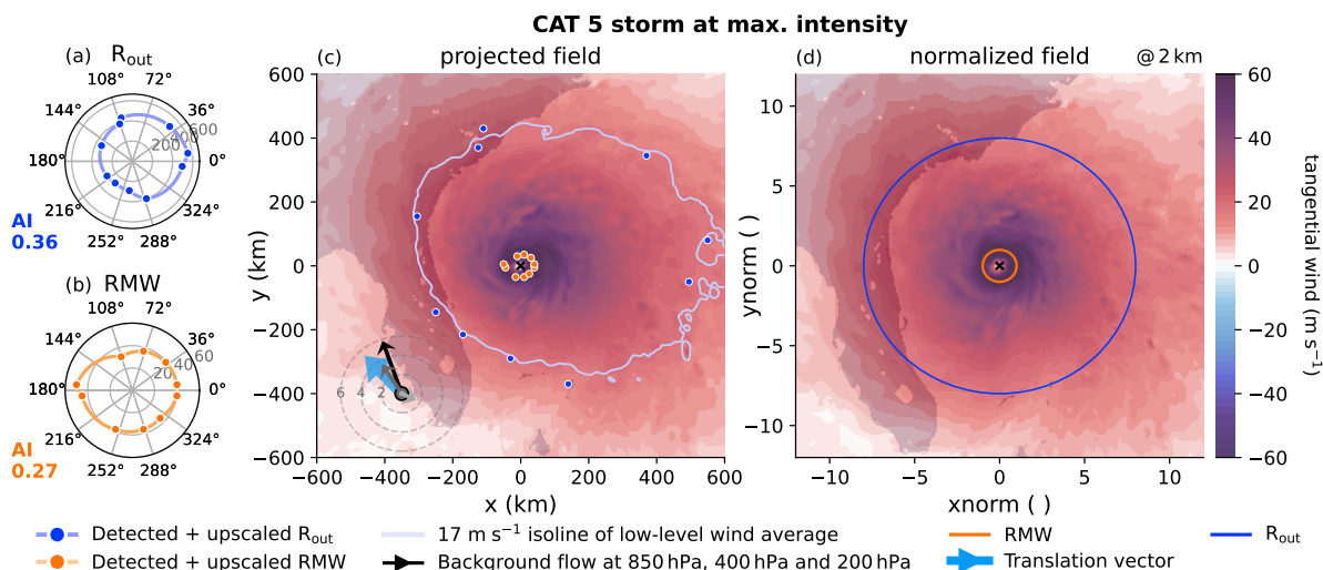
Figure 5. Demonstration of detected wind radii and the effects of SyNC of a cat pres 5 storm at maximum intensity. Detected (blue points) and upscaled (blue line) R_{out} (a). Detected (orange points) and upscaled (orange line) RMW (b). The asymmetry index (AI) of R_{out} and RMW is noted in the left corner of corresponding sub panel. The vortex on the projected grid (c). The cyclone center is marked with a black cross. Contours show the tangential wind field at 2 km height with detected R_{out} (blue points) and detected RMW (orange points). The light blue line marks the 17 m s^{-1} isoline of the low-level (0-2 km) tangential wind average used for R_{out} detection. The arrows in the lower-left corner of panel (c) indicate the background flow at 850 hPa (black), 400 hPa (gray), and 200 hPa (light gray) averaged within 600-800 km horizontal distance of the storm center, as well as the storm's translation vector (blue). Dashed circles provide magnitudes of background winds and translation speeds at levels of 2, 4 and 6 m s^{-1} . The vortex on the normalized grid (d). Contours show the tangential wind field after symmetrization and normalization, where the location of R_{out} (blue circle) and RMW (orange circle) are highlighted. Dark background shading in (c-d) denotes land.
