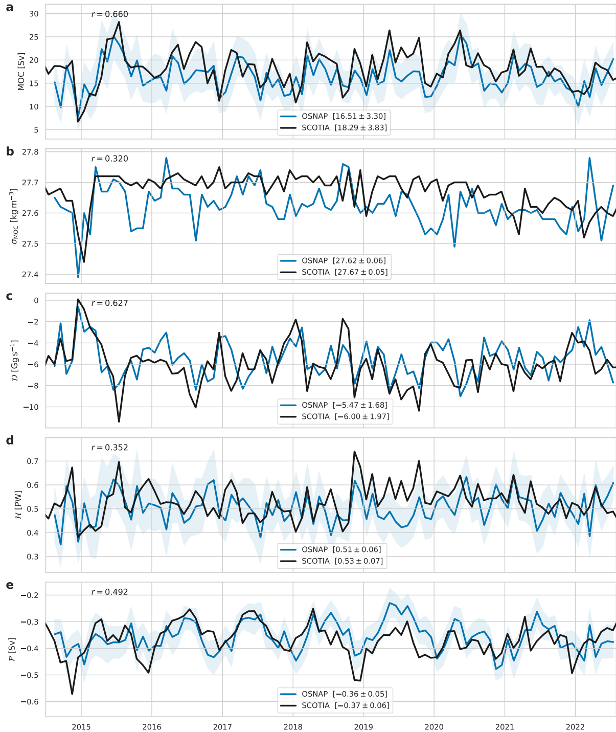
Figure 4. Time series of (a) MOC, (b) \sigma_{\text{MOC}} , (c) northward density flux \mathcal{D} , (d) northward heat flux \mathcal{H} , and (e) northward freshwater flux \mathcal{F} from SCOTIA (black) and OSNAP (blue) for the period covered by the available OSNAP data (2014 to 2022). The mean and standard deviation of each time series are shown in square brackets. Correlation coefficients r are all significant at the 95% confidence level. Blue shading represents the uncertainties provided with the OSNAP data product.
