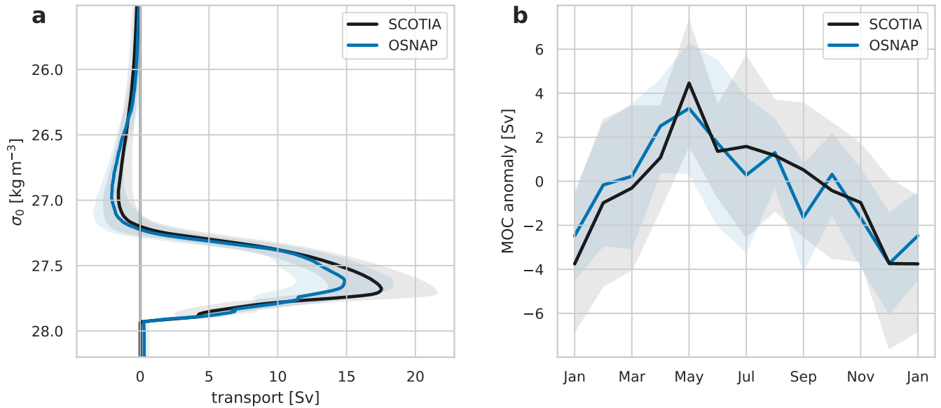
Figure 3. (a) Mean overturning streamfunctions [Sv] in density space for SCOTIA (black line) and OSNAP (blue line). Shaded areas show the standard deviation of the streamfunction. (b) The seasonal cycle of overturning anomalies for SCOTIA (black line) and OSNAP (blue line). Lines show the mean anomaly for each calendar month, shaded areas the standard deviation. The means and seasonal cycle have been calculated for the period spanned by the available OSNAP data (2014 to 2022), but the SCOTIA results are not qualitatively different when considering the full period (2004 to 2024).
