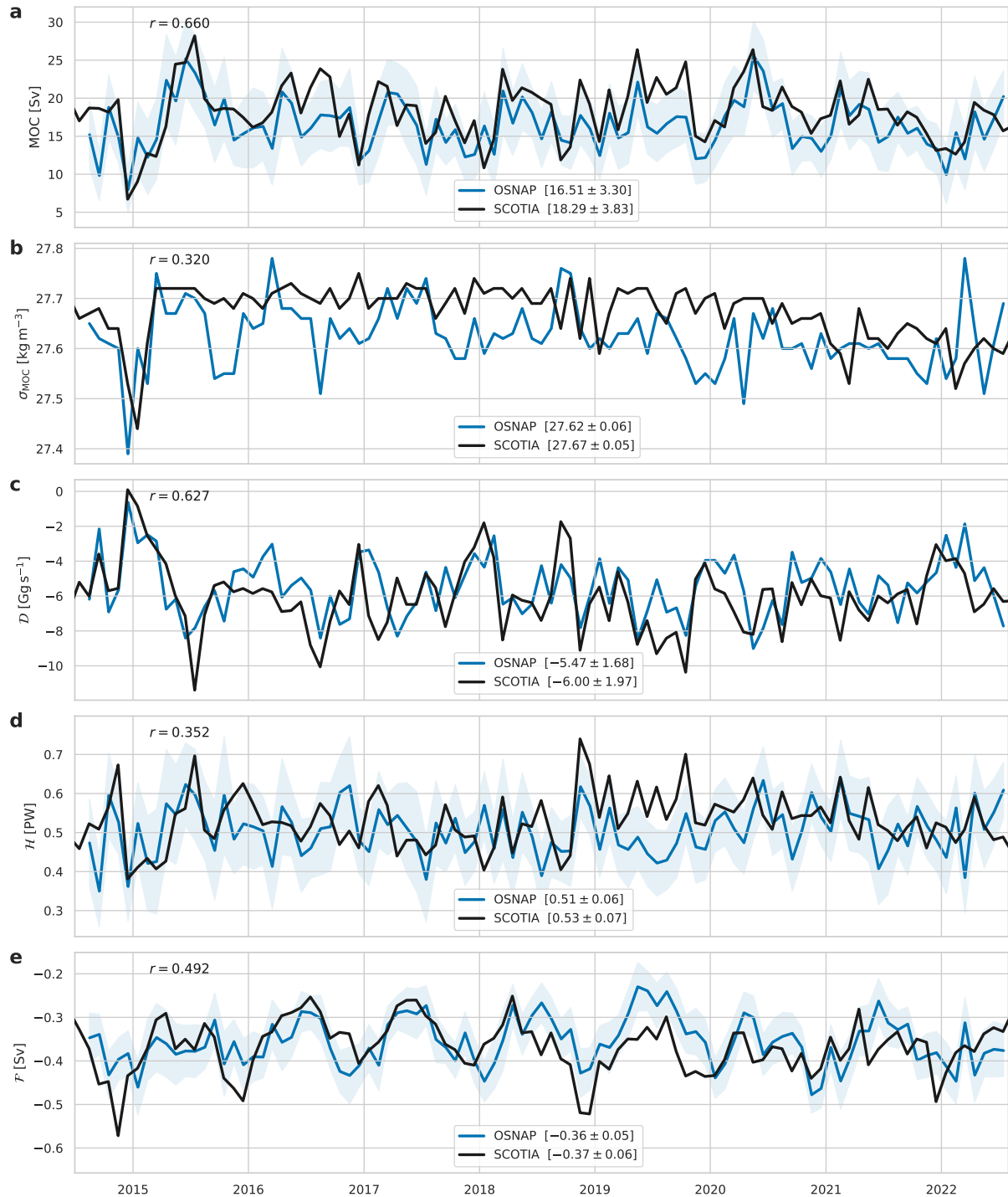
Figure 4. Timeseries Time series of overturning and transports from SCOTIA and OSNAP for the period covered by the available OSNAP data (2014 to 2022). Black lines—SCOTIA, blue lines—OSNAP. Panel (a) MOC, (b) \sigma_{MOC} , (c) northward density flux \mathcal{D} , (d) northward heat flux \mathcal{H} , and (e) northward freshwater flux \mathcal{F} from SCOTIA (black) and OSNAP (blue) for the period covered by the available OSNAP data (2014 to 2022). The mean and standard deviation of each time series are shown in square brackets. Correlation coefficients r are all significant at the 95% confidence level. Blue shading represents the uncertainties provided with the OSNAP data product.
