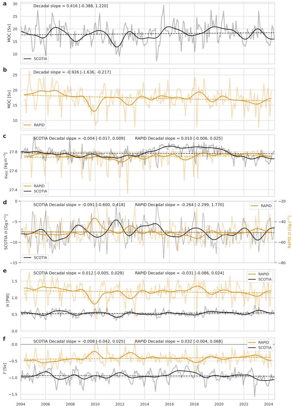
Figure 5. Timeseries-Time series of overturning and transports from SCOTIA and RAPID for the 20 year period 2004 to 2024). Black lines – SCOTIA, amber lines – RAPID. In each case the paler solid lines are the monthly values, darker solid lines the 18 month low-pass filtered timeseries , and the dashed lines show the trend. The trend and the 95% confidence limits on the trend (in square brackets) are given in each panel. Panel (a) SCOTIA MOC, (b) RAPID MOC, (c) \gamma_{MOC} , (d) northward density flux \mathcal{D} , (e) northward heat flux \mathcal{H} , and (f) northward freshwater flux \mathcal{F} . In panel (d) the density fluxes have been scaled for easier comparison.
