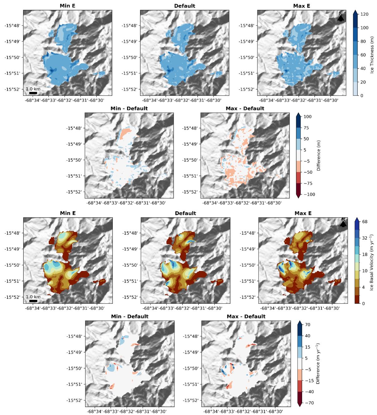
Figure S7: Thickness and velocity outputs, and subsequent difference between minimum and maximum E values with the default value within the Kaka & Boopi (#3) domain (Ancohumá Ice Caps).
