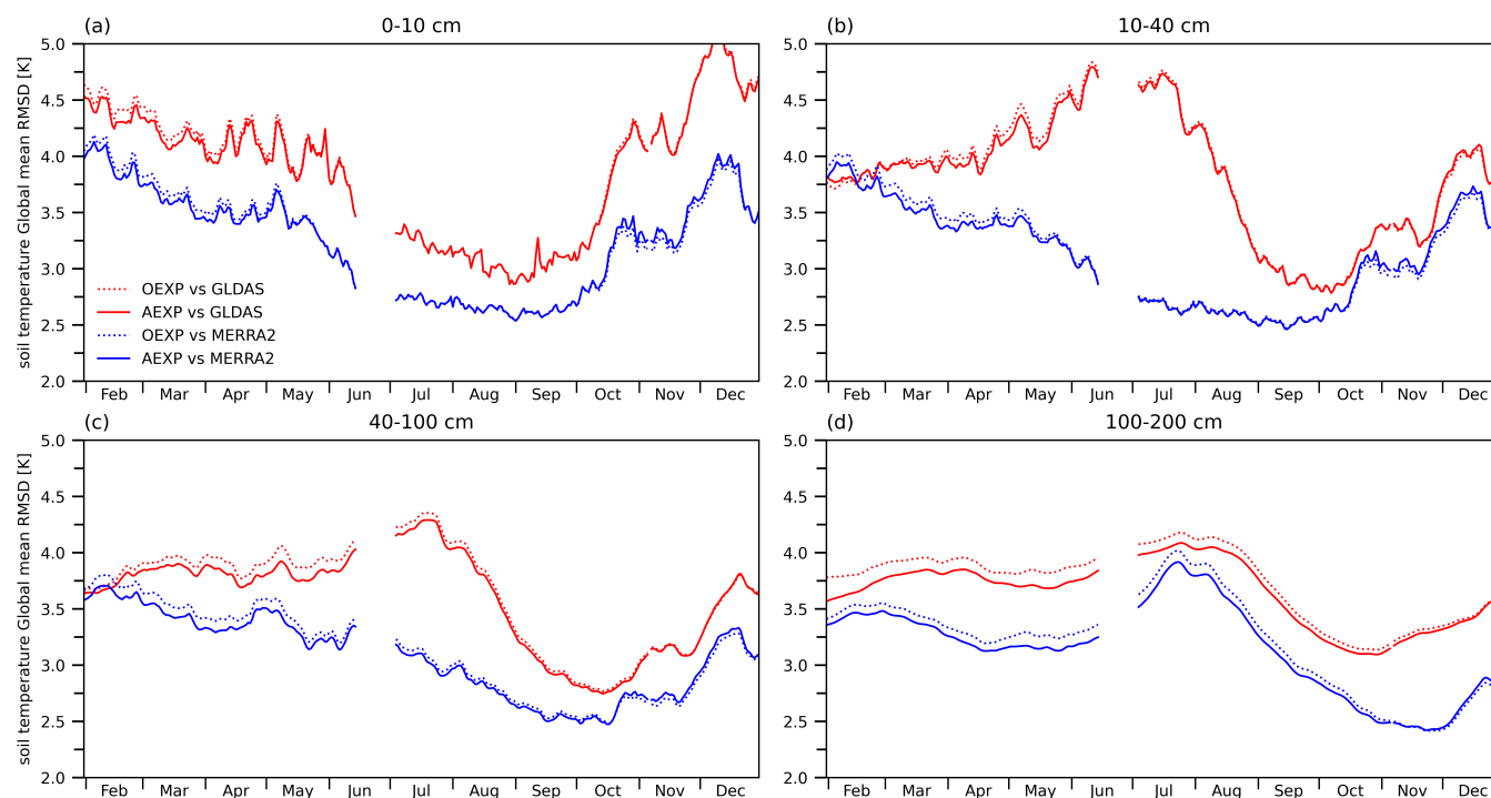
Figure 3. Soil temperature (in K) global RMSD of OEXP (dotted line) and AEXP (solid line) based on GLDAS (red) and MERRA2 (blue): (a) for 0-10 cm, (b) for 10-40 cm, (c) for 40-100 cm, and (d) for 100-200 cm.
