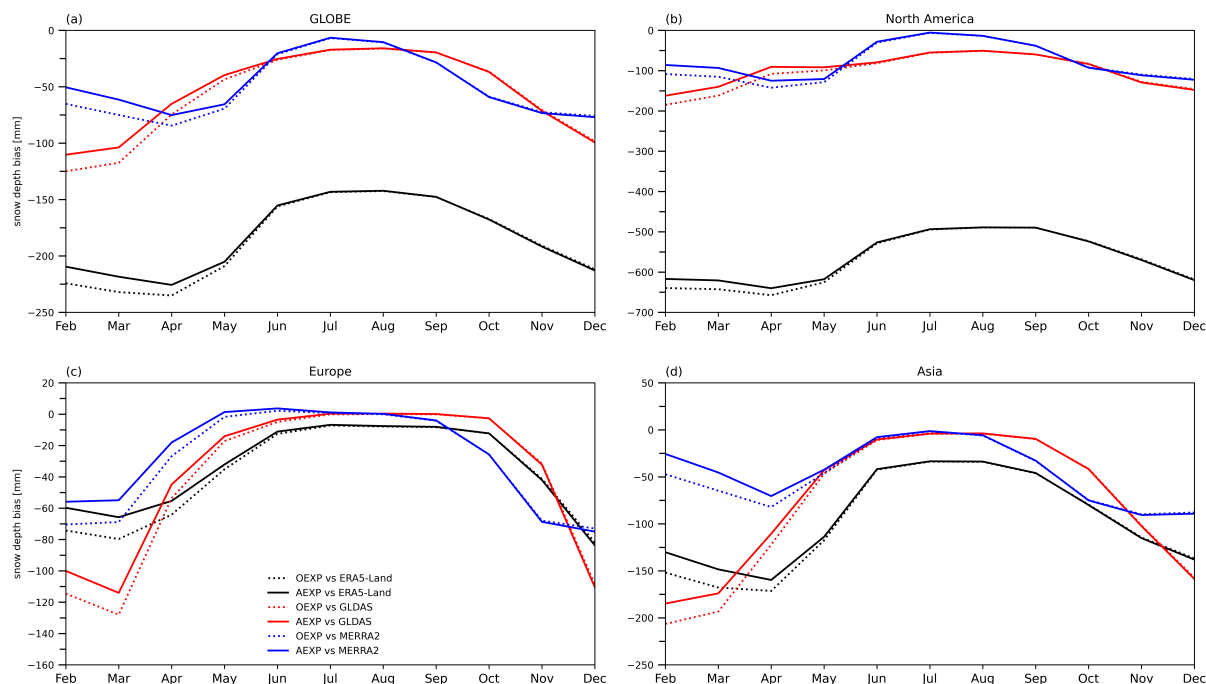
Figure 6. Snow depth (in mm) BIAS of OEXP (dotted) and AEXP (solid) based on ERA5-Land (black), GLDAS (red) and MERRA2 (blue). (a) for global excluding Antarctica, (b) for North America, (c) for Europe, and (d) for Asia.
