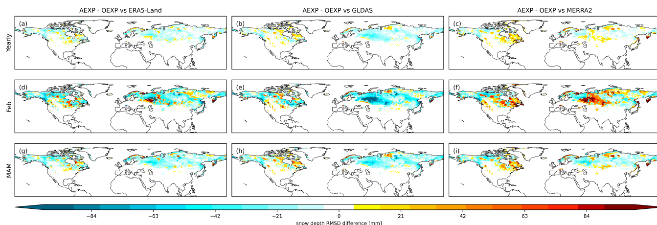
Figure 7. Snow depth (in mm) RMSD_d based on ERA5-Land (first column), GLDAS (second column), and MERRA2 (third column). (a-c) for year, (d-f) for February and (g-i) for MAM.
