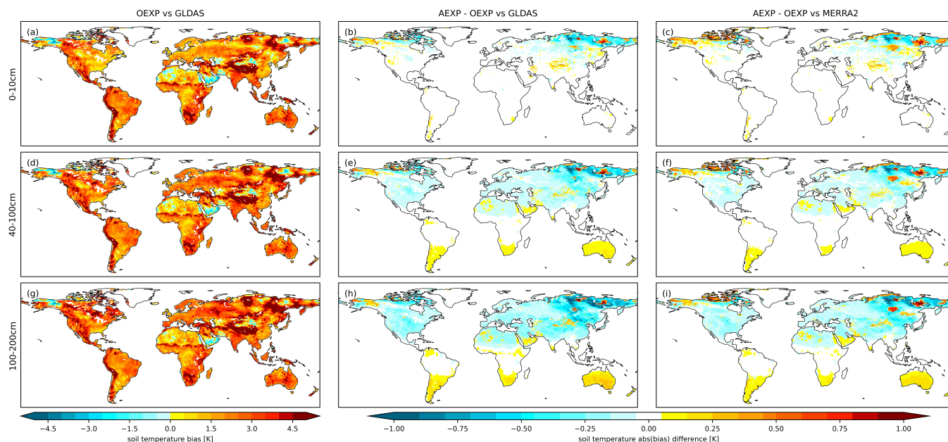
Figure 2. Soil temperature (in K) yearly (31 January 2001 to 31 December 2001) BIAS based on GLDAS of OEXP (first column) and BIAS d based on GLDAS (second column) and MERRA2 (third column): (a-c) for 0-10 cm, (d-f) for 40-100 cm, and (g-i) for 100-200 cm.
