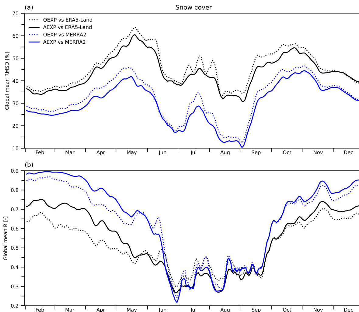
Figure 5. Snow cover (in %) global RMSD (a) and R (b) of OEXP (dotted) and AEXP (solid) based on ERA5-Land (black) and MERRA2 (blue).
