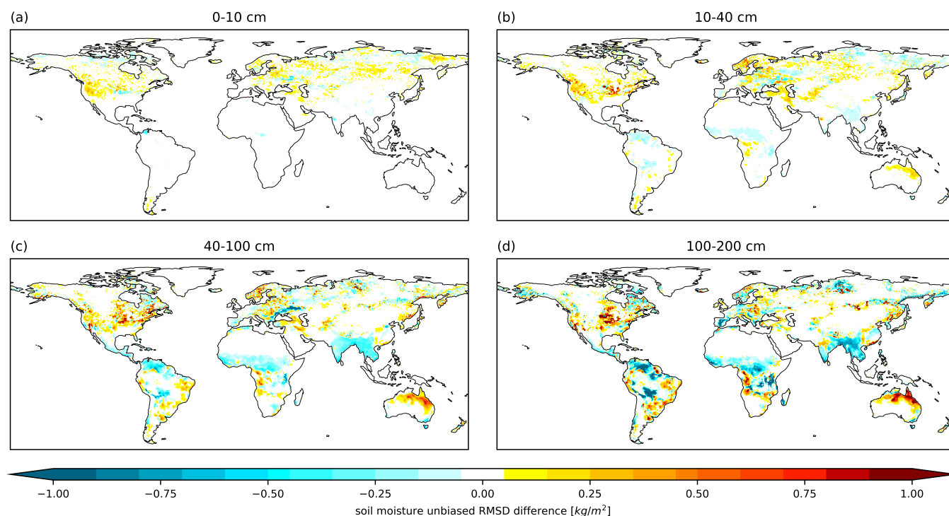
Figure 9. Soil moisture ( \text{kg/m}^2 ) yearly (from 31 January 2001 to 31 December 2001) (unbiased RMSD) d based on GLDAS: (a) for 0-10 cm, (b) for 10-40 cm, (c) for 40-100 cm and (d) for 100-200 cm.
