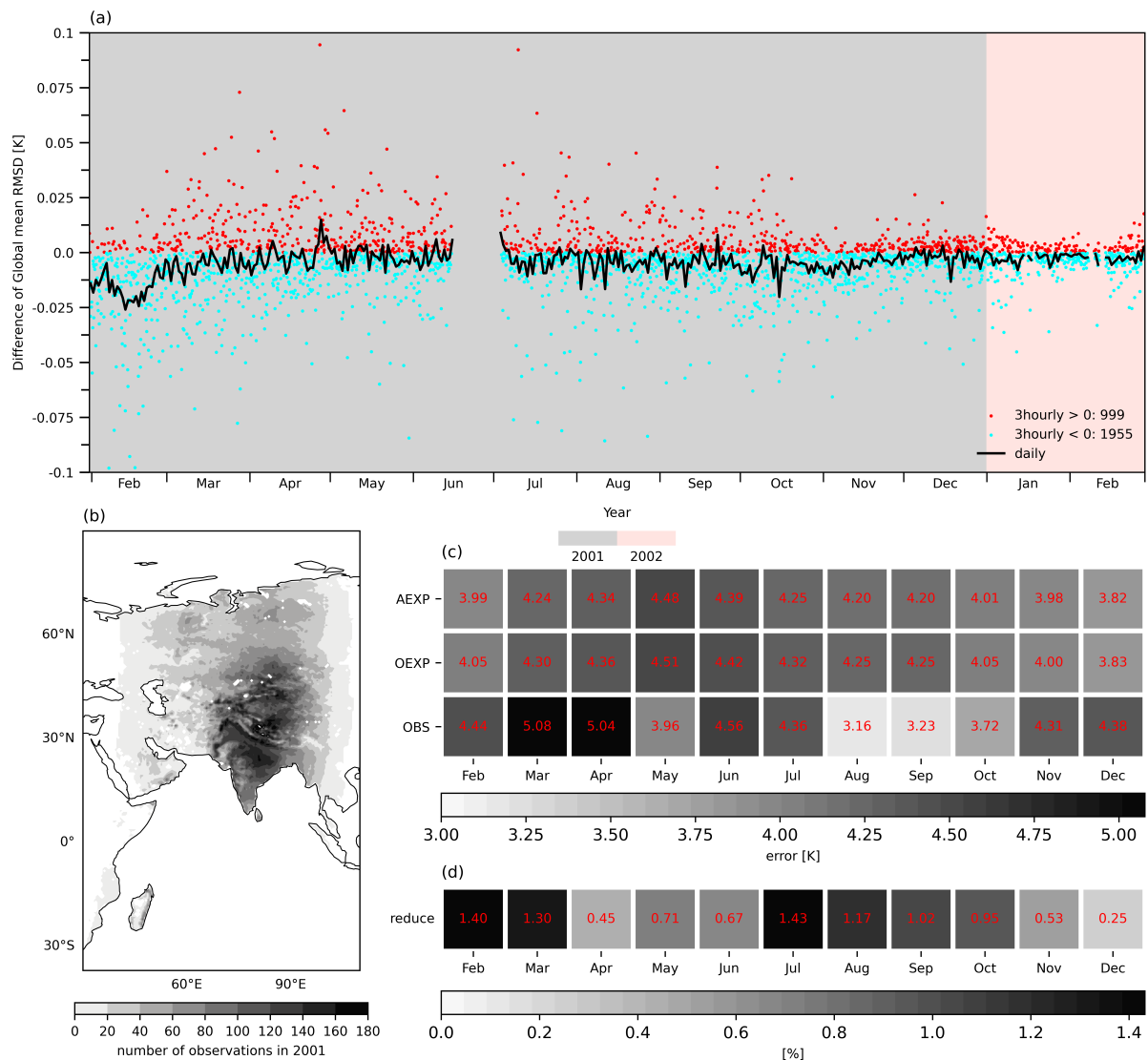
Figure 1. (a) Global LST RMSD d based on the MODIS-LST from 31 January 2001 to 28 February 2002 in 3-hour intervals (red and cyan dots for positive and negative values, respectively) and daily mean (solid black line), as the observations are not available in some days between June and July (blank areas). The number of positive and negative values is shown in the legend. Gray and pink backgrounds represent the period of cycle DA and free forecast, respectively. (b) number of observations centered at 6 UTC within the time window from 1 Jan 2001 – 31 Dec 2001. (c) Eastern Hemisphere (EH) monthly mean spatially averaged error for observations (third row) and the LST RMSD for AEXP (first row) and OEXP (second row) based on the MODIS-LST, and (d) relative reduction in percent of LST RMSD from OEXP to AEXP.
