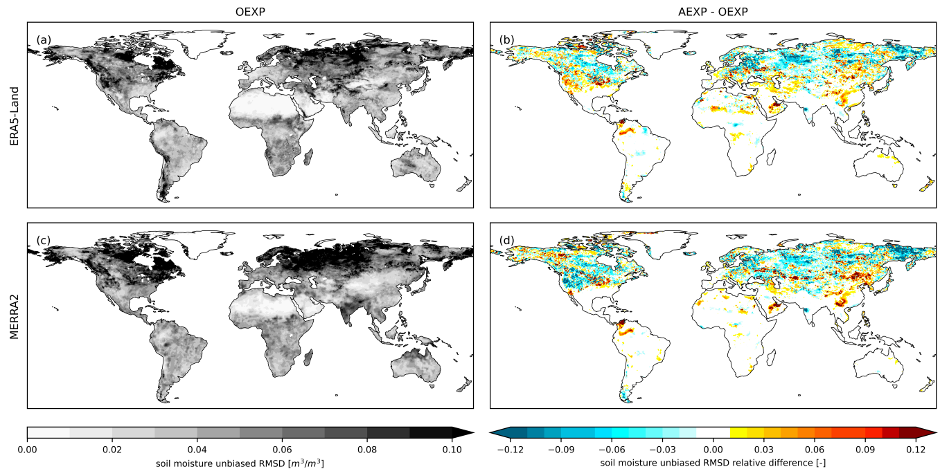
Figure 8. Soil moisture (in m^3/m^3 ) yearly (31 January 2001 to 31 December 2001) unbiased RMSD of OEXP (first column) and relative (unbiased RMSD) d (second column) in the upper soil layer based on (a-b) ERA5-Land and (c-d) MERRA2.
