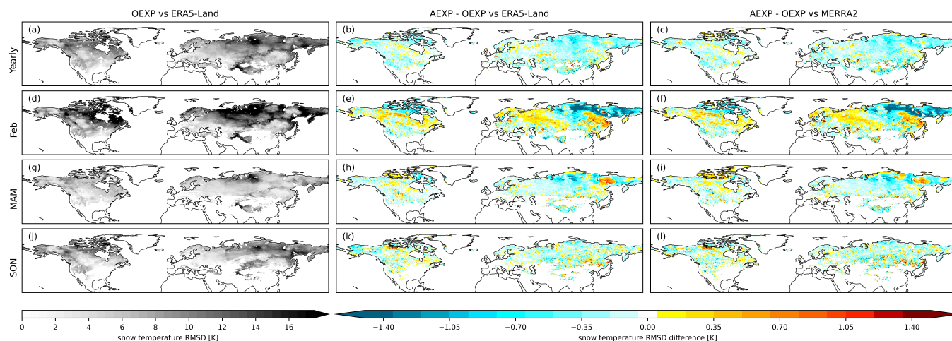
Figure 4. Snow temperature (in K) RMSD based on ERA5-Land (first column) of OEXP and \text{RMSD}_d based on ERA5-Land (second column) and MERRA2 (third column) for (a-c) yearly, (d-f) February, (g-i) MAM, and (j-l) SON.
