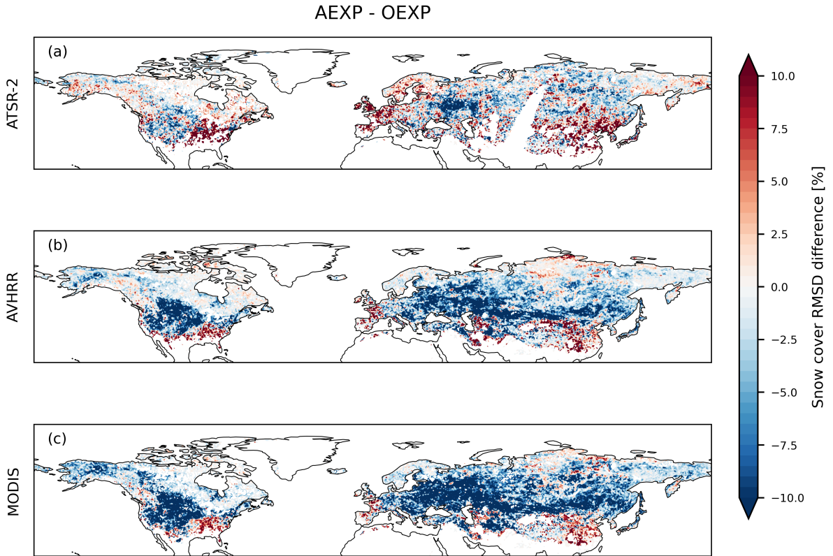
Figure 8. Snow cover [%] yearly (31 January 2001 to 31 December 2001) RMSD_d evaluated based on different satellite products: (a) ATSR-2, (b) AVHRR, and (c) MODIS.
