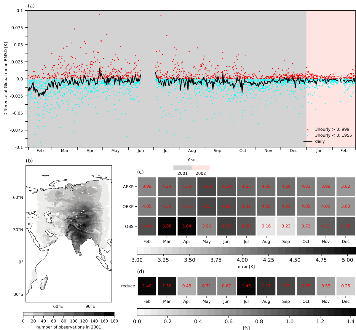
Figure 3. (a) Global LST RMSD d based on the MODIS-LST from 31 January 2001 to 28 February 2002 in 3-hour intervals (red and cyan dots for positive and negative values, respectively) and daily mean (solid black line), as the observations are not available in some days between June and July (blank areas). The number of positive and negative values is shown in the legend. Gray and pink backgrounds represent the period of cycle DA and free forecast, respectively. (b) number of observations centered at 6 UTC within the time window from 1 Jan 2001 – 31 Dec 2001. (c) Eastern Hemisphere monthly mean spatially averaged error for observations (third row) and the LST RMSD for AEXP (first row) and OEXP (second row) based on the MODIS-LST, and (d) relative reduction in percent of LST RMSD from OEXP to AEXP.
