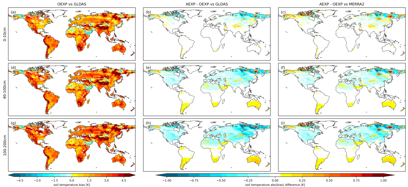
Figure 4. Soil temperature (in K) yearly (31 January 2001 to 31 December 2001) BIAS based on GLDAS of OEXP (first column) and \text{BIAS}_d based on GLDAS (second column) and MERRA2 (third column): (a-c) for 0-10 cm, (d-f) for 40-100 cm, and (g-i) for 100-200 cm.
