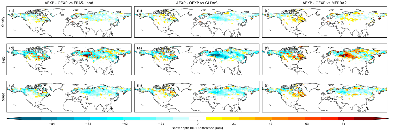
Figure 10. Snow depth (in mm) RMSD d based on ERA5-Land (first column), GLDAS (second column), and MERRA2 (third column). (a-c) for year, (d-f) for February and (g-i) for MAM (March-April-May).
