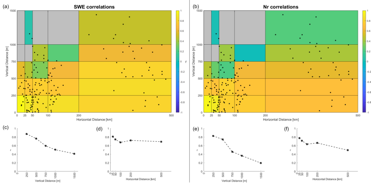
Figure 3: Heatmap of the average correlations of the SWE CRNS (a) and N r (b) time series classified by the horizontal (x-axis) and vertical (y-axis) distances between unmonitored and monitored stations. The black dots represent each pair of monitored-
