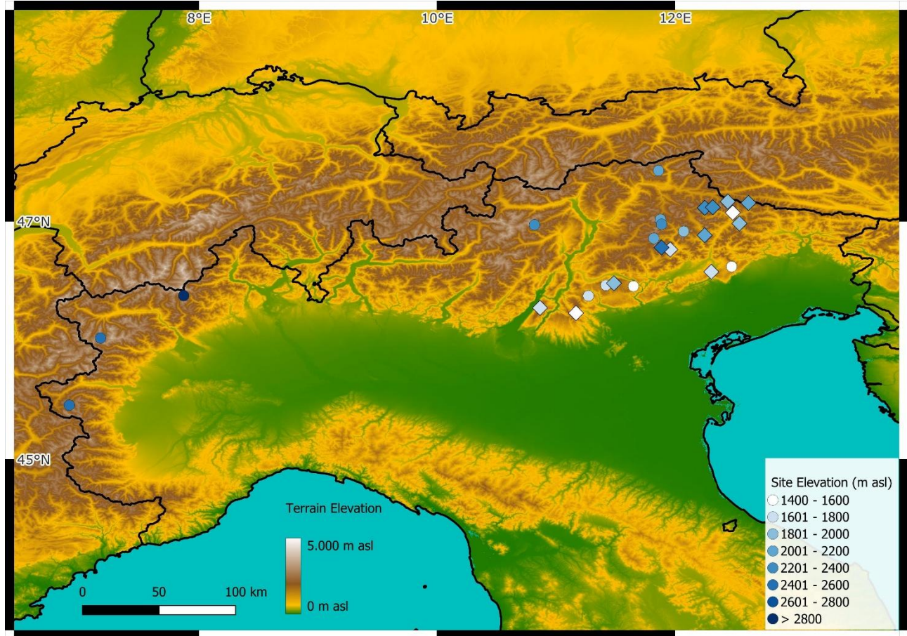
Figure 1: Elevation map of the Alps and northern Italy. Monitored and unmonitored Sites of the network are indicated by circles and diamonds respectively ; circles correspond to locations where manual SWE samples are available (i.e. monitored sites), while diamonds are used for location without available manual SWE samples (i.e. unmonitored sites); the symbols filling follows a scale of blue to represent the elevation of each site, where darker shades correspond to higher elevations. Produced using Copernicus WorldDEM-90 © DLR e.V. 2010-2014 and © Airbus Defence and Space GmbH 2014-2018 provided under COPERNICUS by the European Union and ESA; all rights reserved.
