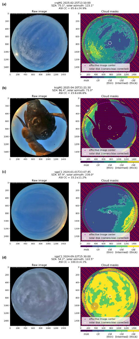
Figure 3: ASISKYCOVER pixel segmentation algorithm output for selected scenes. (left) Raw ASI image (Note that the ASI images appear mirrored in the east-west direction; see Section 2.1 for details), (right) algorithm output. The resolved classes are given in the legend at the bottom of the classification masks. In each classification mask, the red ‘+’ denotes the determined image center, the dashed magenta and white circles designate the image areas covering up to 80° and 5° off-zenith, respectively, the white star marker indicates the corrected position of the solar disk, dotted white hatched areas denote uncertain classification pixels, and the dotted magenta hatched areas mark masked pixels (site mask + solar disk mask). The ASI image site, facility and time, as well as the corresponding SZA, azimuth angle, and algorithm-resolved cloud cover (following section 2.3) are given in the title of each image pair.
