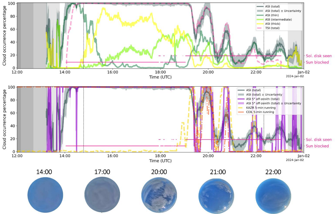
380 Figure 6: ASISKYCOVER cloud cover time series for the SGP central facility on January 1, 2024. (Top) total cloud cover time series using the full 80° off-zenith field-of-view together with time series for the three cloud classes (see legend). The light pink curve illustrates the TSI sky cover time series. The pink markers denote the solar disk state classification output (see right y-axis labels). The grey-shaded regions extending until nearly 14:00 UTC and from roughly 23:00 UTC designate (in decreasing brightness) the civil twilight, nautical twilight, astronomical twilight, and nighttime. The vertical dotted black lines denote 80° SZA crosspoints. 385 (Bottom) Similar, but showing the near-zenith (5° off-zenith) product time series together with the 5-min running mean Ka-band ARM Zenith Radar (KAZR; using moderate sensitivity mode echoes above 4 km range) and ceilometer cloud occurrence (see legend). A selected set of raw ASI images are shown at the bottom of the figure together with their corresponding times. (Note that the ASI images appear mirrored in the east-west direction; see Section 2.1 for details).
