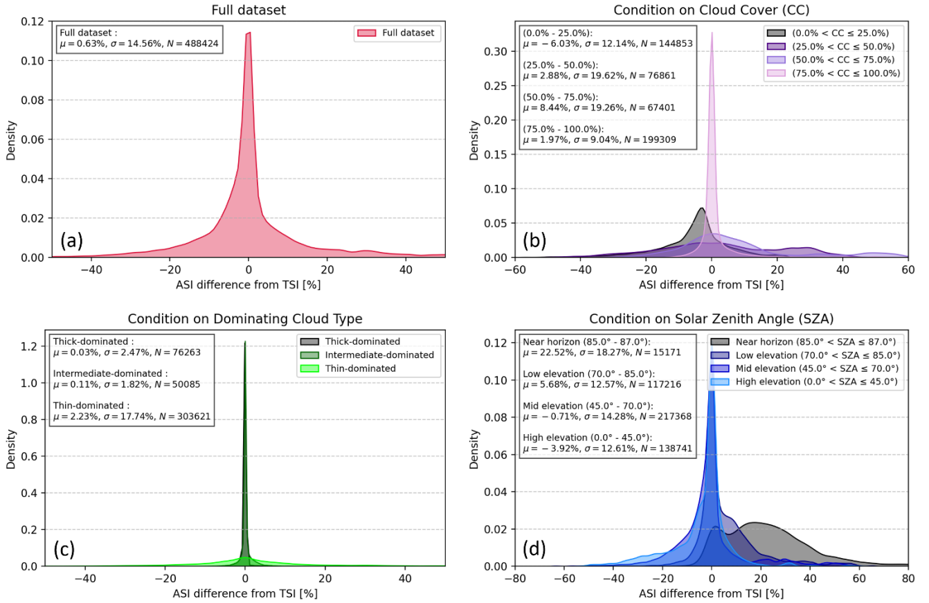
Figure 8: ASISKYCOVER deviations from the TSI cloud cover product kernel density estimations (KDEs) for SGP in 2024 while conditioning on different variables: (a) Full dataset (no conditioning), (b) ASISKYCOVER cloud cover (CC), (c) dominating cloud type per scene with CC greater than 5% based on ASISKYCOVER, and (d) SZA (see legend). Mean deviation ( \mu ), standard deviation ( \sigma ), and number of TSI-ASISKYCOVER sample pairs in the conditioned data subset ( N ) are given on the top left of each panel.
