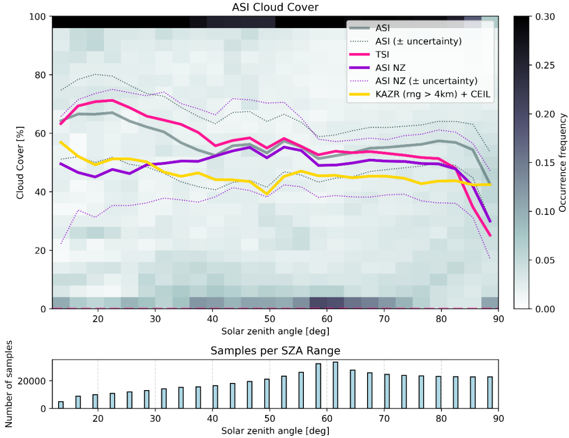
Figure 9: (Top) ASISKYCOVER-determined cloud cover occurrence frequency histogram as a function of SZA (bin sizes of 4° and 3°, respectively) normalized for each SZA bin (i.e., each column of histogram bins sums to 1) for SGP in 2024. The mean cloud cover as a function of SZA is illustrated by the grey curve, with the dotted grey curves designating the mean \pm sample uncertainties. The pink and yellow curves designate the mean cloud cover as a function of SZA for the TSI and the 5-minute running average combination of ceilometer cloud base detections and KAZR moderate sensitivity (MD) mode echoes above 4 km, respectively (see Section 3.1). The purple solid and dotted curves represent the 5-minute running average mean and mean \pm sample uncertainty cloud cover as a function of SZA determined using the ASISKYCOVER near-zenith product (NZ; see text), rendering a more equivalent comparison to the KAZR-CEIL data. (Bottom) The total number of samples (images) per SZA bin range.
