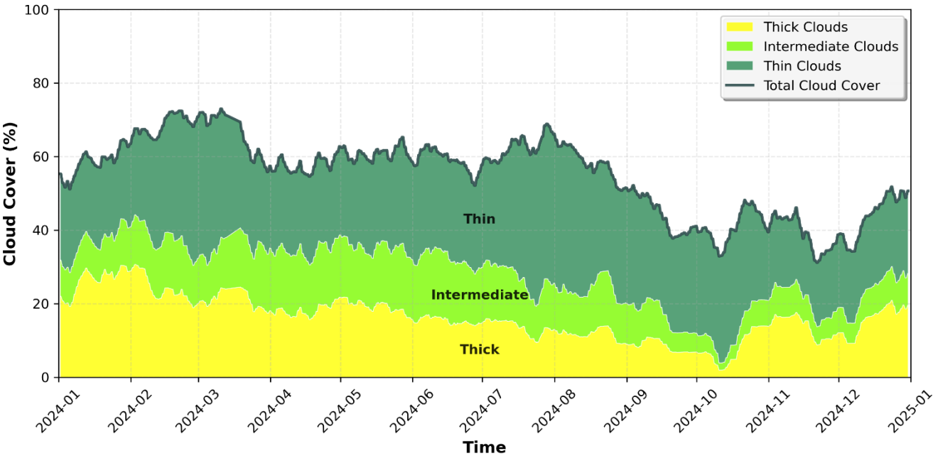
395 Figure 7: Cloud cover 31-day running-mean time series for the SGP site as determined by ASISKYCOVER for 2024. The stacked colored areas represent the distribution of cloud types (see legend and labels).
