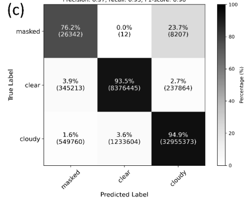
Figure 4: Confusion matrices of the segmentation algorithm output against the testing dataset. (a) Using all segmentation algorithm classes; (b) merging all cloudy classes to focus on cloudy-clear separation; and (c) same, but excluding testing samples with SZA exceeding 80°. The weighted precision, recall, and F1-score metrics for each testing subset are given in panel titles.
