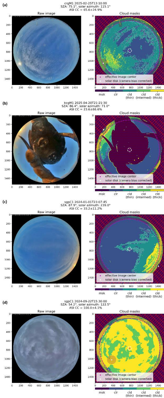
190 Figure 3: ASISKYCOVER pixel segmentation algorithm output for selected scenes. (left) Raw ASI image (Note that the ASI images appear mirrored in the east-west direction; see Section 2.1 for details), (right) algorithm output. The resolved classes are given in the legend at the bottom of the classification masks. In each classification mask, the red ‘+’ denotes the determined image center, the dashed magenta and white circles designate the image areas covering up to 80° and 5° off-zenith, respectively, the white star marker indicates the corrected position of the solar disk, dotted white hatched areas denote uncertain classification pixels, and the 195 dotted magenta hatched areas mark masked pixels (site mask + solar disk mask). The ASI image site, facility and time, as well as the corresponding SZA, azimuth angle, and algorithm-resolved cloud cover (following section 2.3) are given in the title of each image pair.
