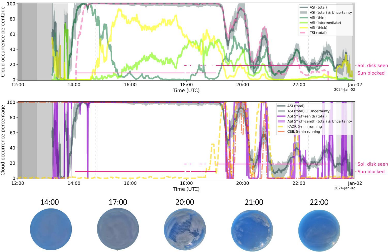
Figure 6: ASISKYCOVER cloud cover time series for the SGP central facility on January 1, 2024. (Top) total cloud cover time series using the full 80° off-zenith field-of-view together with time series for the three cloud classes (see legend). The light pink curve illustrates the TSI sky cover time series. The pink markers denote the solar disk state classification output (see right y-axis labels). The Grey-shaded regions extending until nearly 14:00 UTC and from roughly 23:00 UTC designate (in decreasing brightness) the civil twilight, nautical twilight, astronomical twilight, and nighttime. The vertical dotted black lines denote 80° SZA crosspoints. (Bottom) Similar, but showing the near-zenith (5° off-zenith) product time series together with the 5-min running mean Ka-band ARM Zenith Radar (KAZR; using moderate sensitivity mode echoes above 4 km range) and ceilometer cloud occurrence (see legend). A selected set of raw ASI images are shown at the bottom of the figure together with their corresponding times. (Note that the ASI images appear mirrored in the east-west direction; see Section 2.1 for details).
