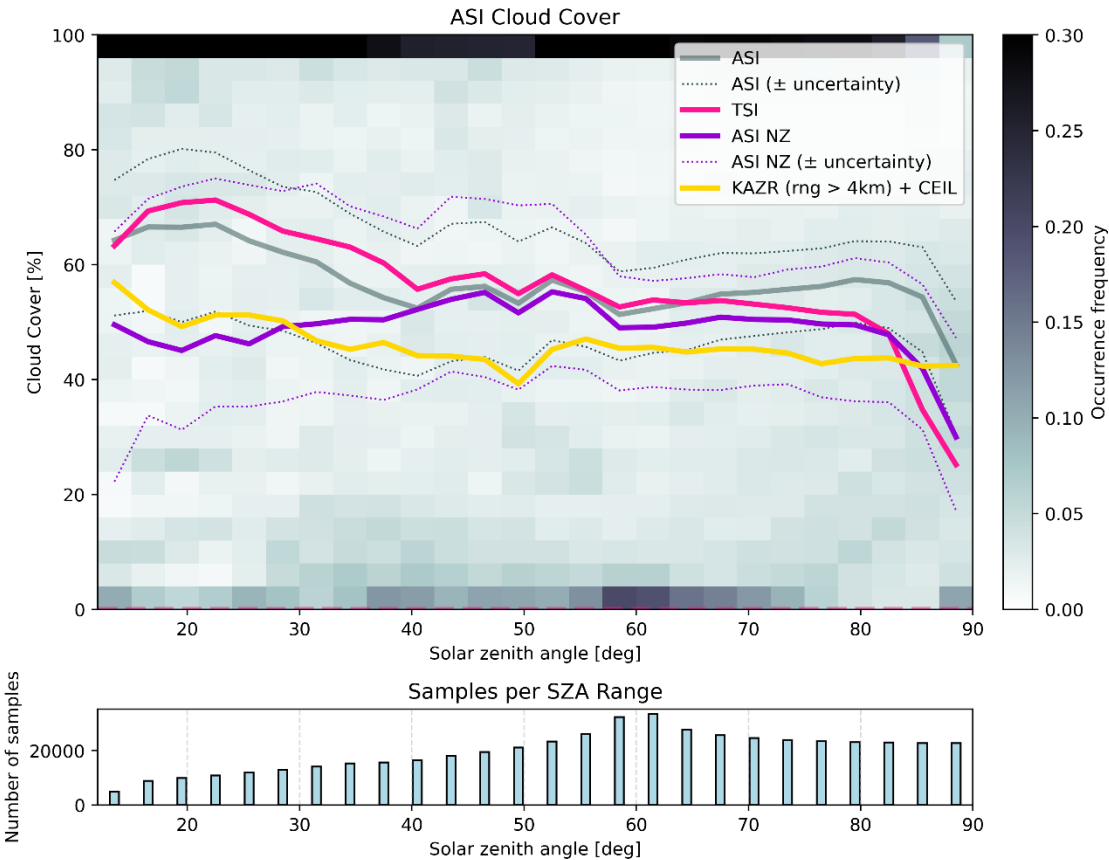
490 Figure 9: (Top) ASISKYCOVER-determined cloud cover occurrence frequency histogram as a function of SZA (bin sizes of 4% and 3°, respectively) normalized for each SZA bin (i.e., each column of histogram bins sums to 1) for SGP in 2024. The mean cloud cover as a function of SZA is illustrated by the grey curve, with the dotted grey curves designating the mean \pm sample uncertainties. The pink and yellow curves designate the mean cloud cover as a function of SZA for the TSI and the 5-minute running average combination of ceilometer cloud base detections and KAZR moderate sensitivity (MD) mode echoes above 4 km, respectively (see Section 3.1). The purple solid and dotted curves represent the 5-minute running average mean and mean \pm sample uncertainty cloud cover as a function of SZA determined using the ASISKYCOVER near-zenith product (NZ; see text), rendering a more equivalent comparison to the KAZR-CEIL data. (Bottom) The total number of samples (images) per SZA bin range. 495
