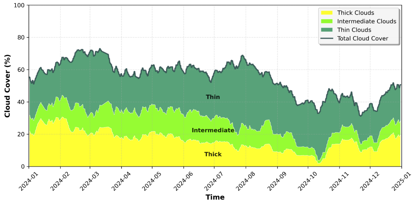
400 Figure 7: Cloud cover 31-day running-mean time series for the SGP site as determined by ASISKYCOVER for 2024. The stacked colored areas represent the distribution of cloud types (see legend and labels).
