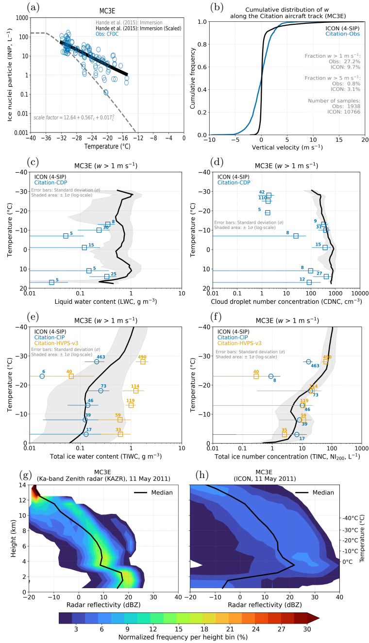
Figure 8. As in Fig. 6 but for MC3E case observed on 11 May 2011. In (a), INP observations (DeMott et al., 2015; Waman et al., 2022) are from the same month but a different year (2014). During MC3E, the LWC and CDNC were measured by the CDP probes mounted on the Citation aircraft. In (f), the black line represents mean NI_{200} from the control simulation and from both the CIP and HVPS-v3 probes. The radar observations are from the Ka-band zenith radar ( 97.485^{\circ} W, 36.605^{\circ} N) operational during MC3E.
