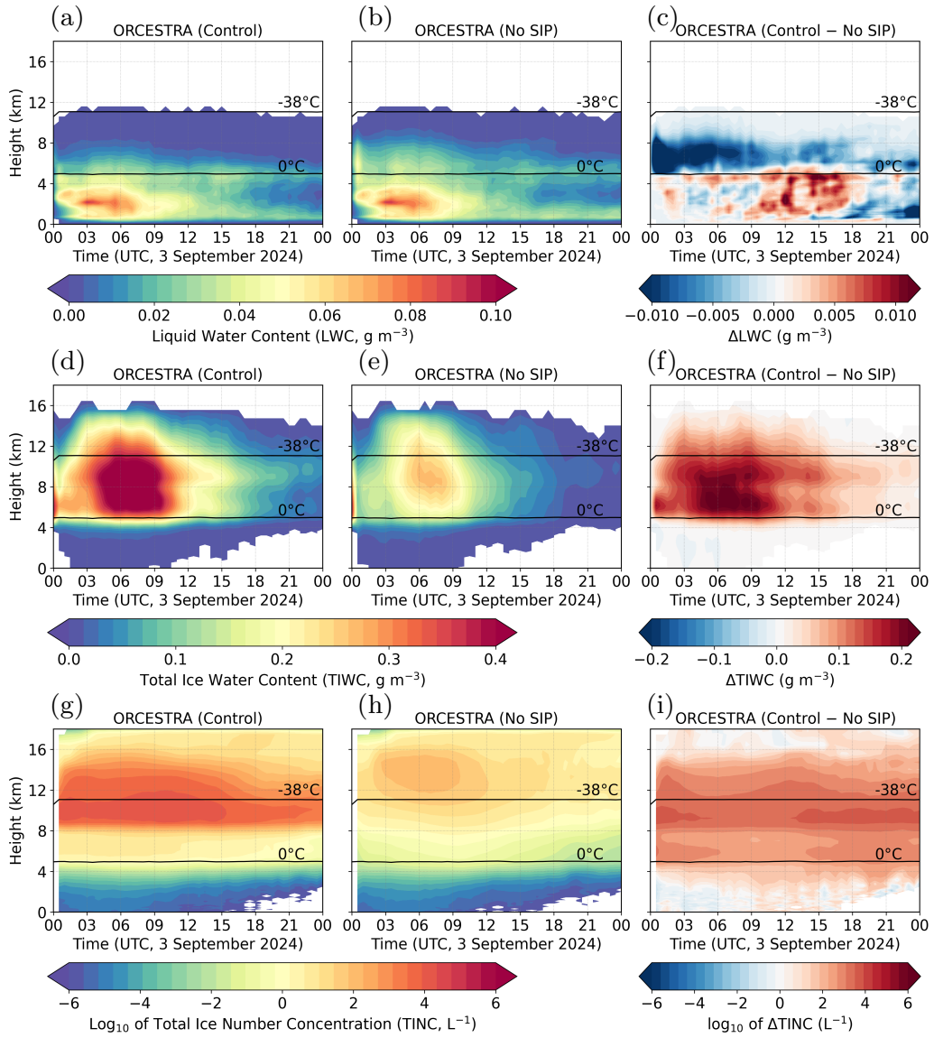
Figure 14. As in Fig. 11, but for ORCESTRRA convection.
