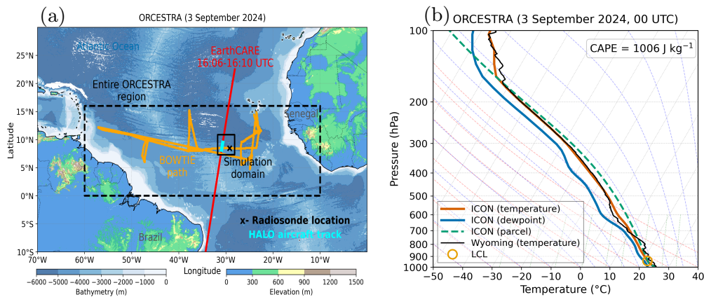
Figure 4. (a) Geographical location of the entire ORCESTR campaign (dashed black box). The yellow line in (a) shows the track of the research vessel RV Meteor during the BOWTIE campaign, the cyan line indicates the HALO aircraft track, and the red line shows the EarthCARE overpass over the selected ORCESTR region (solid black box), and ‘x’ shows the Radiosonde location on 3 September 2024. Also shown are the vertical profiles of (b) the simulated (red line) and observed (black line, Wyoming Sonde archive [8.47° N, 29.206° W]) air and simulated dew point temperature (blue line) at 00 UTC on 03 September 2024. In (b), the orange circle denotes LCL, and the simulated temperature profiles are from the control (Table 3) run of the ORCESTR case.
