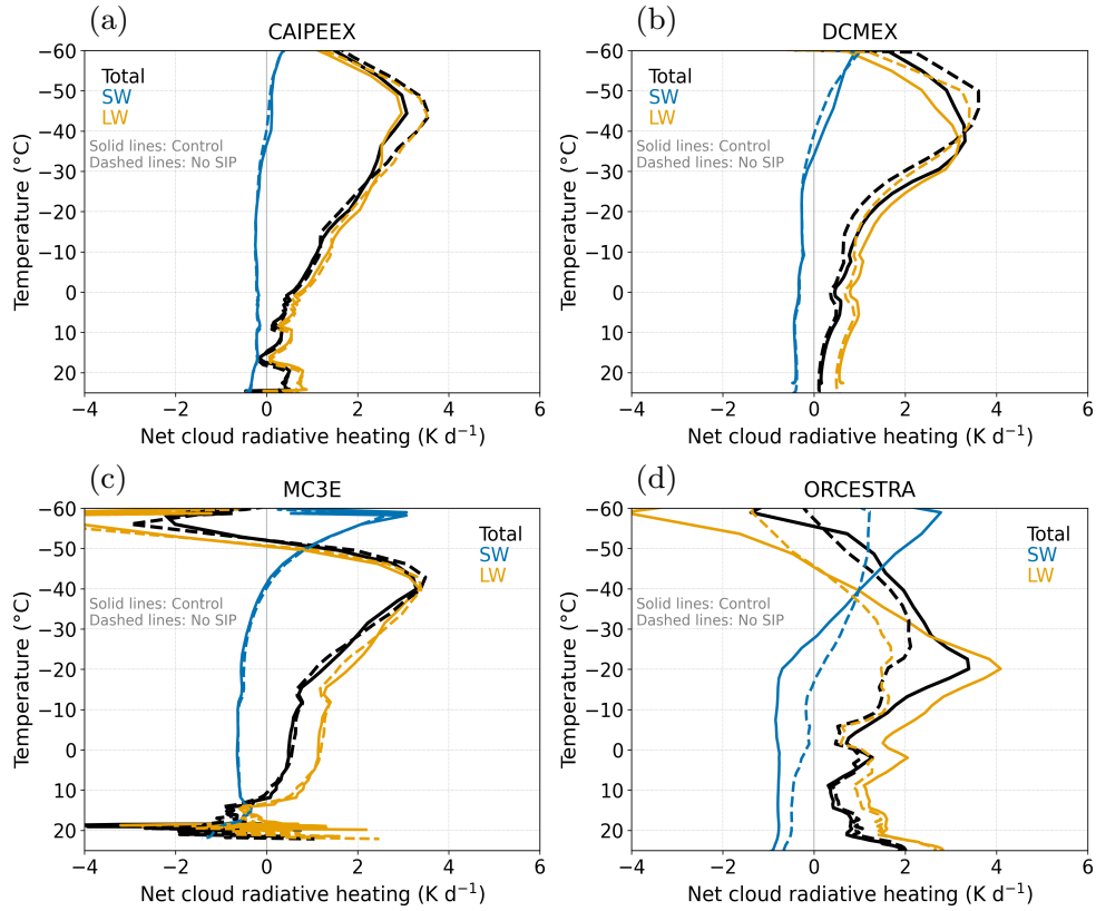
Figure 17. Simulated domain-averaged net cloud radiative heating (CRH, K d -1 , black lines) from the control (solid lines) and No SIP (dashed lines) simulations of (a) CAIPEEX, (b) DCMEX, (c) MC3E, and (d) ORCESTR clouds. Also shown are the SW (blue lines) and LW (yellow lines) components of CRH.
