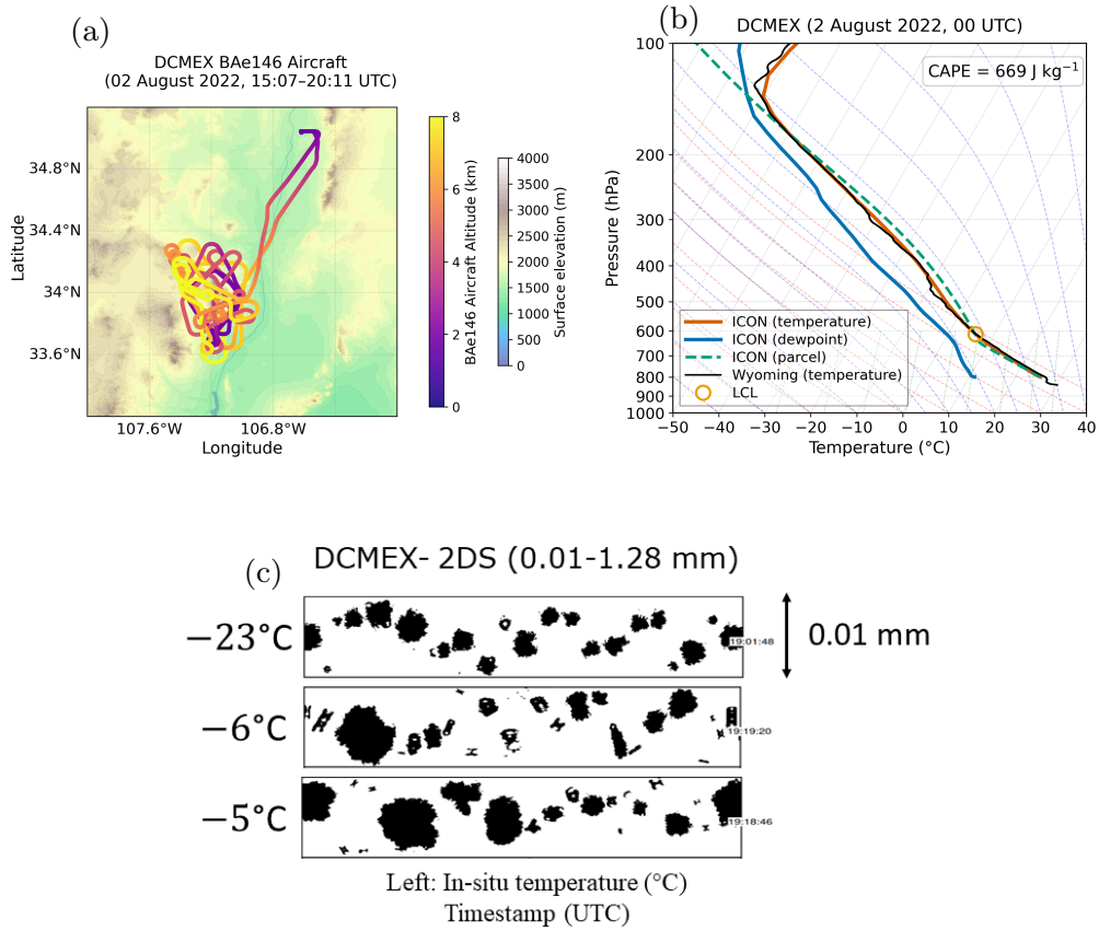
Figure 2. As in Fig. 1, but in (a) the flight path is for the BAE146 aircraft. In (b), observed air temperature (black line) is from the University of Wyoming archive [35.038° N, 106.623° W] at 00 UTC on 02 August 2022. The particle habits in (c) are from 2DS probe mounted on the BAE146 aircraft.
