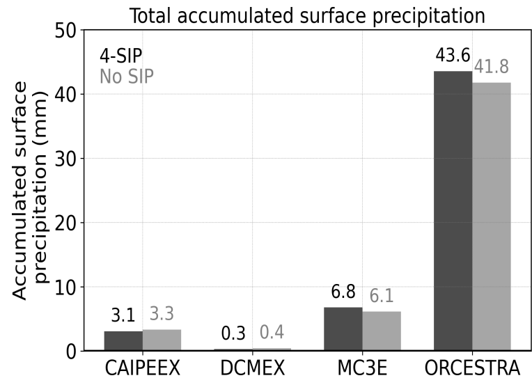
Figure 15. Total accumulated surface precipitation from the control (black bars) and No SIP (gray bars) simulations of CAIPEEX, DCMEX, MC3E, and ORCESTRA clouds.
