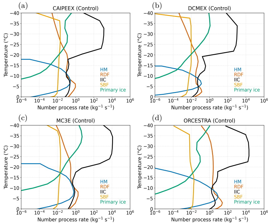
Figure 10. Profiles of the number process rates of various SIP processes, such as fragmentation in raindrop freezing (RDF, brown lines), Hallett-Mossop rime-splintering (HM, blue lines), ice-ice collision (IIC, black lines), and sublimation (SBF, yellow lines), averaged cloudy grid points for the control simulations of the DCCs, such as (a) CAIPEEX, (b) DCMEX, (c) MC3E, and (d) ORCESTRA. Also shown is the process rate for heterogeneously nucleated ice (Primary ice, green lines). Process rates represent time-integrated values over the simulation period.
