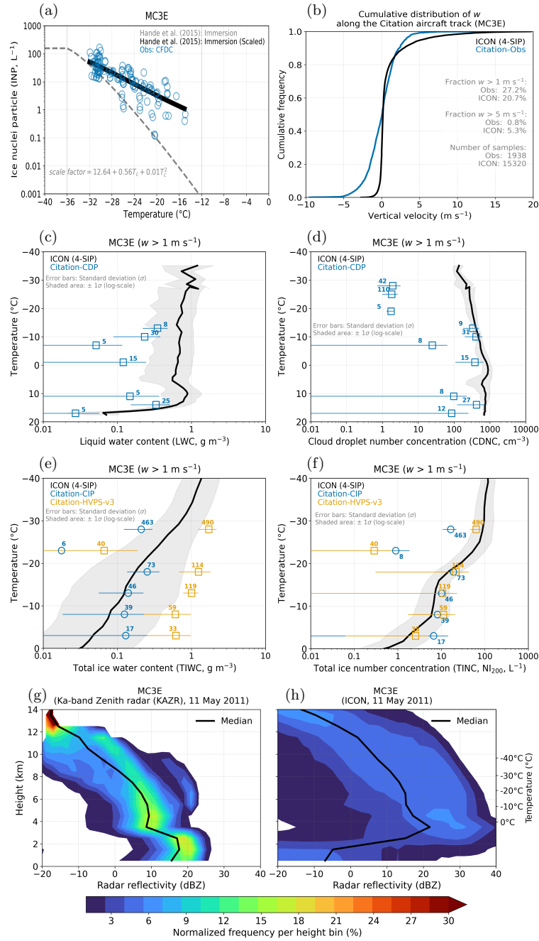
Figure 8. As in Fig. 6 but for MC3E case observed on 11 May 2011. In (a) INP observations (DeMott et al., 2015; Waman et al., 2022) are from the same month but different year (2014). During MC3E, the LWC and CDNC were measured by the CDP probes mounted on the Citation aircraft. In (f), the black line represents mean NI_{200} from the control simulation and from both the CIP and HVPS-v3 probes. The radar observations are from the Ka-band zenith radar ( 97.485^{\circ} W, 36.605^{\circ} N) operational during MC3E.
