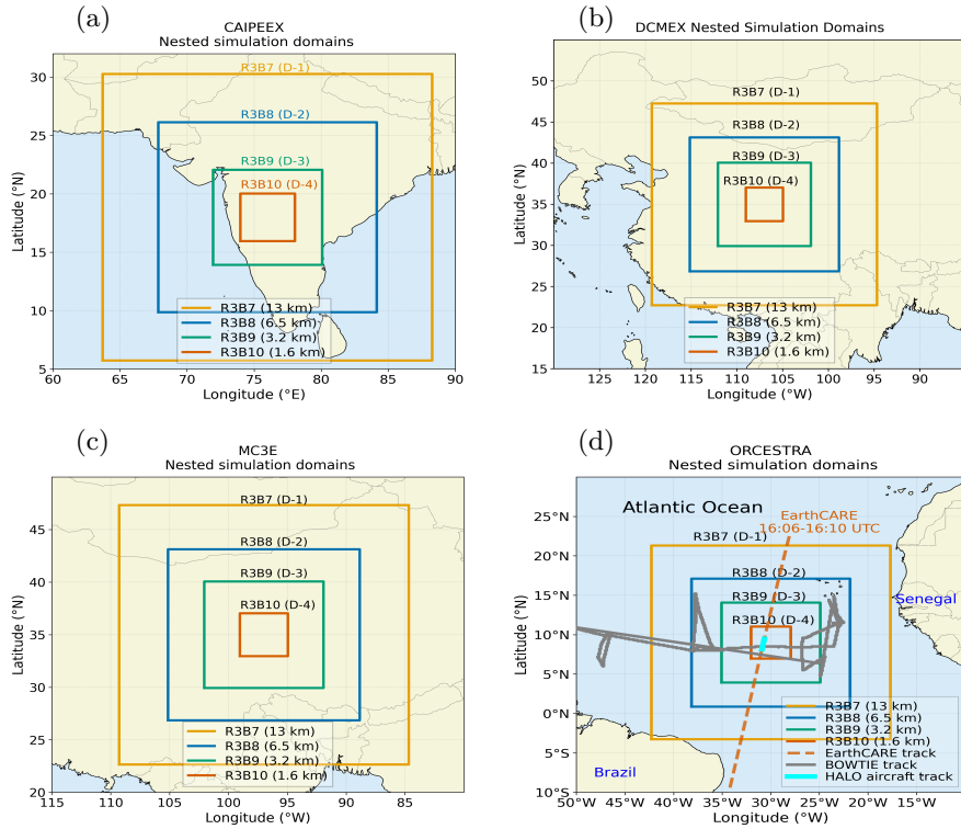
Figure 5. Outlines of the geographical areas used as domains for the simulated events of convection during (a) CAIPEEX, (b) DCMEX, (c) MC3E, and (d) ORCESTRA. The dashed red and thick cyan lines in (d) show the EarthCARE overpass and HALO aircraft track over the study location between 1606 and 1610 UTC on 3 September 2024.
