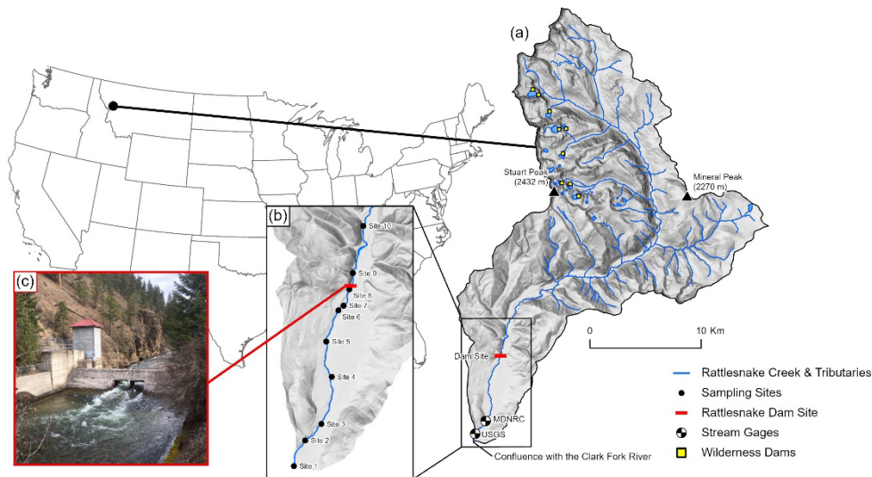
Figure 1: Location of the Rattlesnake Creek watershed (a) in Montana, United States, with the locations of the nine upstream wilderness dams (yellow squares). Stream Team monitoring site locations are indicated along with the Rattlesnake Dam site (red bar) and the Montana Department of Natural Resources and Conservation (MDNRC) stream gage and decommissioned USGS stream gage. Downstream sites 1–8 are the impact sites (b), upstream sites 9 and 10 are the reference sites (b). A photo of the dam (c) before removal and after permanent opening of the sluice gates is shown (from TU). A timeline of the Rattlesnake dam (d) highlights main events from the construction to removal of the dam.
