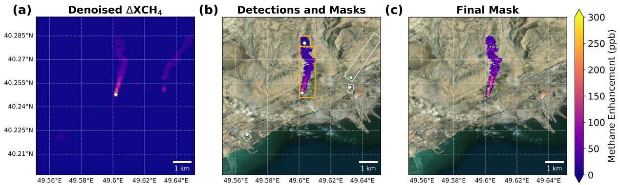
Figure 5. Plume mask creation process for one-of-the plumes-western plume from Fig. 3a. (a) The denoised Methane-methane enhancement ( \Delta XCH_4 ) field obtained by applying the Chambolle total variance-denoising-variation (TV) denoising filter to \Delta XCH_4 within the 1300~2500 nm window. The white star is-marks the manually identified source location for the western plume. (b) The-initial-plume-Initial candidate masks derived from the watershed algorithm for-the-western-plume . White dots indicate high- \Delta XCH_4 locations, while-and-colored rectangles represent the minimum rotated rectangles ( oriented bounding boxes ) for each mask. Orange rectangles denote masks with azimuth differences less than 30^\circ -relative to the reference mask (containing the source marker of the western source) and are merged into a single plume . The gray rectangles correspond-to-other-potential-plumes are candidates excluded by the azimuth criterion. (c) The final \Delta XCH_4 plume mask for the western emission source after merging . Background imagery source: Esri | Powered by Esri.
