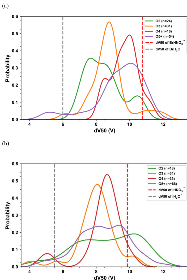
Figure 5. Probability density distributions of dV_{50} for compounds C_xH_yO_z ( z \geq 2 ) detected in the (a) bromide channel and (b) iodide channel of MR-CIMS. dV_{50} of water and nitric acid in each channel are shown for comparison. The number of compounds in each category are shown in the label.
