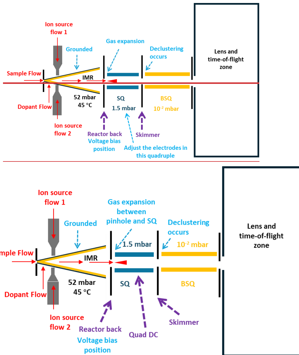
Figure 1. Schematic of the MR-CIMS structure. Gas flow paths are indicated in red, and key the electrodes/voltages adjusted during voltage scanning are highlighted by purple dashed arrows and texts. Explanatory annotations are denoted by blue dashed arrows and words. Pressures of the IMR, SQ (short quadrupole), and BSQ (big-segmented quadrupole), as well as the temperature of the IMR, are labeled to facilitate understanding of the operating conditions in MR-CIMS.
