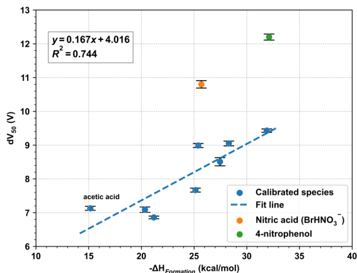
Figure 3. Comparison between the cluster formation enthalpy calculated at the DLPNO-CCSD(T)/def2-QZVPPD level at 298.15 K and experimentally determined \text{dV}_{50} . The error of \text{dV}_{50} represents the standard error of the sigmoid fit. Nitric acid was an obvious outlier due to the stabilization effects of water clusters. 4-nitrophenol was clustered at the collision limit, causing its \text{dV}_{50} to deviate substantially from the fitted trend of the other data points.
