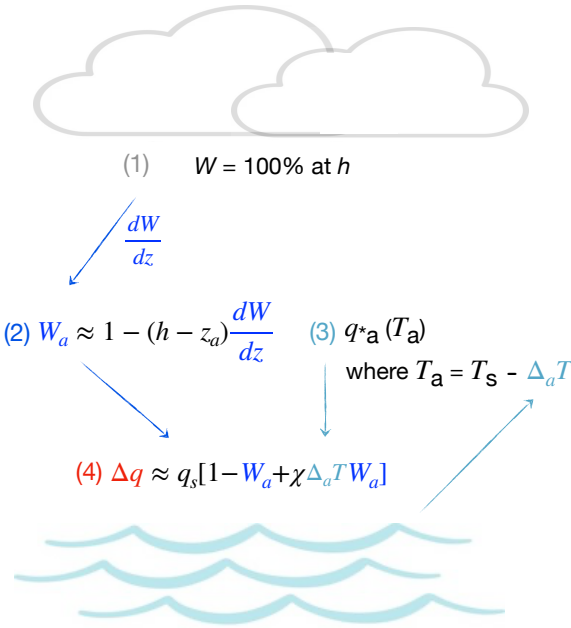
Figure 2. Schematic overview of the methodology highlighting the three main error sources: (1) estimating cloud base height, h , where W=100\% W=100\% is assumed and then extrapolated to z_a using (2) a fixed relative humidity lapse rate \frac{dW}{dz} , which is then converted to q_a as described in the text with (3) a fixed \Delta_a T = 1.3 K.
