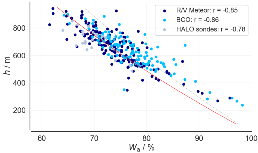
Figure 4. Near-surface relative humidity at 40 m, W_a , from radiosondes and ceilometer-based estimates of cloud base height, h (using the first, major peak of the distribution), from R/V Meteor ( n=171 , dark blue) and BCO ( n=118 , medium blue) measurements. Also shown are area-averaged estimates of h from HALO dropsondes (light blue) as calculated by Vogel et al. (2022) and Albright et al. (2022). Lines are theoretical relationships, as described in the text (red: adiabatic lapse rate of -9.8 K/km; light grey dashed line: temperature lapse rate of -8.5 K/km).
