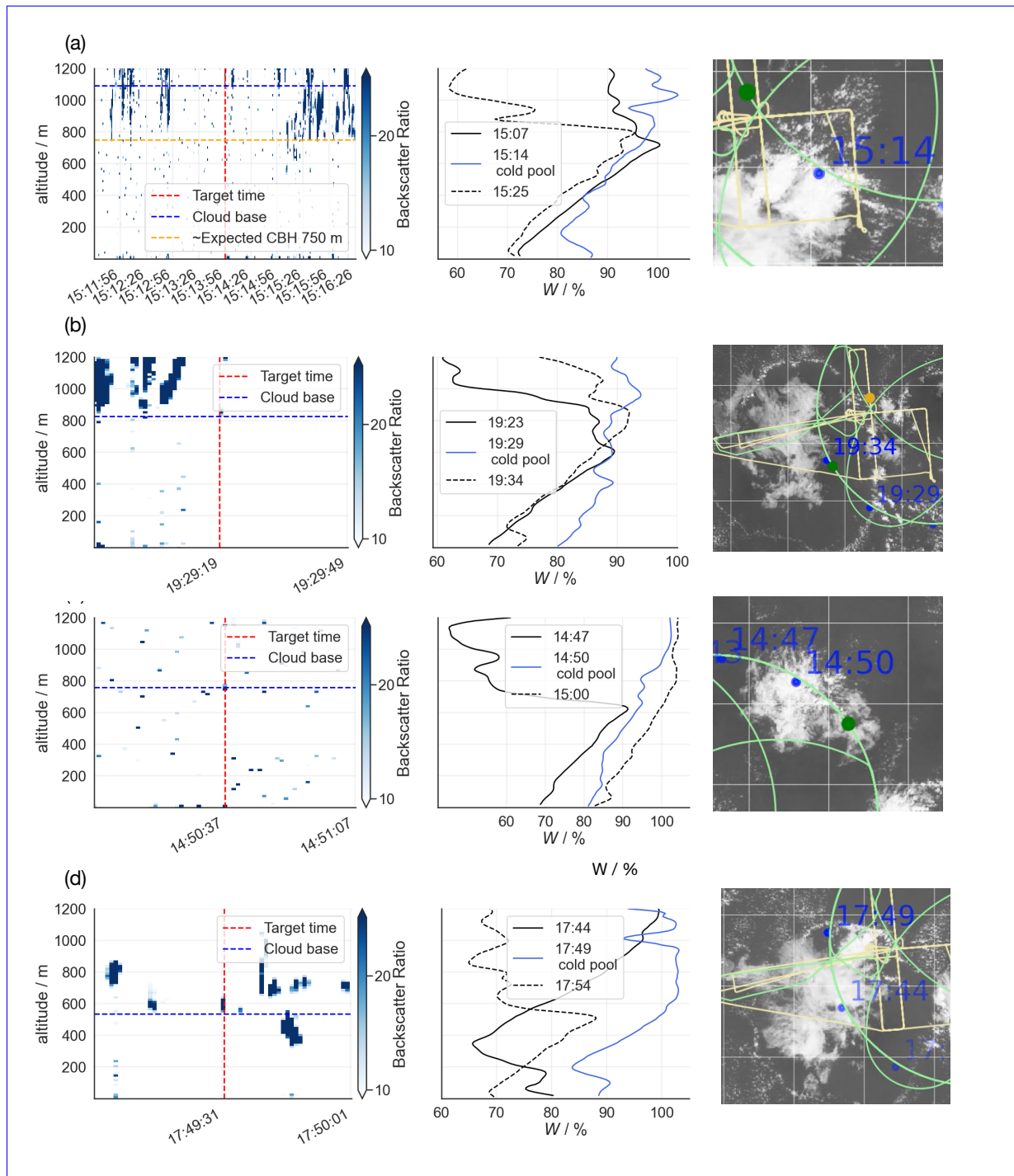
Figure 6. The four Four anomalous W_a and h pairings labeled as outliers, (a), (b), (c), and (d), in from Fig. 5. Left column Shown for the four outlier points are: (left column) the backscatter ratio including the selected time as vertical line (red), the inferred cloud base height (blue horizontal line), and for the top panel, an approximate cloud base height value expected from the linear relationship (orange horizontal line); (center column) relative humidity profiles for the nearest sounding in blue, as well as the soundings immediately before and after (black, solid and dashed, respectively); (right column) visible satellite images (GOES-16 ABI) illustrating showing the cloud organization structure from above and the location of the dropsonde at its launch time, accessed via https://observations.ipsl.fr/aeris/eurec4a-data/PRODUCTS/GOES-E_movies/VIS_IR_combined/v1.0.0/ .
