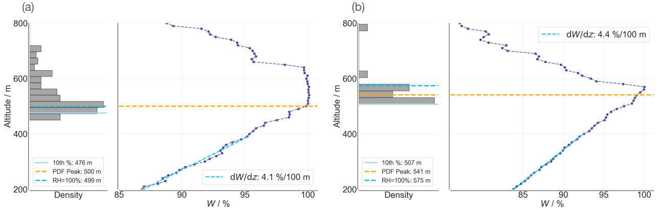
Figure 3. Ceilometer-First ceilometer cloud returns for 30 minutes before and after the radiosonde launch time (grey histograms) and the relative humidity profiles measured by the radiosondes (blue profiles, data every 10 m). Also shown on the ceilometer cloud base height histograms are the 10th percentile (solid light blue line), the first major peak of the distribution calculated from a Gaussian kernel density estimate (orange dashed line), and the height at which relative humidity would reach 100% when extrapolating from a linear regression fit to the observed profile from 200–400 m (turquoise dashed line), as described in the text. Panel (a) is around the radiosonde launched on Jan. 29, 2020 at 06:44 UTC (2:44 am local Barbados time) and panel (b) is Feb. 1 2020 at 00:25 UTC (8:25 pm local Barbados time). These are two cases where radiosonde relative humidity reached 100% below 1000 m.
