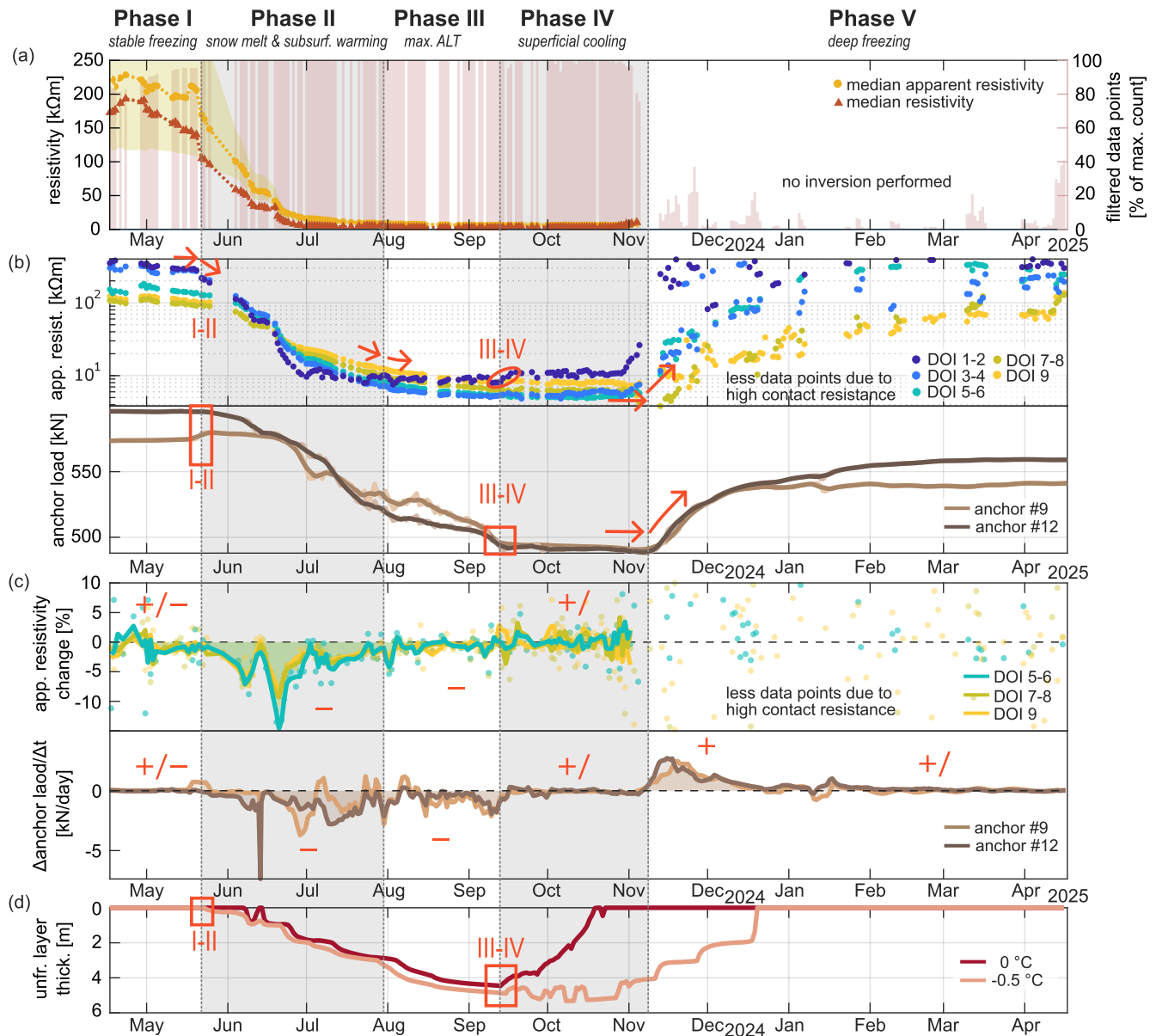
Figure 5. a) Median apparent resistivity with interquartile range (yellow shading). Salmon bars indicate the percentage of available data points (n=135) after filtering. b) Median apparent resistivity for specific depths of investigation (DOI) and raw as well as one-week-smoothed anchor load variations. c) Relative changes in median apparent resistivity from deep-reaching ERT signals (DOI5–9), smoothed over one week, and the rate of change (first derivative) of anchor loads. d) Evolution of the unfrozen layer thickness based on the 0^\circ\text{C} and -0.5^\circ\text{C} isotherms. Red rectangles and arrows indicate the shifts in the parameter's pattern between the seasonal phases.
