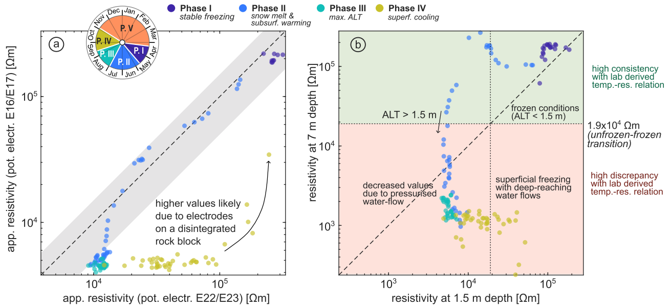
Figure 6. (a) Influence of small-scale rock heterogeneity on apparent resistivity, illustrated by a log–log plot comparing quadrupole measurements using potential electrodes E22/E23 (positioned on a disintegrated rock block) with E16/E17 (located at the profile centre). The grey band indicates a \pm 50\% deviation from the 1:1 line. (b) Median resistivity values at depths representative of permafrost conditions (7 m) and seasonally unfrozen conditions (1.5 m). The timing at which the active layer depth exceeds 1.5 m is marked. The transition between the unfrozen and frozen conditions at \sim 19 \text{ k}\Omega\text{m} is derived from laboratory experiments, see Offer et al. (2025) and Figure 5.
