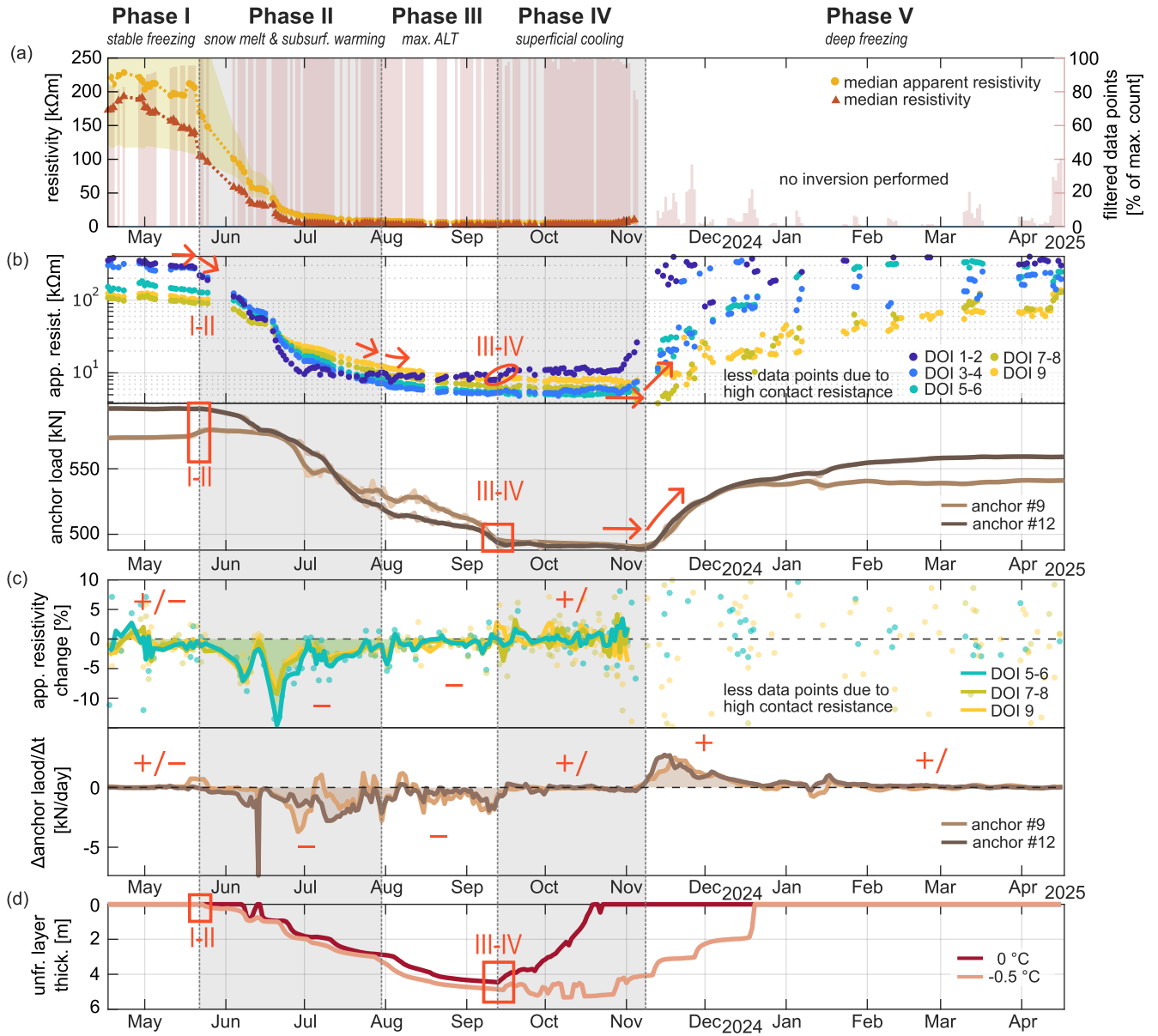
Figure 4. a) Median apparent resistivity with interquartile range (yellow shading). Salmon bars indicate the percentage of available data points (n=135) after filtering. b) Median apparent resistivity for specific depths of investigation (DOI) and raw as well as one-week-smoothed anchor load variations. c) Relative changes in median apparent resistivity from deep-reaching ERT signals (DOI5-9), smoothed over one week, and the rate of change (first derivative) of anchor loads. d) Evolution of the unfrozen layer thickness based on the 0°C and -0.5°C isotherms. Red rectangles and arrows indicate the shifts in the parameter's pattern between the seasonal phases.
