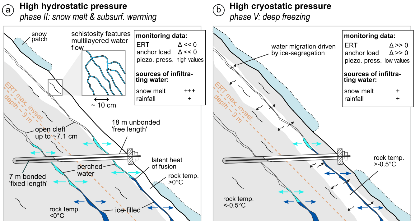
Figure 7. Schematic illustration of seasonal phases associated with high a) hydrostatic and b) cryostatic pressures that might predispose permafrost rockwalls to instability: a) During snowmelt and subsurface warming (phase II), high hydrostatic pressure can develop above sealed fractures, leading to mechanically widening of fractures. b) During deep freezing in winter (phase V), ice formation within discontinuities promotes ice segregation and associated cryostatic pressure build-up, resulting in stress redistribution within the rock mass.
