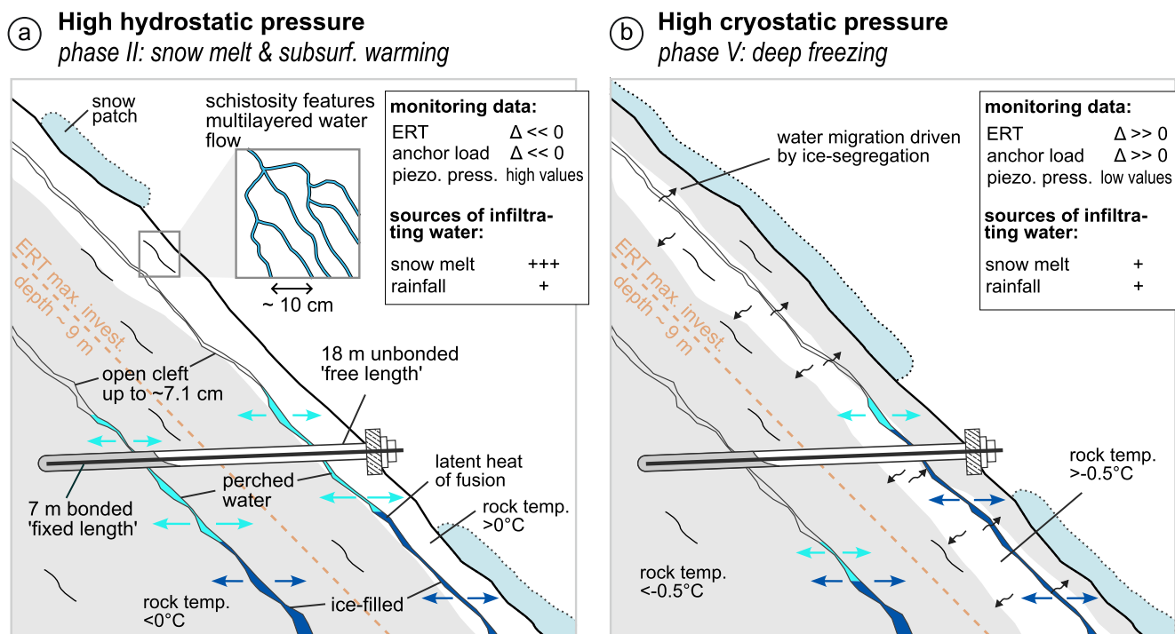
Figure 8. Schematic illustration of seasonal phases associated with high a) hydrostatic and b) cryostatic pressures that might predispose permafrost rockwalls to instability: a) During snowmelt and subsurface warming (phase II), high hydrostatic pressure can develop above sealed fractures, leading to mechanically widening of fractures. b) During deep freezing in winter (phase V), ice formation within discontinuities promotes ice segregation and associated cryostatic pressure build-up, resulting in stress redistribution within the rock mass.
