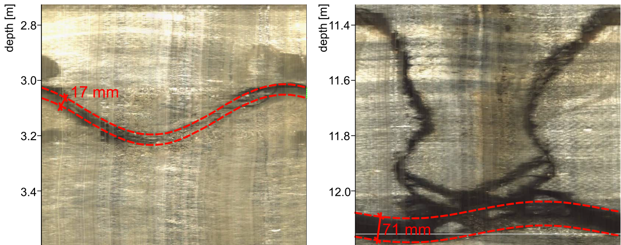
Figure A2. The high degree of fracturing of the rockwall is shown by an optical scan of a vertical drilled borehole located within < 2 m of electrode 1 ( x = 0 m). The upper meters of the borehole scan revealed open discontinuities with apertures of 17 and 71 mm, providing effective pathways for water infiltration or ice formation.
