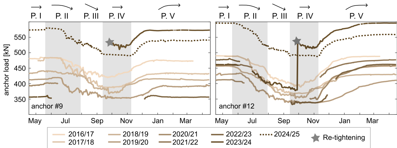
Figure A3. Seasonal patterns in anchor loads since the start of monitoring in 2016. High loads during phase I (stable freezing) are followed by a progressive decrease through phases II (snow melt and subsurface warming) and III (maximum active layer thickness), with minimum values typically observed in late summer in phase IV (superficial cooling). Loads increase again during phase V (deep freezing). The period of automated ERT monitoring between April 2024 and April 2025 is highlighted by a dashed line. Anchor re-tightening events are indicated.
