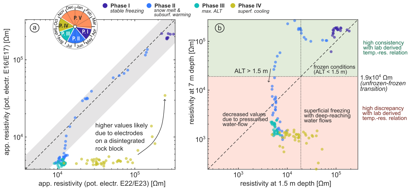
Figure 7. (a) Influence of small-scale rock heterogeneity on apparent resistivity, illustrated by a log–log plot comparing quadrupole measurements using potential electrodes E22/E23 (positioned on a disintegrated rock block) with E16/E17 (located at the profile centre). The grey band indicates a \pm 50\% deviation from the 1:1 line. (b) Median resistivity values at depths representative of permafrost conditions (7 m) and seasonally unfrozen conditions (1.5 m). The timing at which the active layer depth exceeds 1.5 m is marked. The transition between the unfrozen and frozen conditions at \sim 19\text{k}\Omega\text{m} is derived from laboratory experiments, see Offer et al. (2025) and Figure 6.
