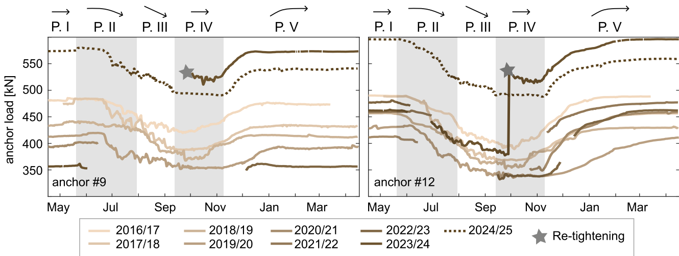
Figure 4. Seasonal patterns in anchor loads since the start of monitoring in 2016. High loads during phase I (stable freezing) are followed by a progressive decrease through phases II (snow melt and subsurface warming) and III (maximum active layer thickness), with minimum values typically observed in late summer in phase IV (superficial cooling). Loads increase again during phase V (deep freezing). The period of automated ERT monitoring between April 2024 and April 2025 is highlighted by a dashed line. Anchor re-tightening events are indicated.
