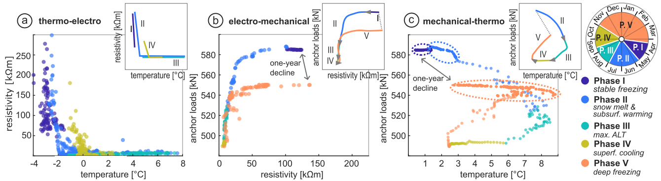
Figure A5. Electro-thermo-mechanical interaction of the rockwall with schematic representations for phases I–V: a) Temperature–resistivity relation along borehole B2 down to 5 m depth, (b) resistivity–load relation based on the median apparent resistivity (from DOI 9, corresponding to a maximum electrode spacing of 18 m) and the mean load of both anchors, (c) temperature–load relation, represented by the mean anchor load and the temperature range (minimum to maximum) measured along the perpendicular anchor length (0–13 m). Dashed-line circles indicate periods when temperatures were entirely below 0 °C, making cryosuction unlikely. The one-year decline in anchor load is marked accordingly.
