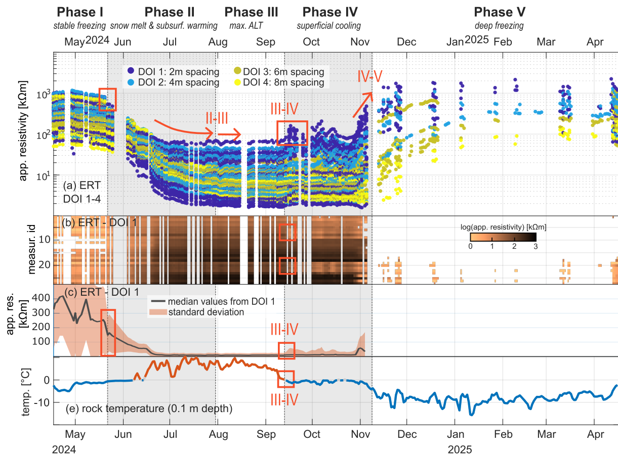
Figure A4. Apparent electrical resistivity and near-surface rock temperature: a) Apparent resistivity in the upper subsurface layer measured with electrode spacing between 2 to 8 m (DOI 1–4). b)+c) Apparent resistivity near the rock surface with 2 m electrode spacing. e) Rock temperature at 0.1 m depth in borehole B2, showing positive temperatures between early June and mid-September 2024. Red rectangles and arrows highlight shifts in parameter patterns corresponding to different seasonal phases.
