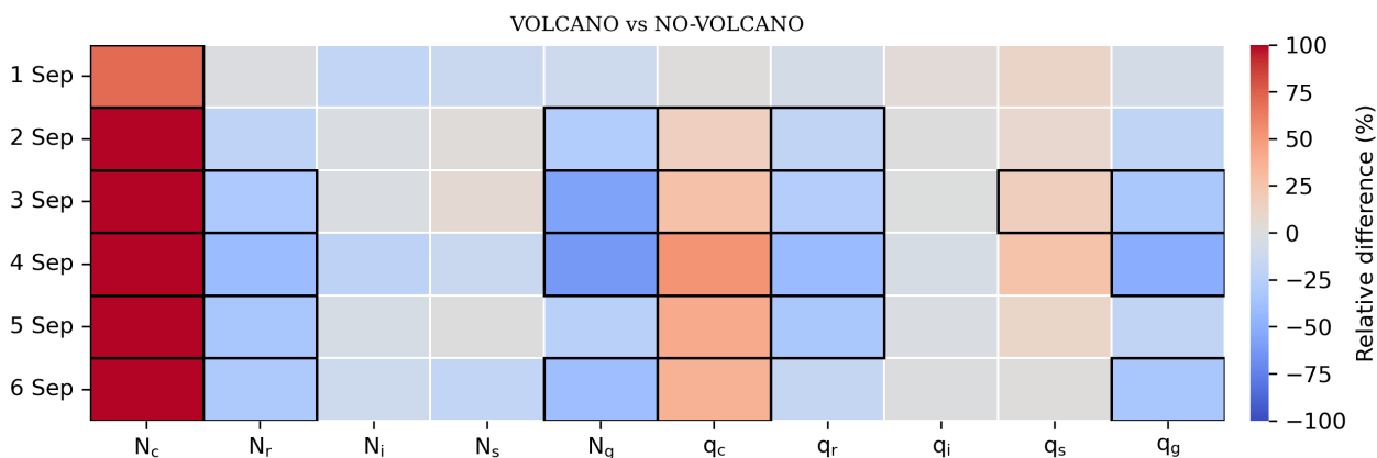
Figure 6. Statistical-Relative differences (VOLCANO minus NO-VOLCANO divided by NO-VOLCANO) and statistical significance of daily changes in-between the VOLCANO and NO-VOLCANO simulations for Holuhraun inside the plume. The color bar shows Colors indicate the p-value. Dark blue relative difference, while black boxes denote statistically significant differences ( p < 0.05 ) shows a statistically significant change in cloud hydrometeors in the VOLCANO and NO-VOLCANO simulations inside the plume on the for each day indicated by (y-axis).
