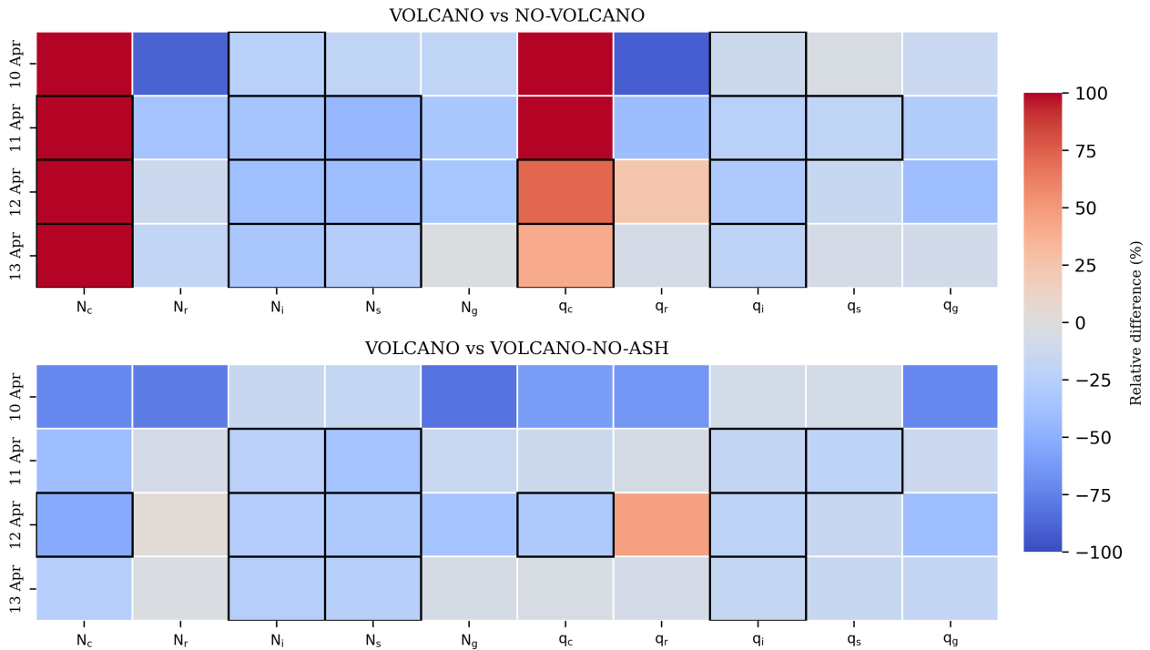
Figure 13. Statistical Relative difference and statistical significance of daily changes in VOLCANO and NO-VOLCANO simulations (top) and VOLCANO and VOLCANO-NO-ASH simulations for La Soufrière inside the plume. The color bar shows Colors indicate the p-value. Dark blue shows a relative difference, while black boxes denote statistically significant change differences ( p < 0.05 ) in cloud hydrometeors in these simulations inside the plume on the for each day indicated by (y-axis).
