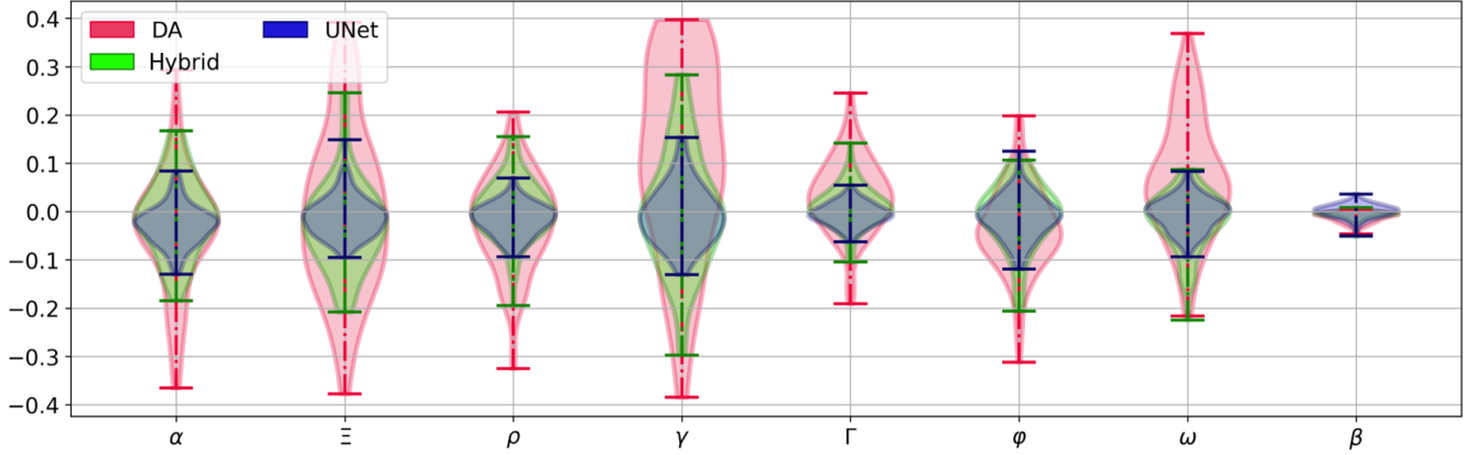
Figure E1. Evaluation metrics of the calibration of the BGC model. We assess a 4Dvar scheme (red distribution), a learning-based scheme (blue distribution) and a hybrid scheme (green distribution). We consider the normalized parameter estimate error as detailed in Section 3.5.
